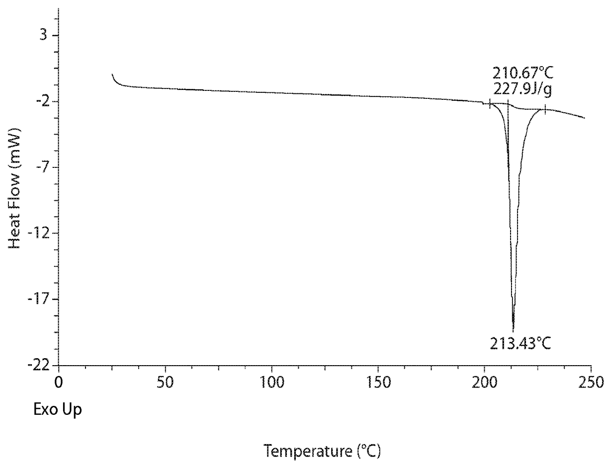
DSC profile of Form 3
