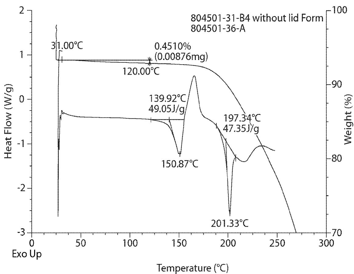
DSC and TGA profile of Form 10
