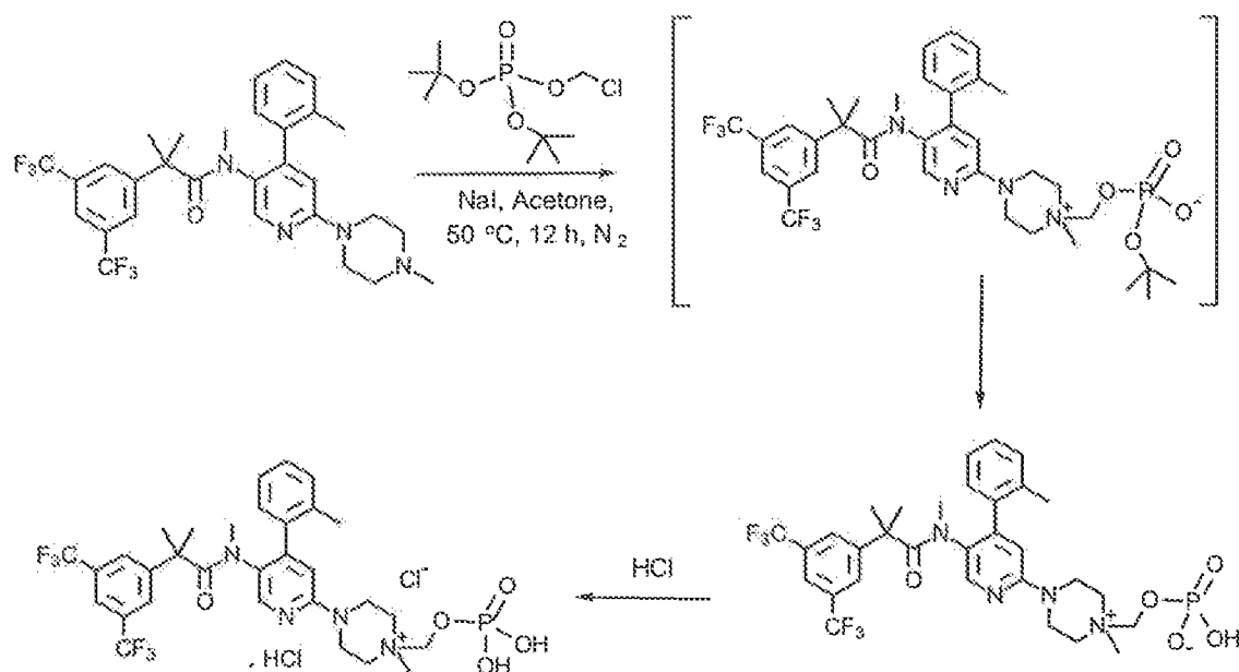
Scheme 6A
