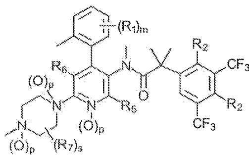
Formula (V)
