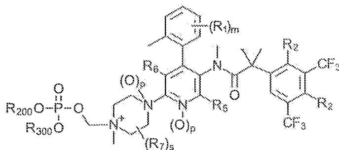
Formula (VI)
