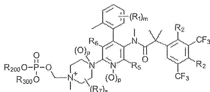
Formula (VI)
