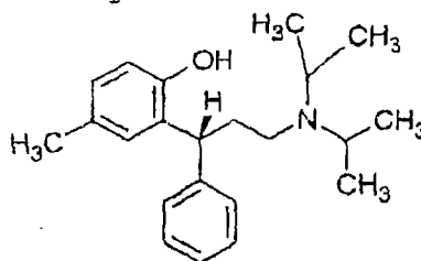
(R)-stereoisomer
