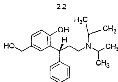
(R)-stereoisomer
