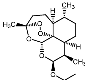
arteether ( 1d )
