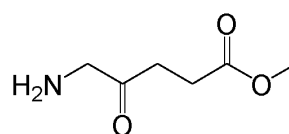
methyl-5-aminolevulinic acid (MAL)
