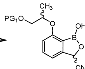
[Chemical Formula 8]
