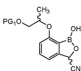
[Chemical Formula 8]
