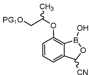
[Chemical Formula 9]
