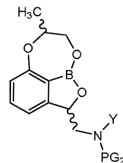
[Chemical Formula 11]
