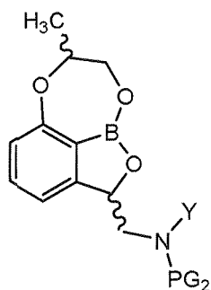
[Chemical Formula 1]
