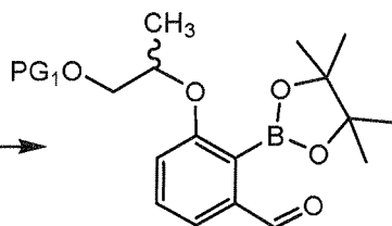
[Chemical Formula 7]
