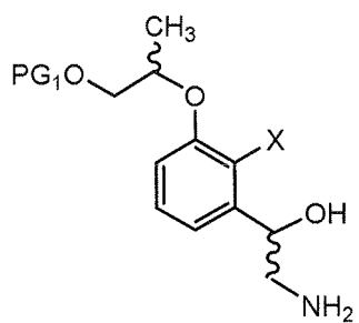
[Chemical Formula 14]
