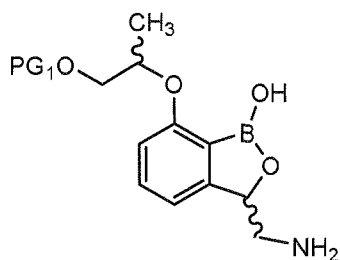
[Chemical Formula 10]
