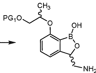
[Chemical Formula 9]
