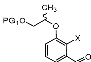
[Chemical Formula 6]
