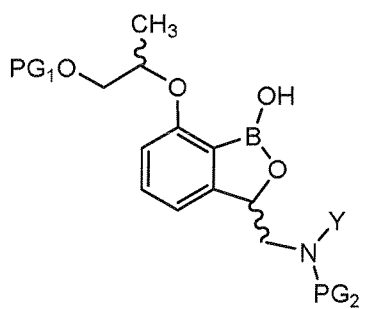
[Chemical Formula 11]
