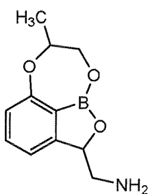
[Chemical Formula 1]
