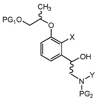
[Chemical Formula 10]
