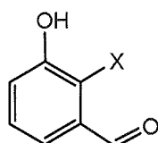
[Chemical Formula 6]
