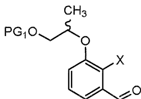
[Chemical Formula 7]
