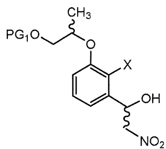
[Chemical Formula 13]
