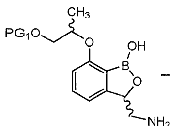
[Chemical Formula 9]
