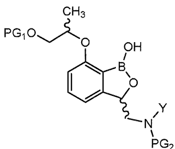
[Chemical Formula 11]
