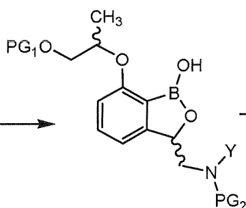
[Chemical Formula 10]
