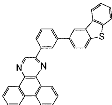
[Chemical Formula 10]
