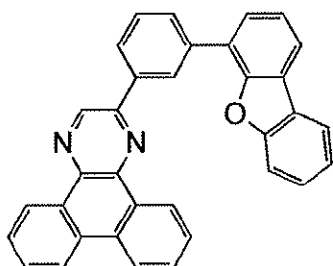
[Chemical Formula 9]
