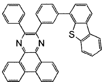
[Chemical Formula 8]
