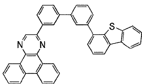
[Chemical Formula 6]
