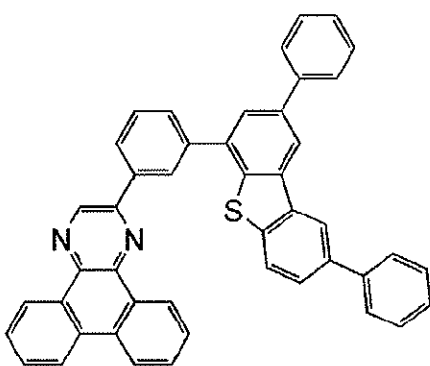
[Chemical Formula 7]
