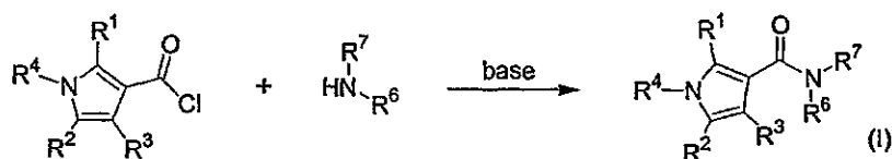
Scheme 1. General synthesis of compounds of formula (I).
