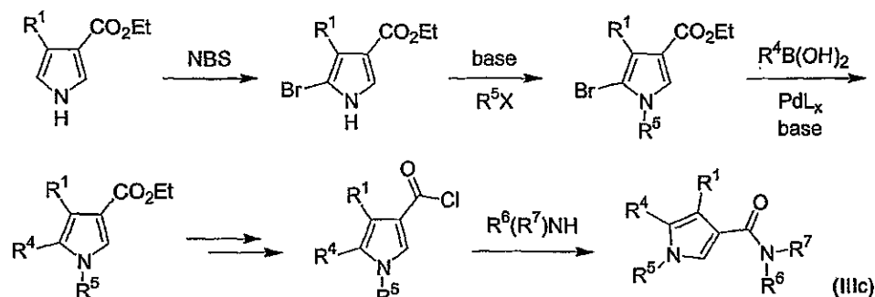
Scheme 10. Alternate preparation of pyrrole compounds (IIIc).
