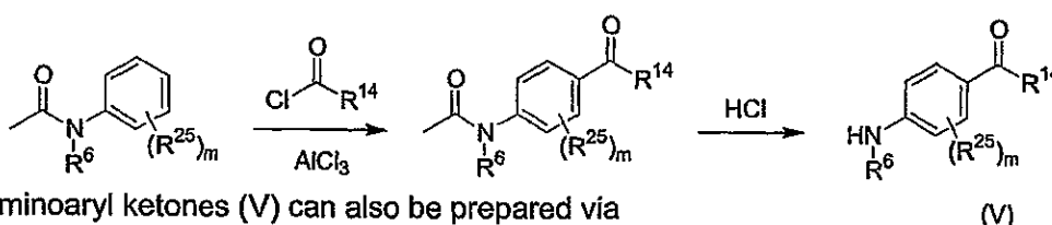
Scheme 16. Preparation of aminoaryl ketones (V).
