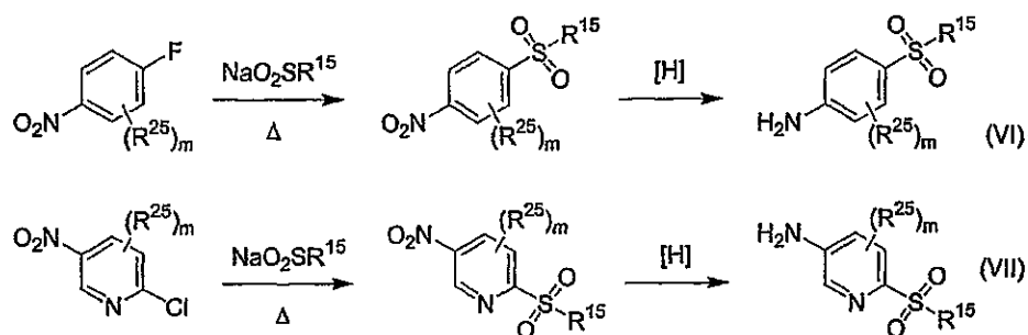
Scheme 18. Preparation of aminoaryl sulfones (VI) and pyridine analogues (VII).
