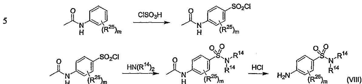
Scheme 23. Alternate synthesis of aminoaryl sulfonamides (VIII).
