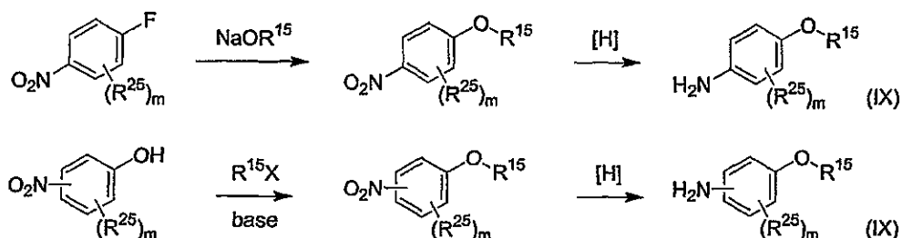
30 Scheme 24. Preparation of aminoaryl ethers (IX).
