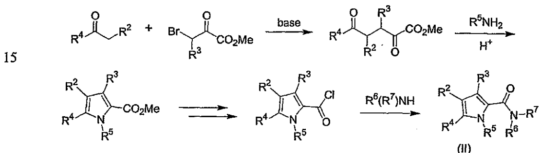
Scheme 7. Preparation of compounds of formula (II).
