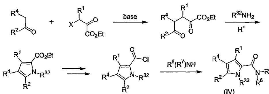
Scheme 14. Preparation of pyrrole compounds of formula (IV).
