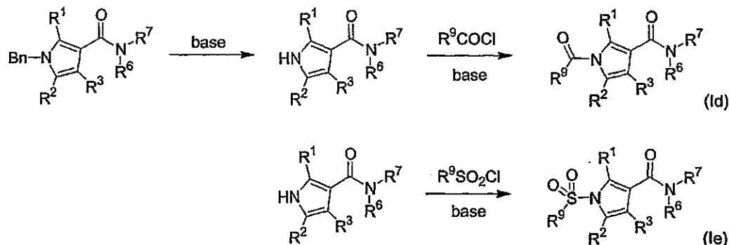
Scheme 26. Synthesis of compounds of formulae (Id) and (Ie).
