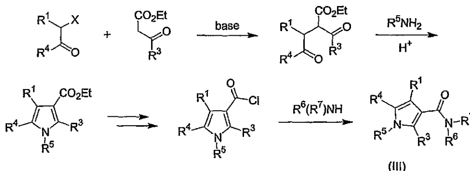
Scheme 8. General preparation of compounds of formula (III).
