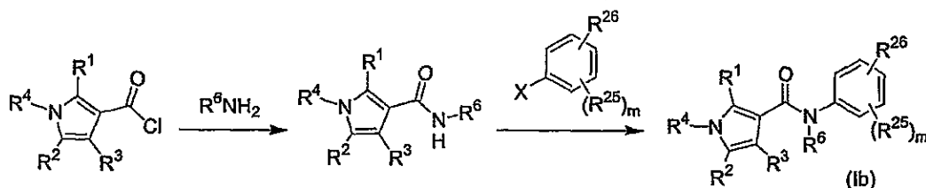
Scheme 2. Preparation of compounds of formula (Ib).
