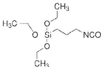
isocyanatopropyl-triethoxy-silane (ICN-TES)
