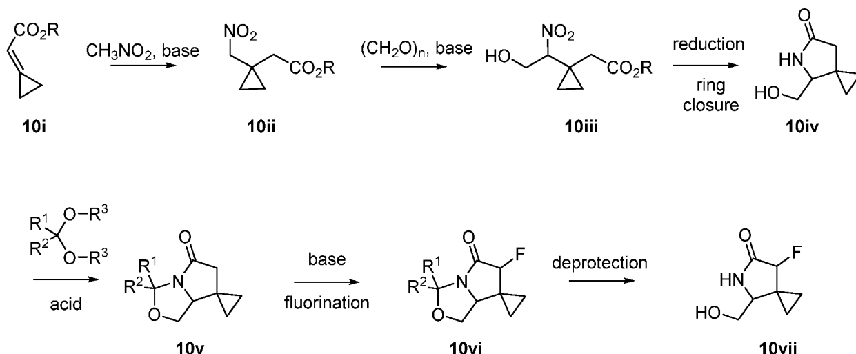
Scheme 10
