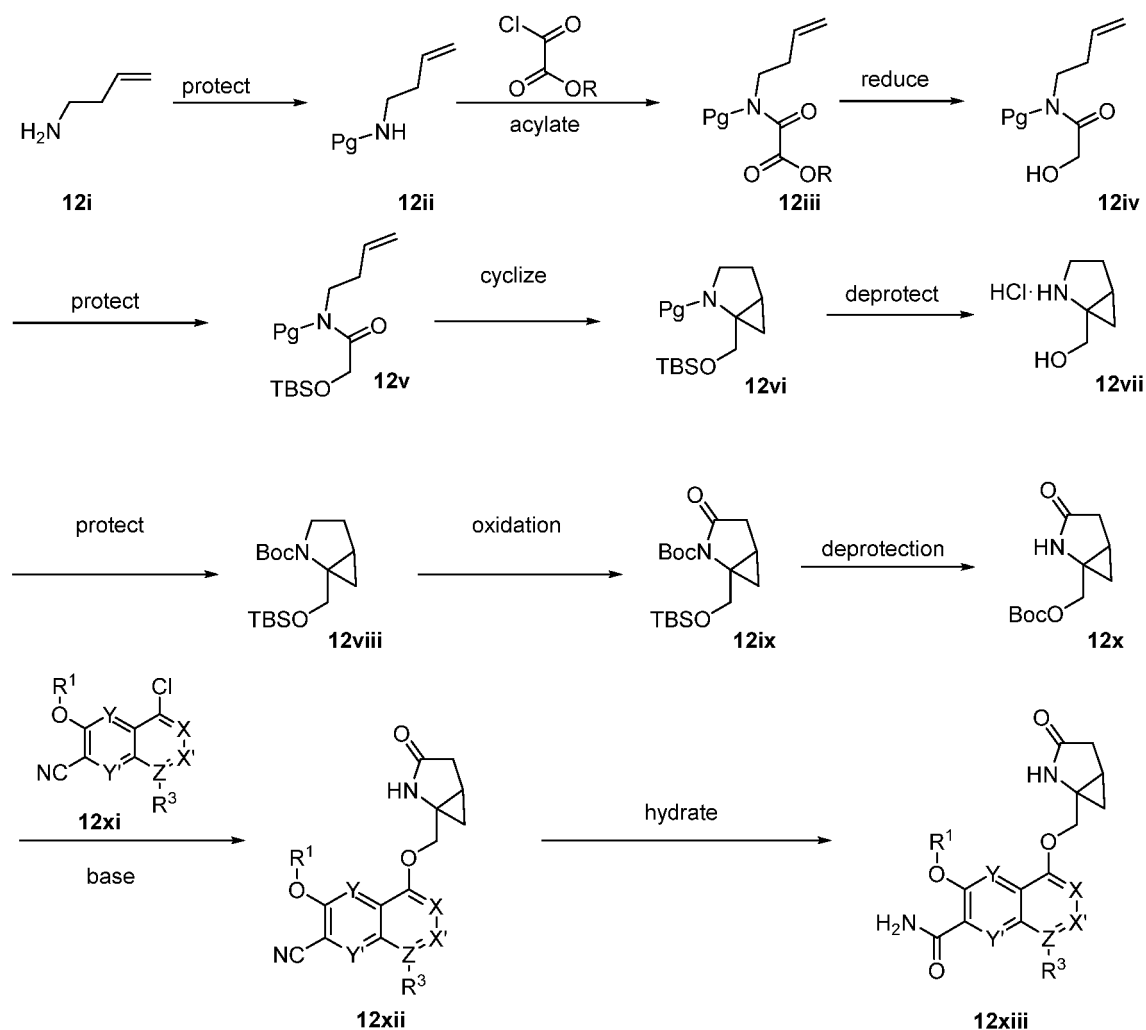
Scheme 12
