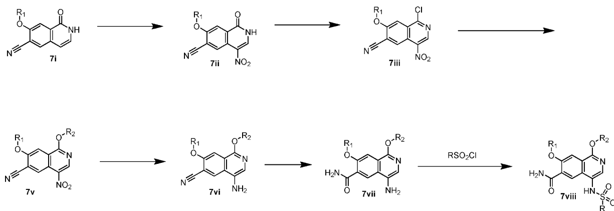
Scheme 7
