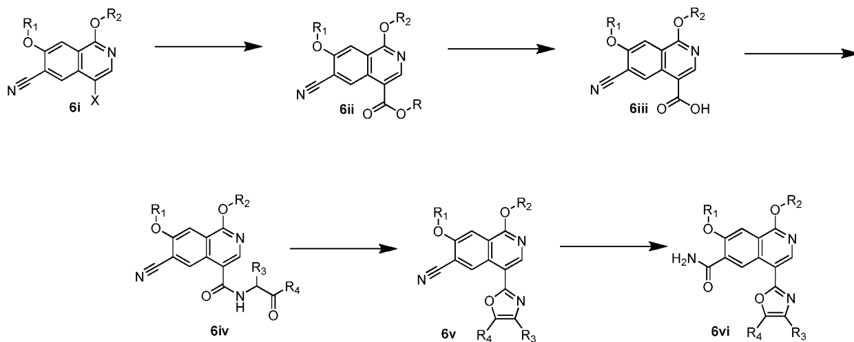
Scheme 6
