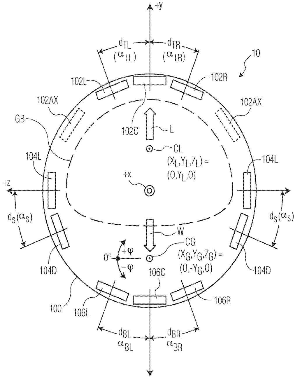
FIG. 3 ANTENNA PLACEMENT
