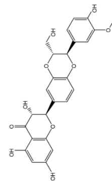
Isosilybin A
