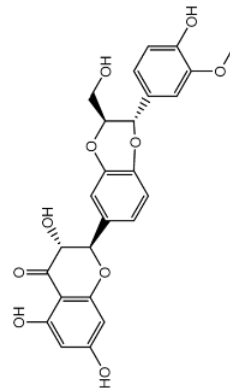
Isosilybin B
