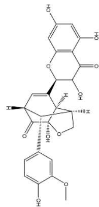
Silydianin
