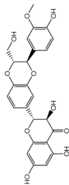
Silybin A
