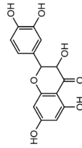
Dihydroquercetin
