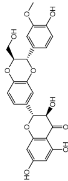
Silybin B
