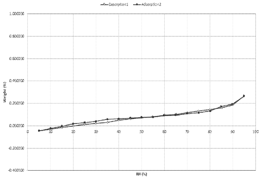
FIG. 4 Adsorption/Desorption Isotherm
