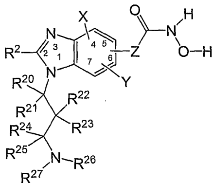
Formula (IIIb)
