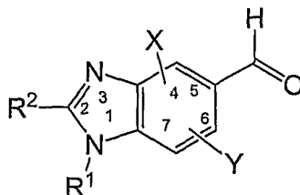
(B1)
