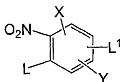
(C3)
