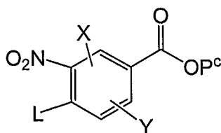
(B3)
