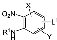
(C4)
