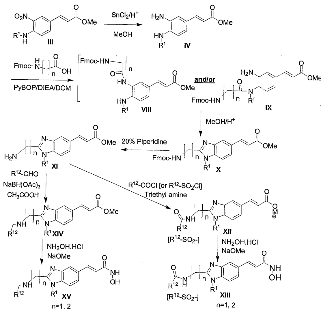
Scheme III
