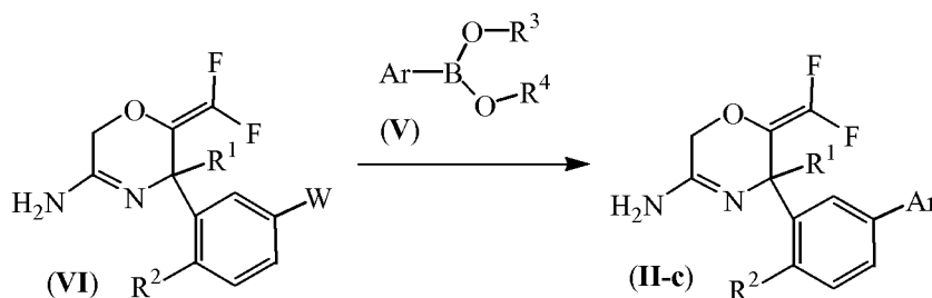
Reaction Scheme 3
