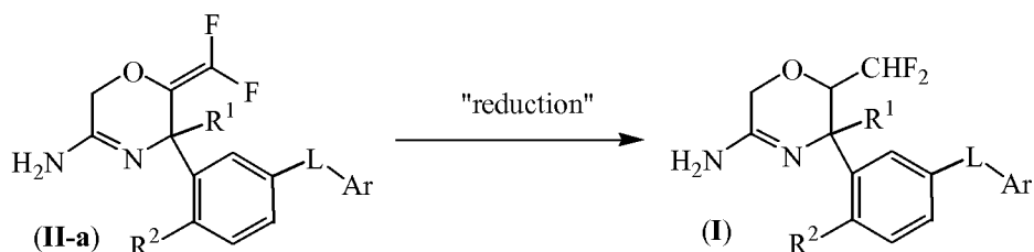
Reaction Scheme 1
