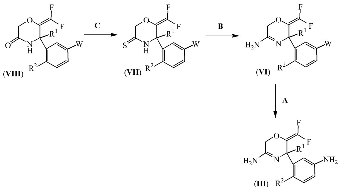
Reaction Scheme 4
