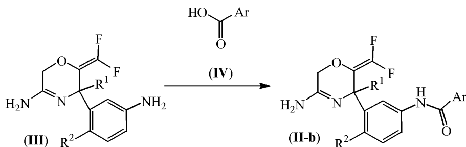
Reaction Scheme 2
