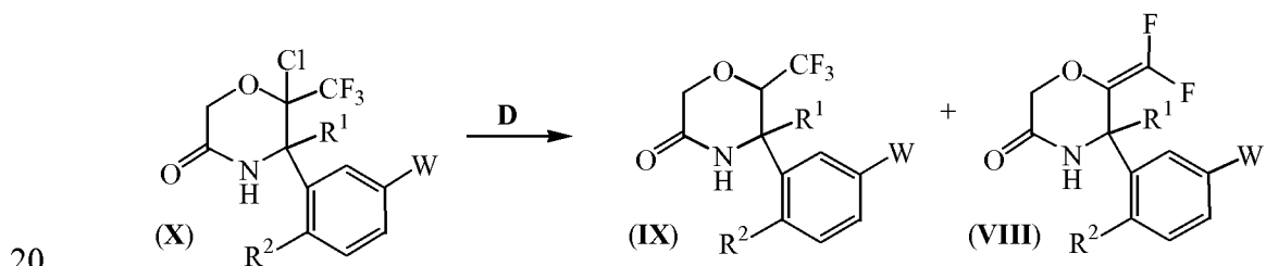
Reaction Scheme 5
