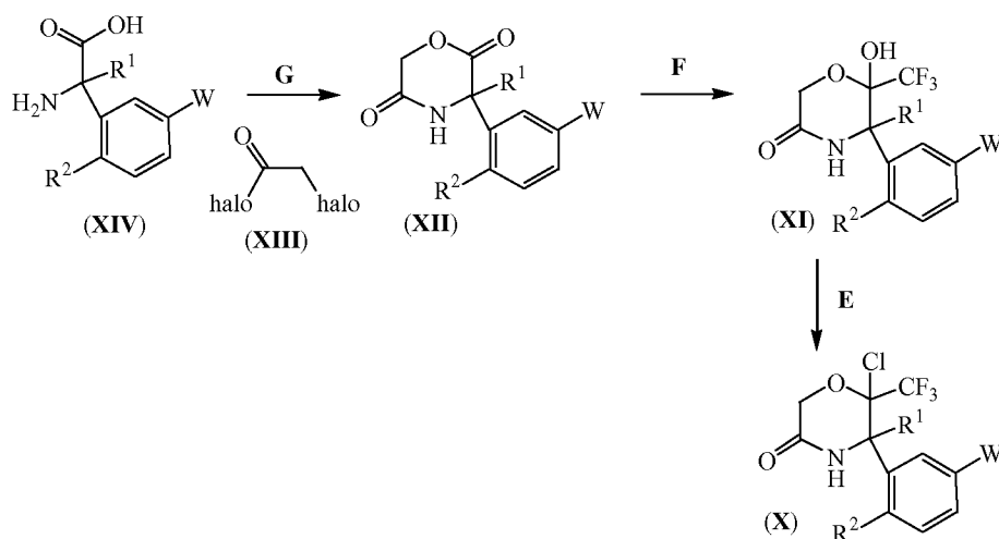
Reaction Scheme 6
