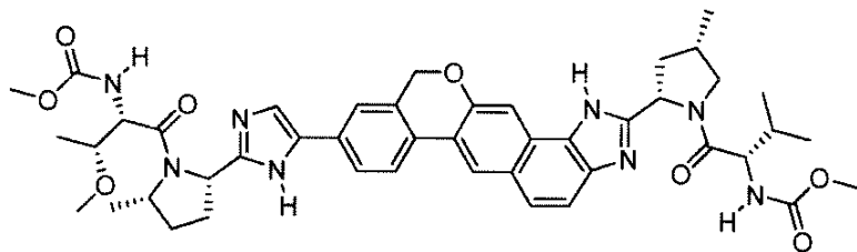
methyl [(2S)-1-[(2S,4S)-2-[9-(2-[(2S,5S)-1-[N-(methoxycarbonyl)-O-methyl-L-threonyl]-5-methylpyrrolidin-2-yl]-1H-imidazol-5-yl)-1,11-dihydroisochromeno[4',3':6,7]naphtho[1,2-d]imidazol-2-yl]-4-methylpyrrolidin-1-yl]-3-methyl-1-oxobutan-2-yl]carbamate
