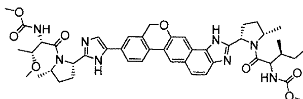
methyl{(3S)-1-[(2S,5S)-2-(9-{2-[(2S,5S)-1-[(2S,3R)-3-methoxy-2-[(methoxycarbonyl) amino]butanoyl)-5-methylpyrrolidin-2-yl]-1H-imidazol-5-yl}-1,11-dihydroisochromeno[4',3':6,7]naphtho[1,2-d]imidazol-2-yl)-5-methylpyrrolidin-1-yl]-3-methyl-1-oxopentan-2-yl}carbamate
