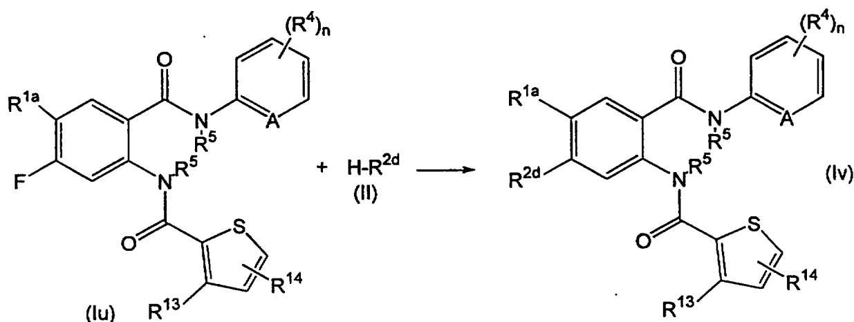
Reaction Scheme 16
