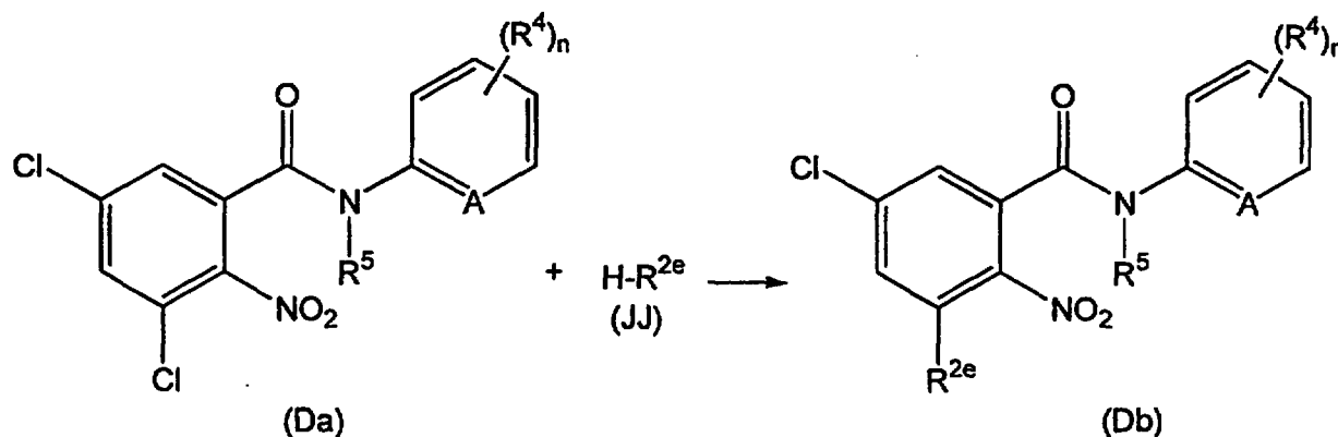
Reaction Scheme 19
