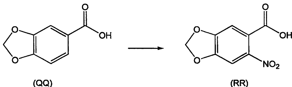
Reaction Scheme 22
