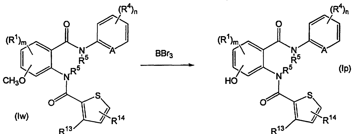
Reaction Scheme 17
