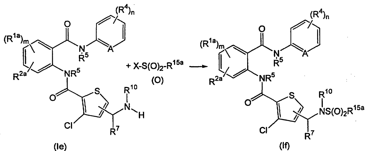
Reaction Scheme 5
