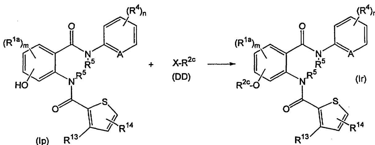
Reaction Scheme 13
