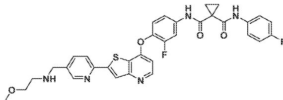
Compound 1 (sitravatinib)
