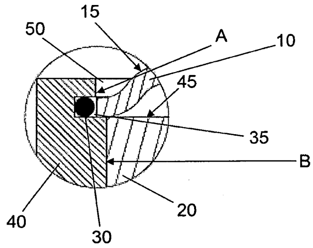
Fig. 2 Detail X
