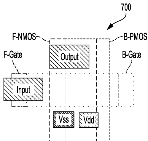
FIG. 7C (combined view 706)
