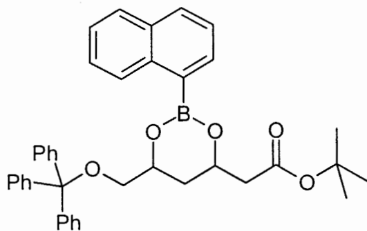
Formula VIa
