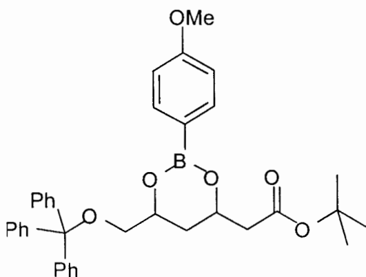
Formula VIc
