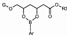
Formula VI
