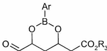
Formula VIII
