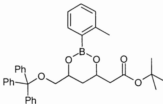
Formula VIb
