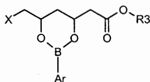
Formula IX
