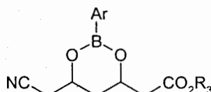
Formula VII
