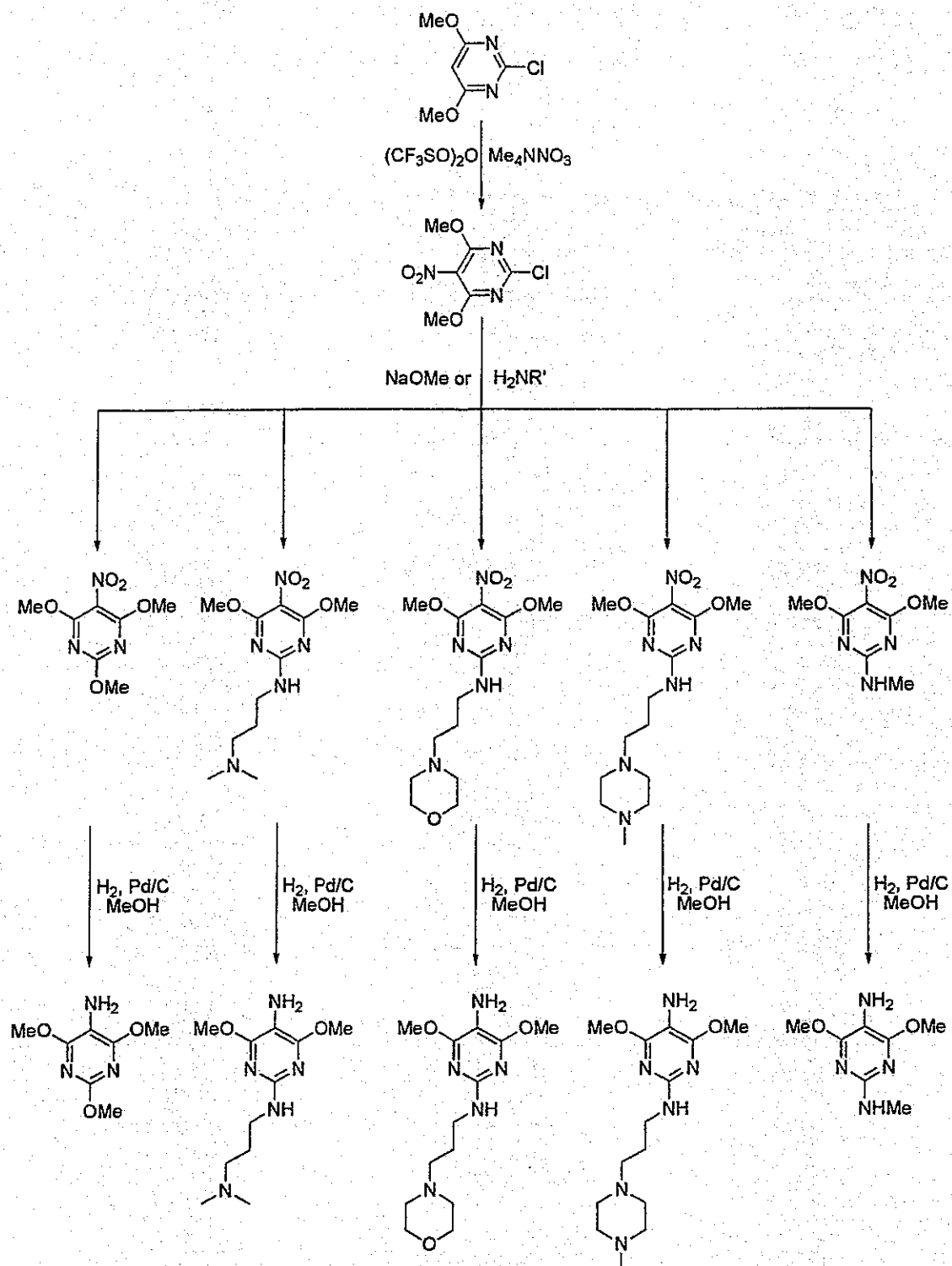
Scheme 4
