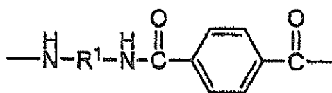
Structural formula a
