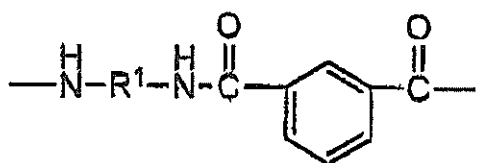
Structural formula b
