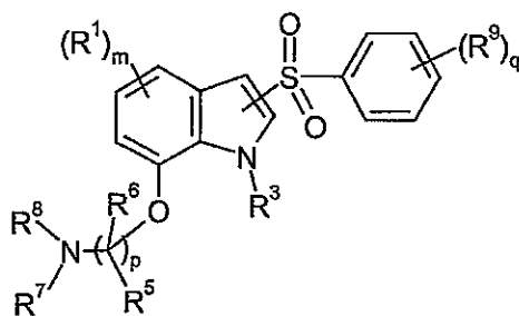
Ia1
