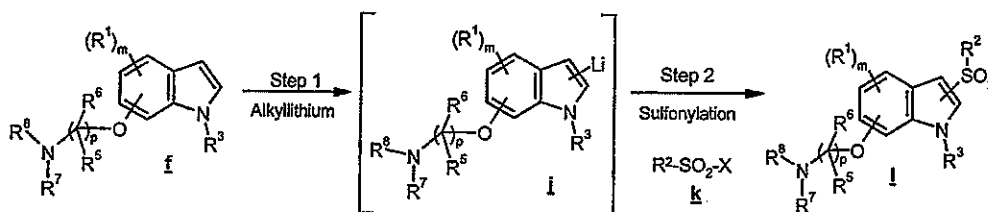
SCHEME B
