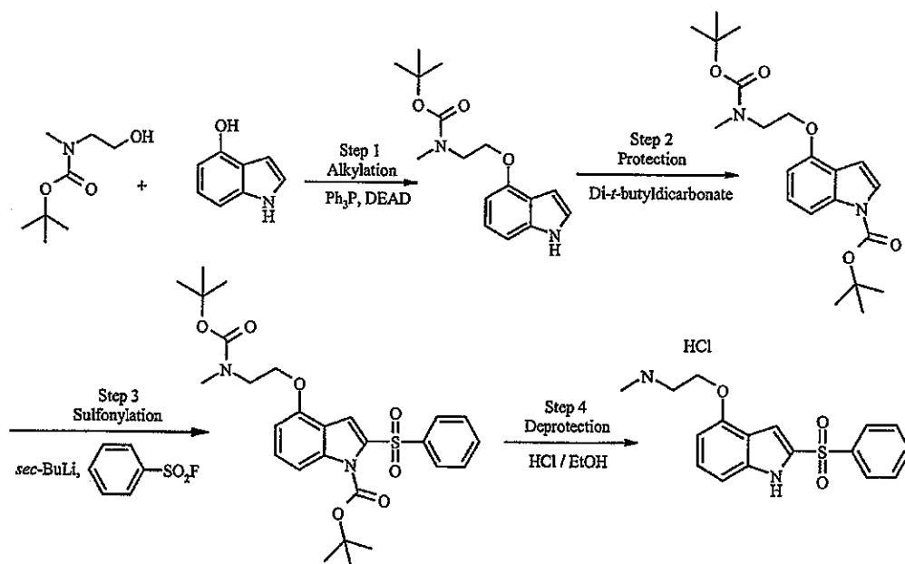
SCHEME F
