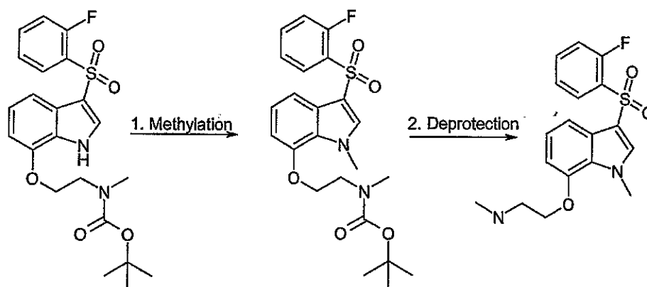
SCHEME E
