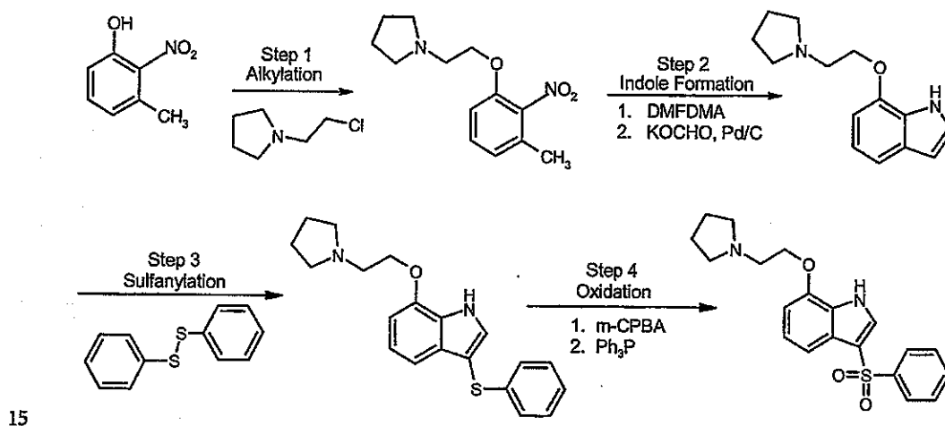
SCHEME C
