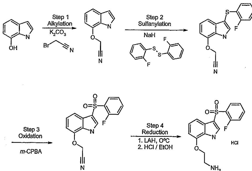
SCHEME I
