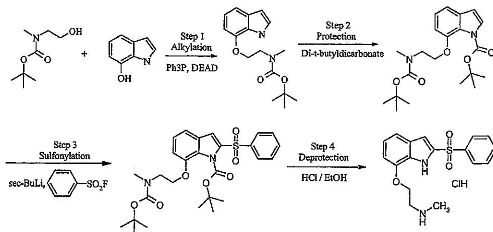
SCHEME G
