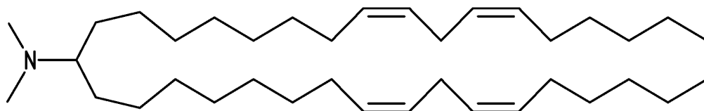
CLX ((6Z,9Z,26Z,29Z)-N,N-dimethylpentatriaconta-6,9,26,29-tetraen-18-amine)
