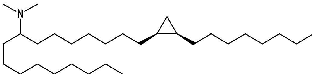
CLY (N,N-dimethyl-1-((1S,2R)-2-octylcyclopropyl)heptadecan-8-amine)
