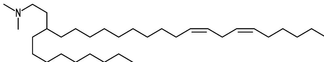
CLA ((13Z,16Z)-N,N-dimethyl-3-nonyldocosa-13,16-dien-1-amine)
