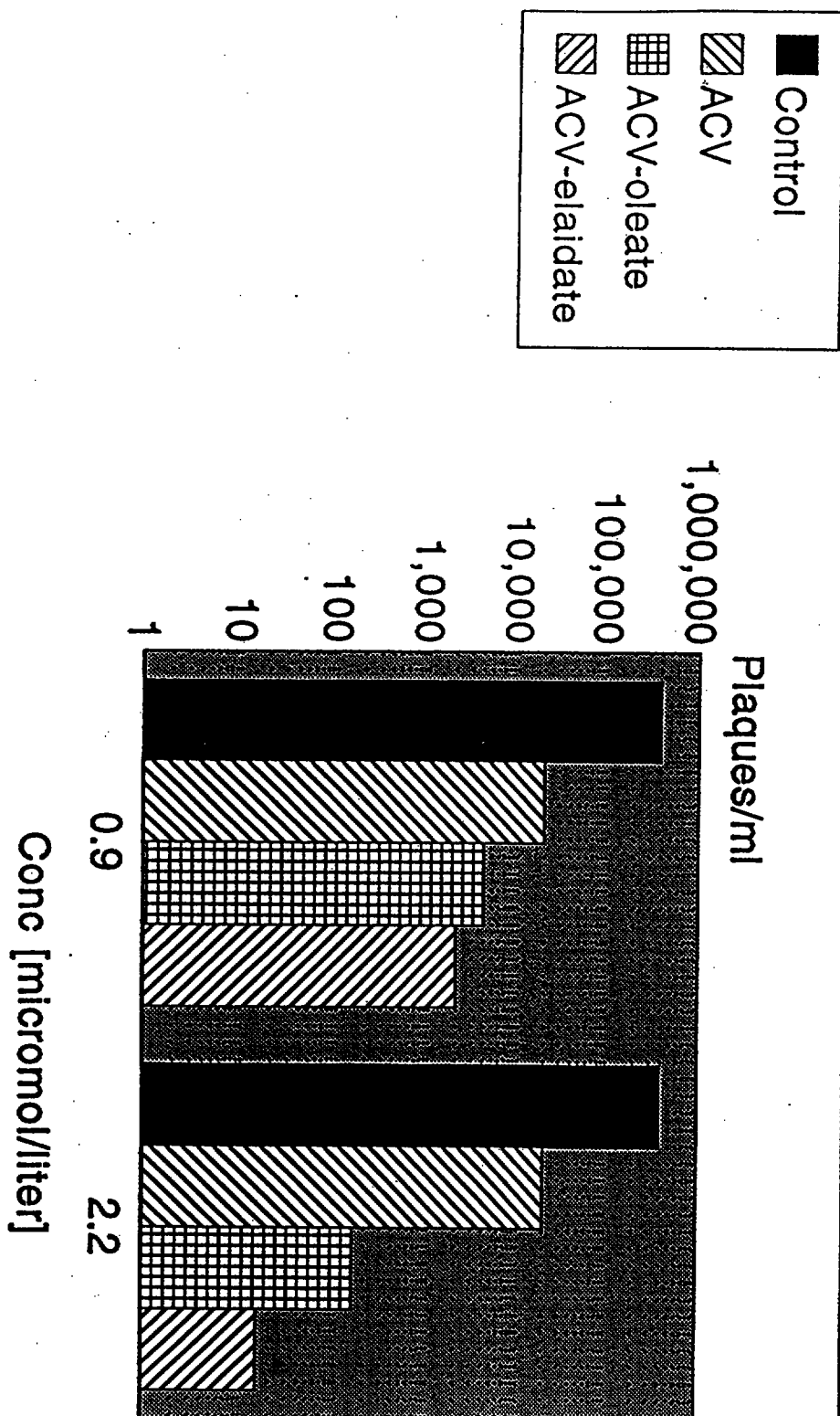
Figure 1b Effect of ACV esters on HSV 2
