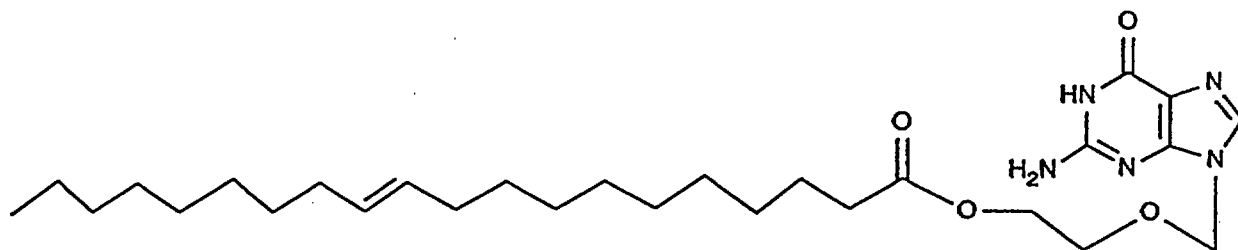
ACV eicosenate, trans
