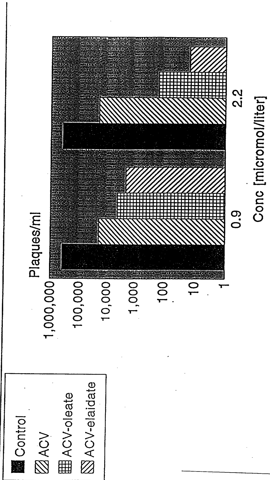
Figure 1b Effect of ACV esters on HSV 2
