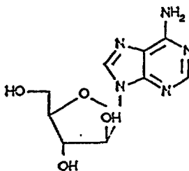
Arabino-furanosyl adenine (Ara A)
