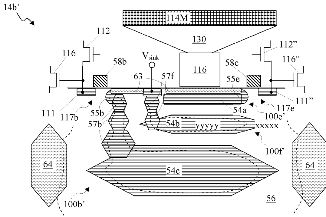
FIG. 19 (Depletion Regions Pinched)
