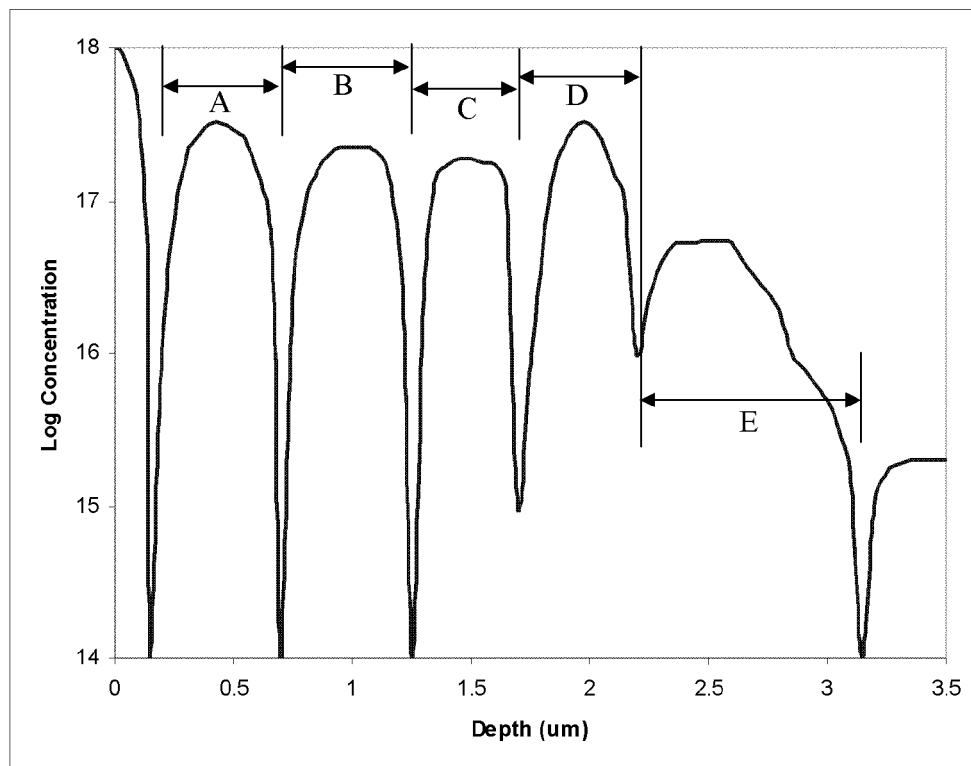
FIG. 9 (Doping Profile)
