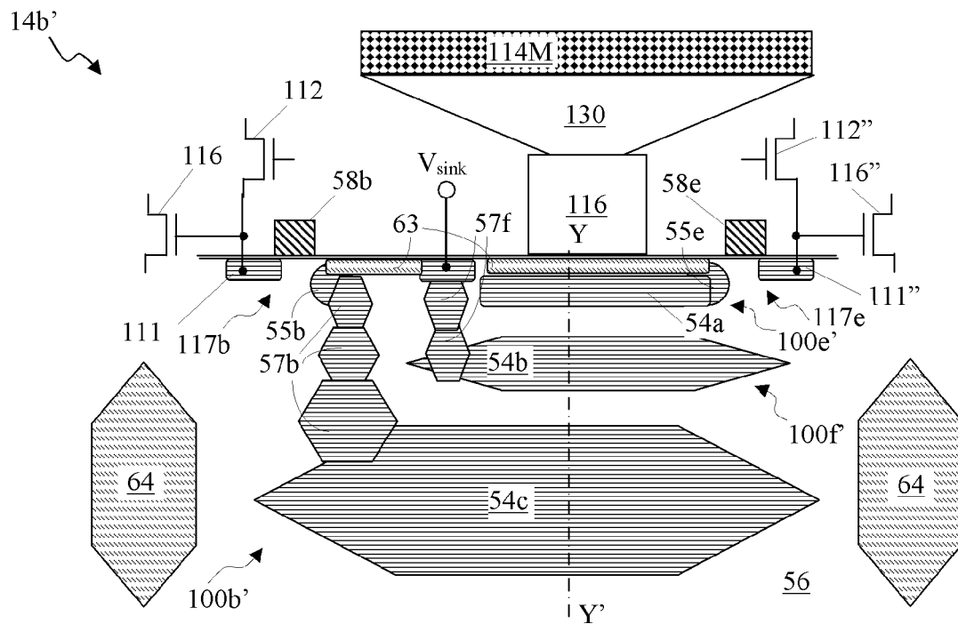
FIG. 17 (Magenta Pixel, 2 nd embodiment)
