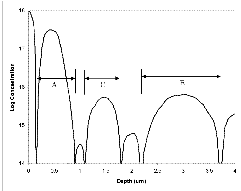
FIG. 18 (Doping profile, 2nd embodiment)
