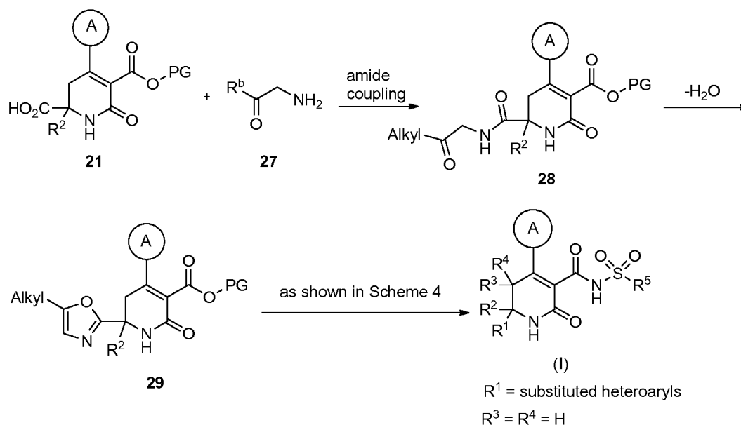
Scheme 8
