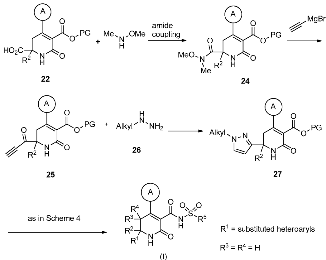
Scheme 7
