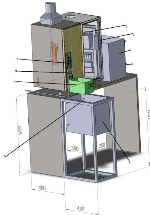
Figure 1a : Overview Drawing on a larger scale
