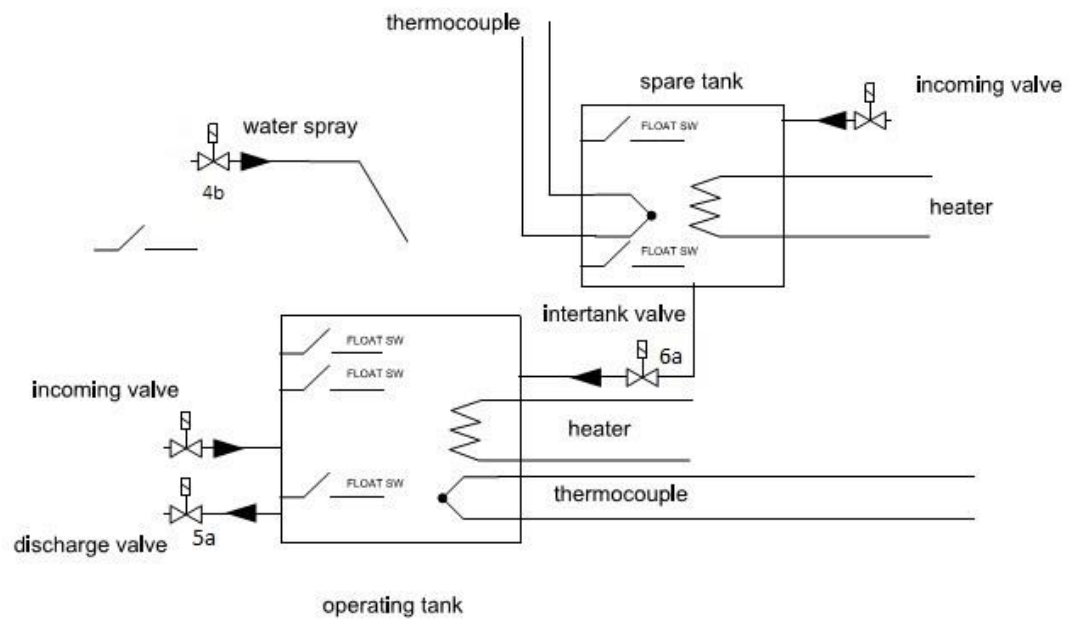
Figure 6 water tank schematic drawing
