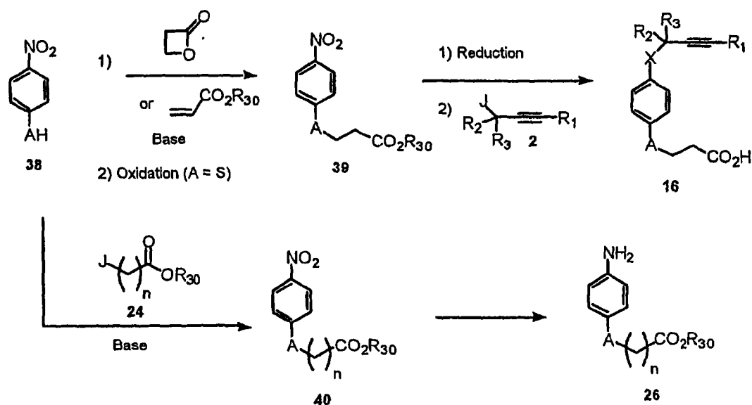
Scheme 8:
