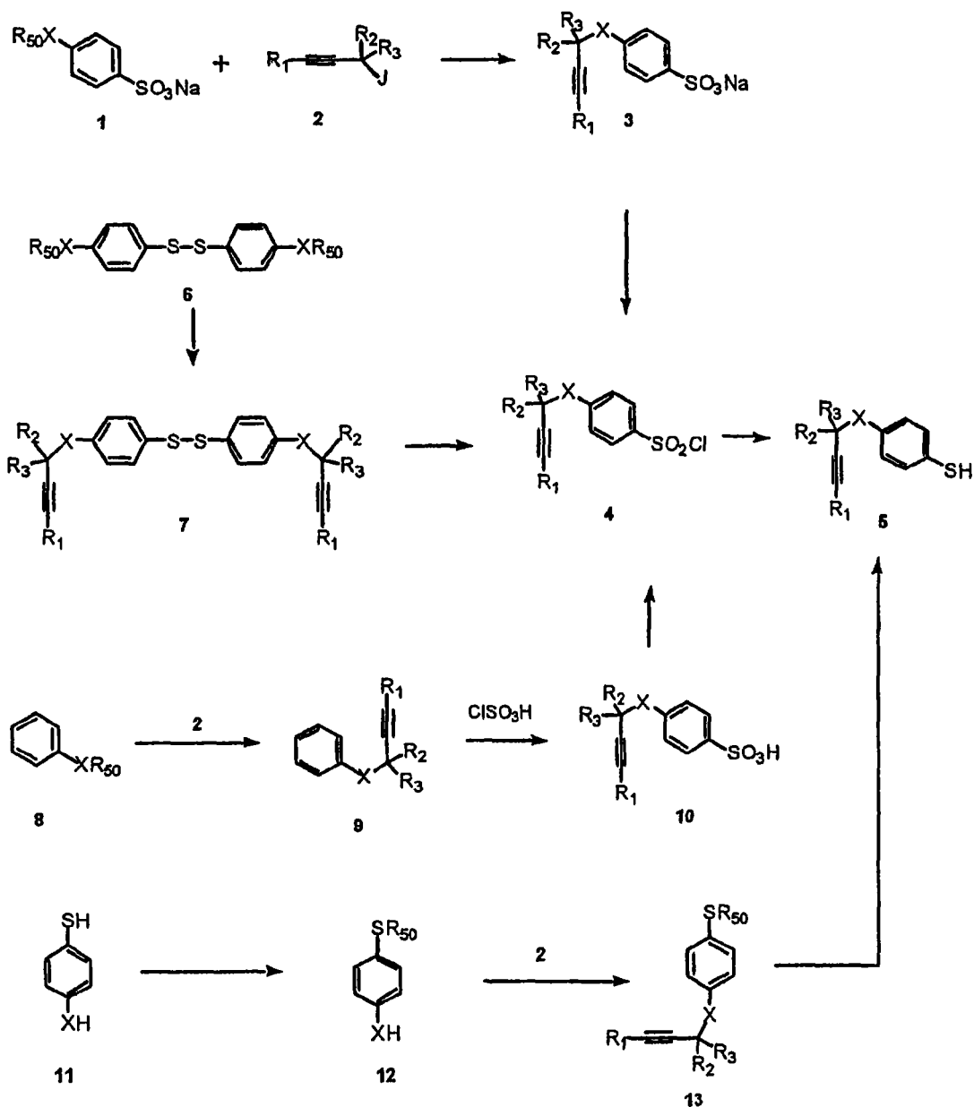
Scheme 3:
