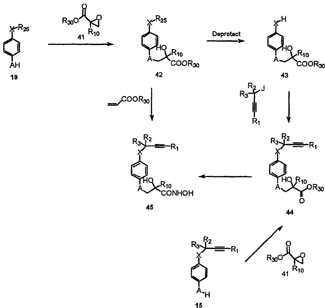
Scheme 9:
