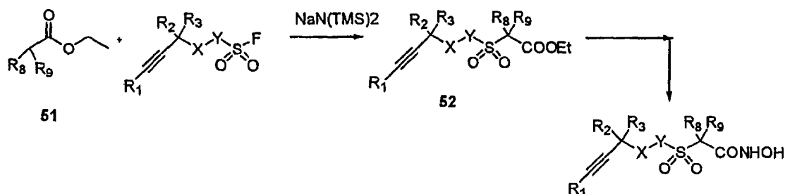
SCHEME 12
