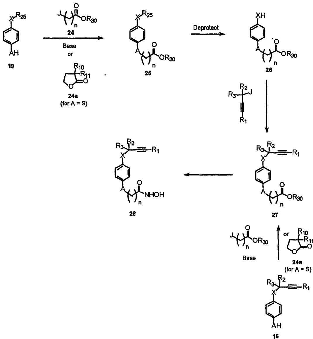
Scheme 5:
