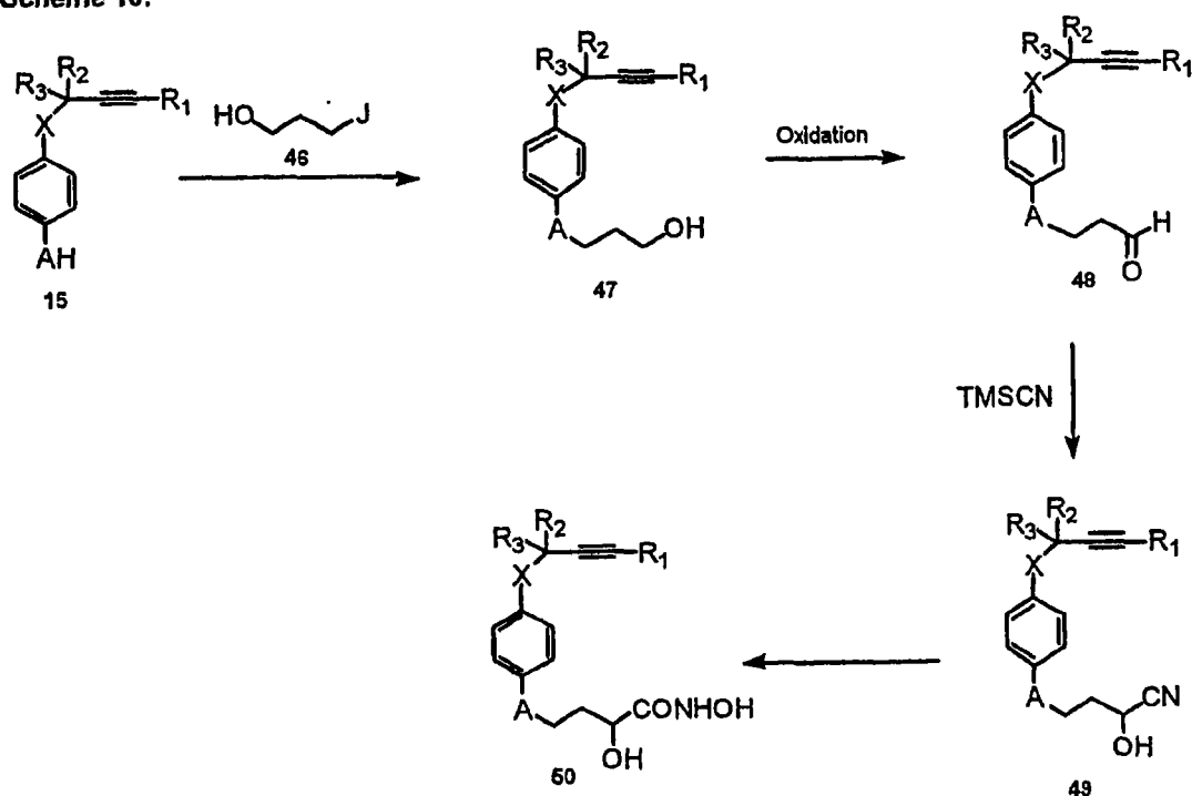
Scheme 10:
