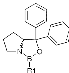
(IA) alkyl-CBS
