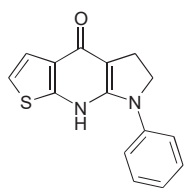
(Compound 2b)
