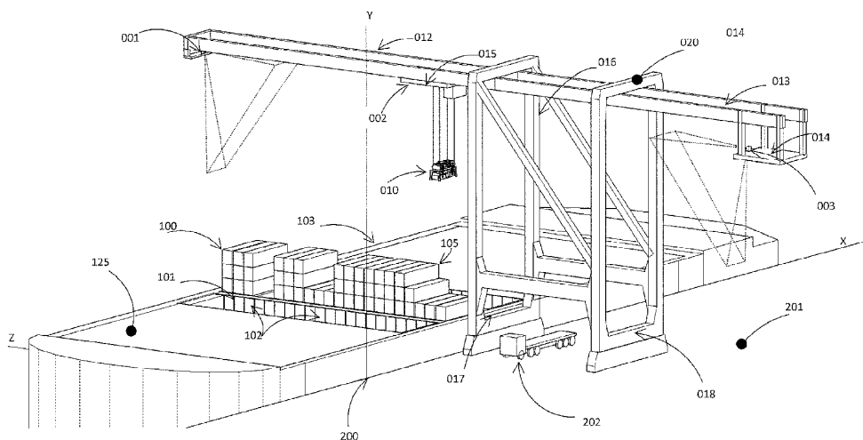
Figure 1: Apparatus preferred embodiment view 1
