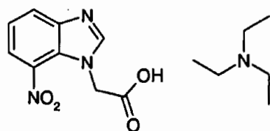
1) (7-Nitro-1H-benzimidazol-1-yl)acetic acid (triethylammonium salt)
