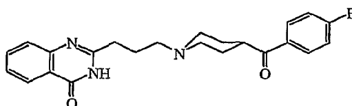
Compound 14
