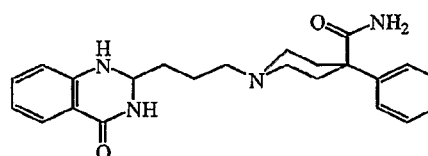
Compound 5
