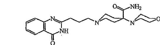
Compound 11
