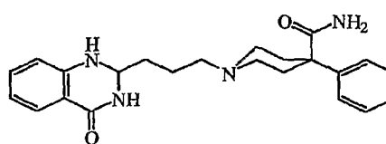
Compound 5
