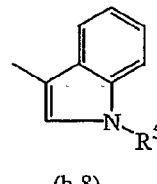
(b-8)
