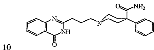
Compound 4
