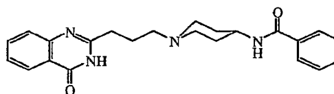
Compound 12
