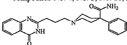
Compound 4
