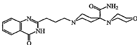
Compound 11
