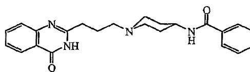
Compound 12
