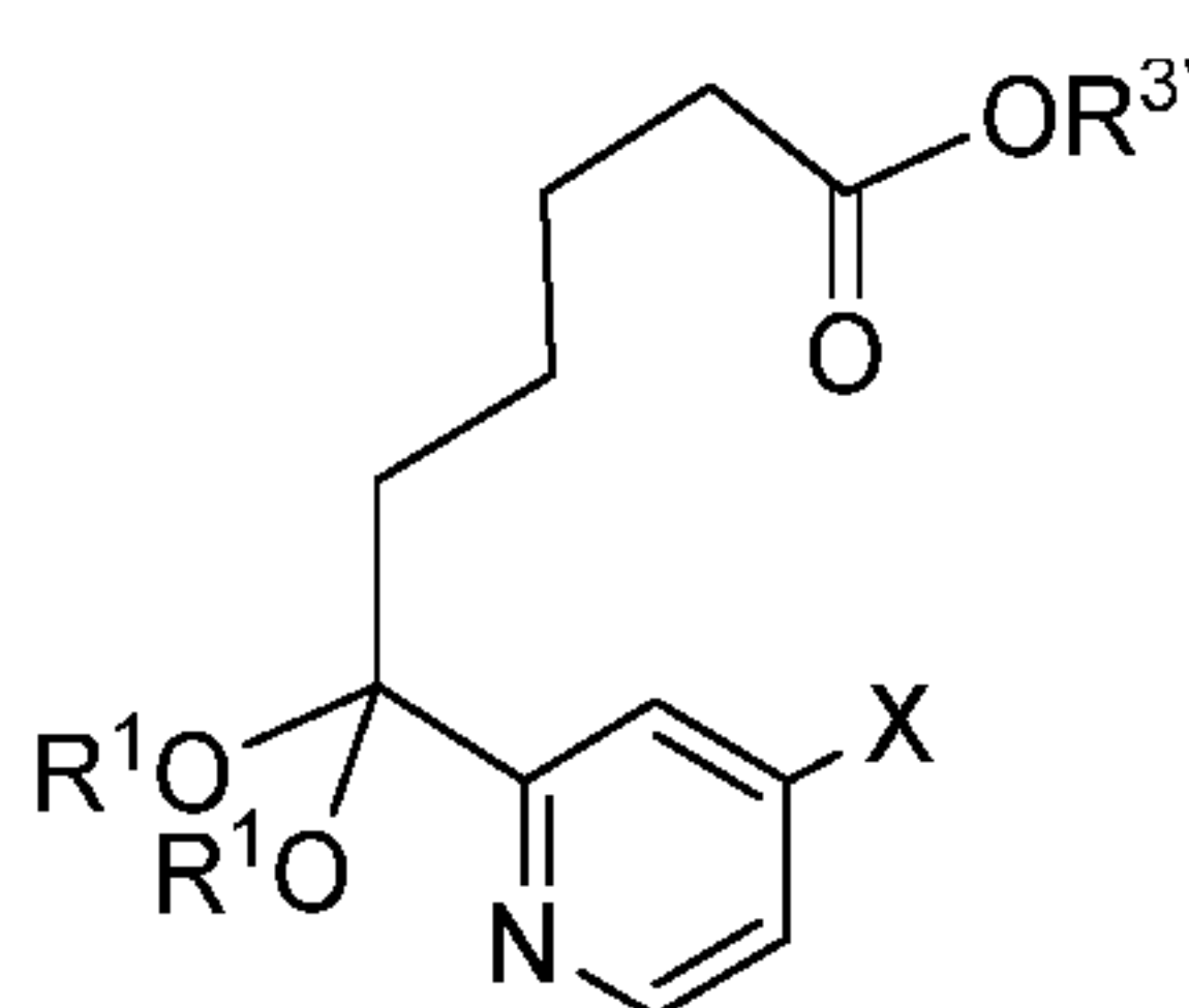
Compound 5
