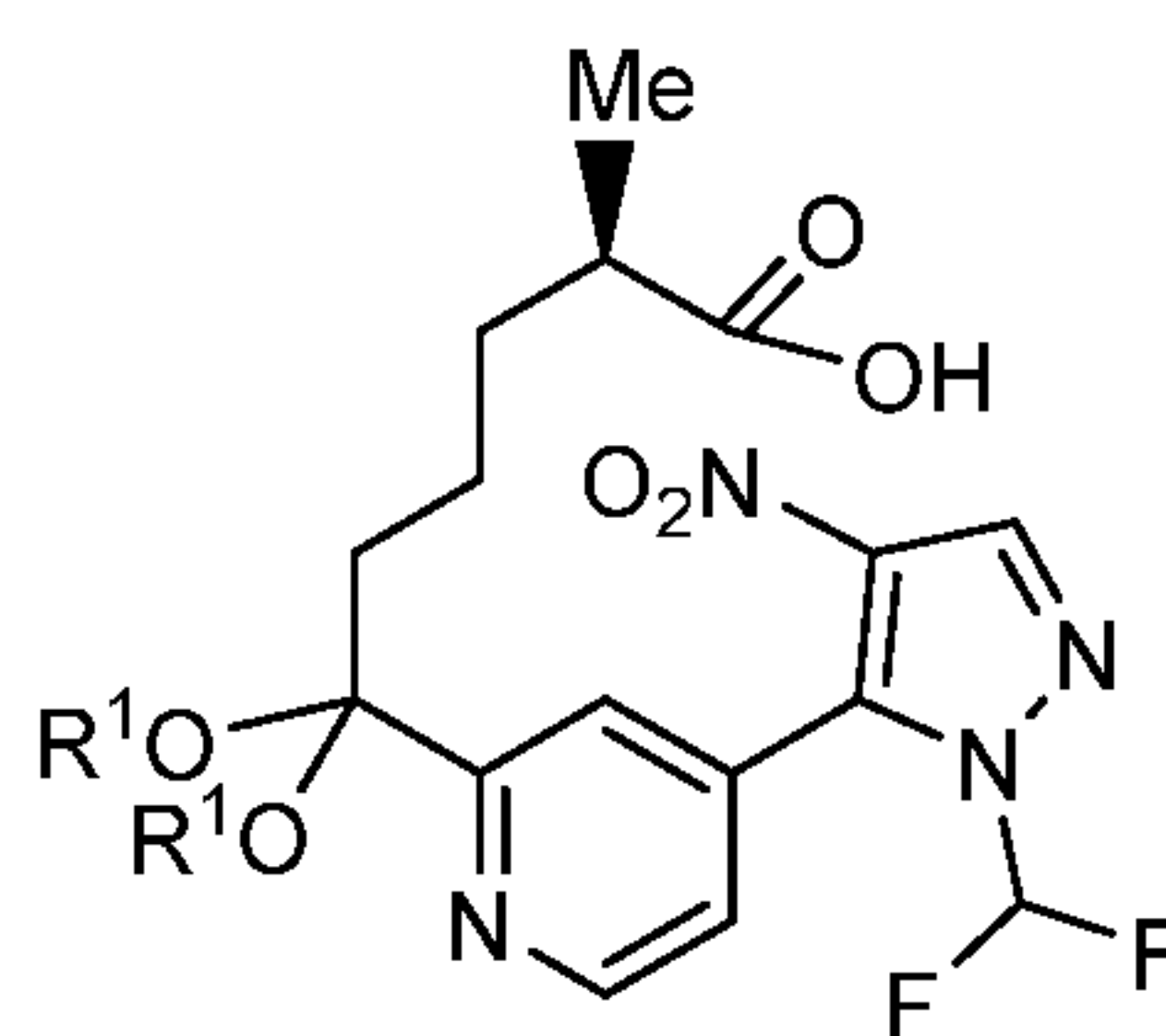
Compound 9;
