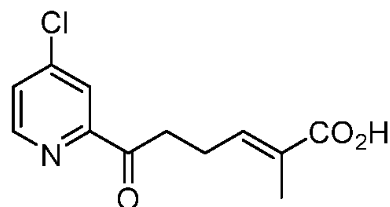
Compound 18a;
