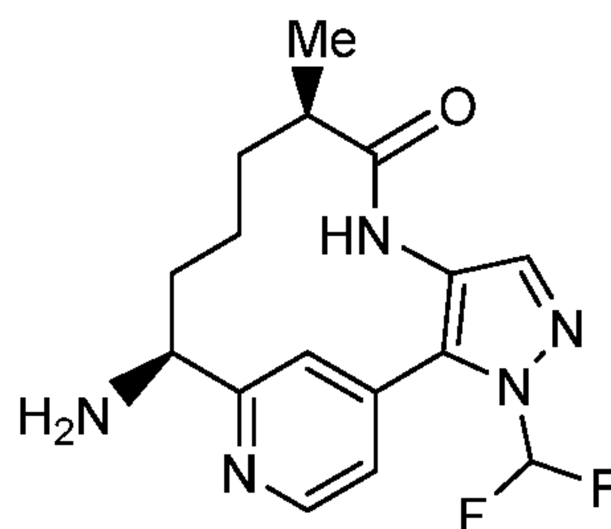
Compound 13;
