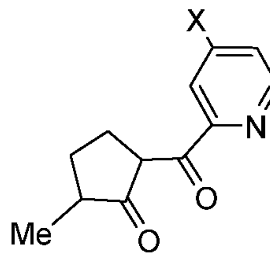
Compound 23b
