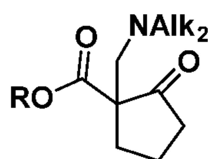
Compound 40,
