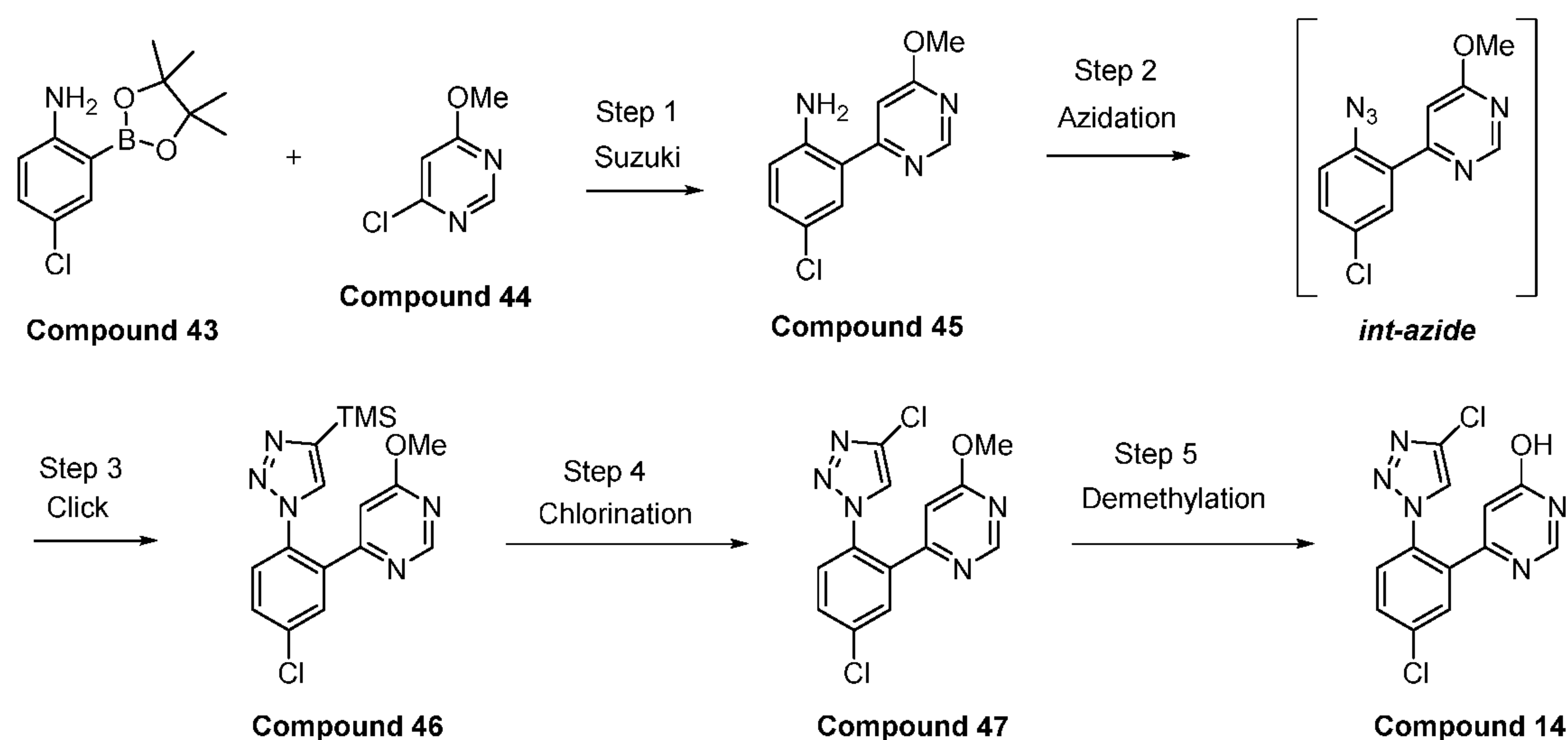
Scheme 9
