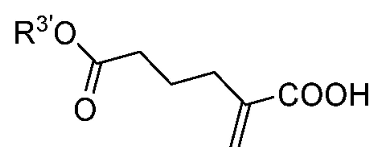
Compound 42
