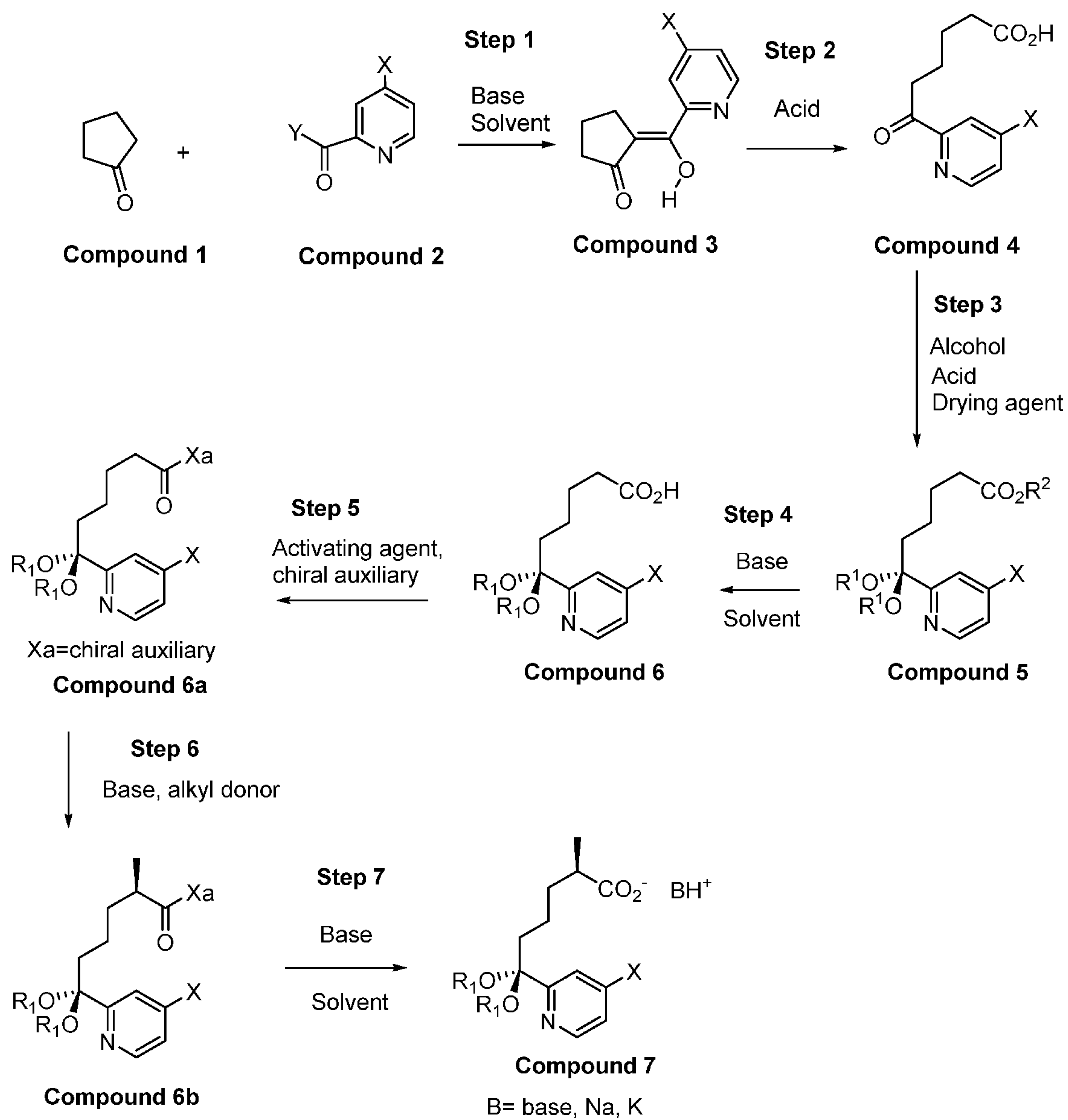
Scheme 1
