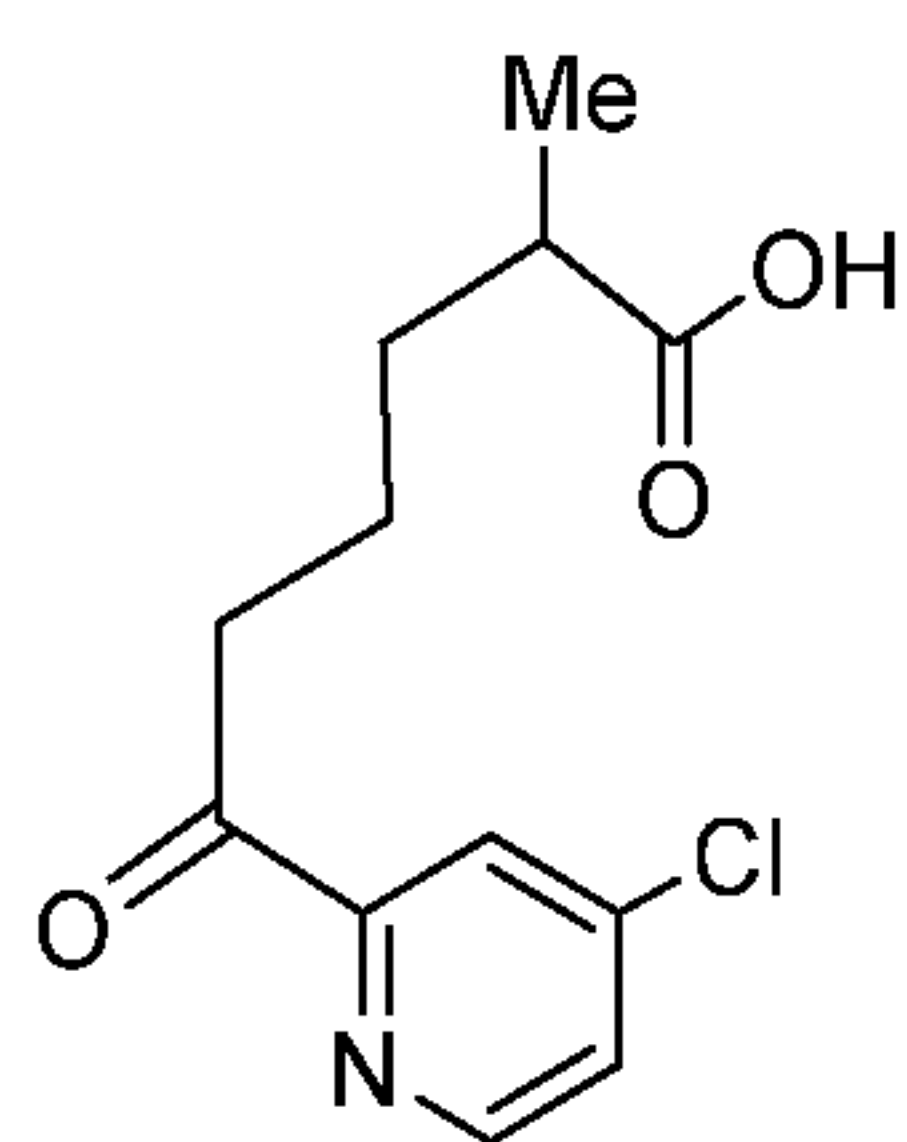
Compound 34.
