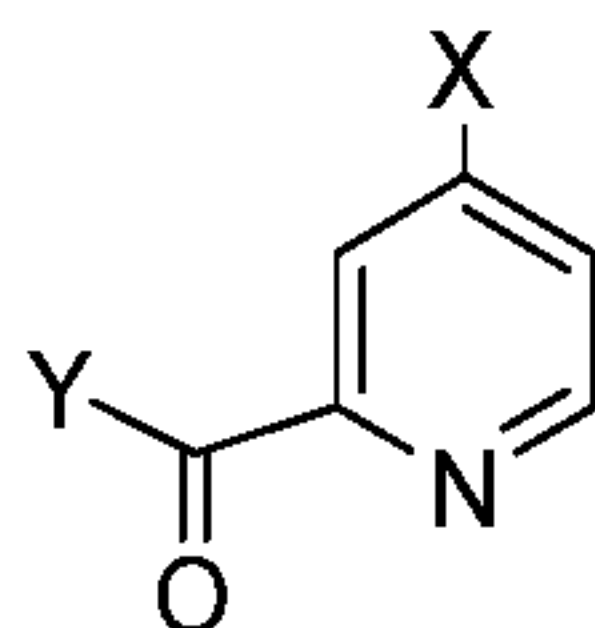
Compound 2
