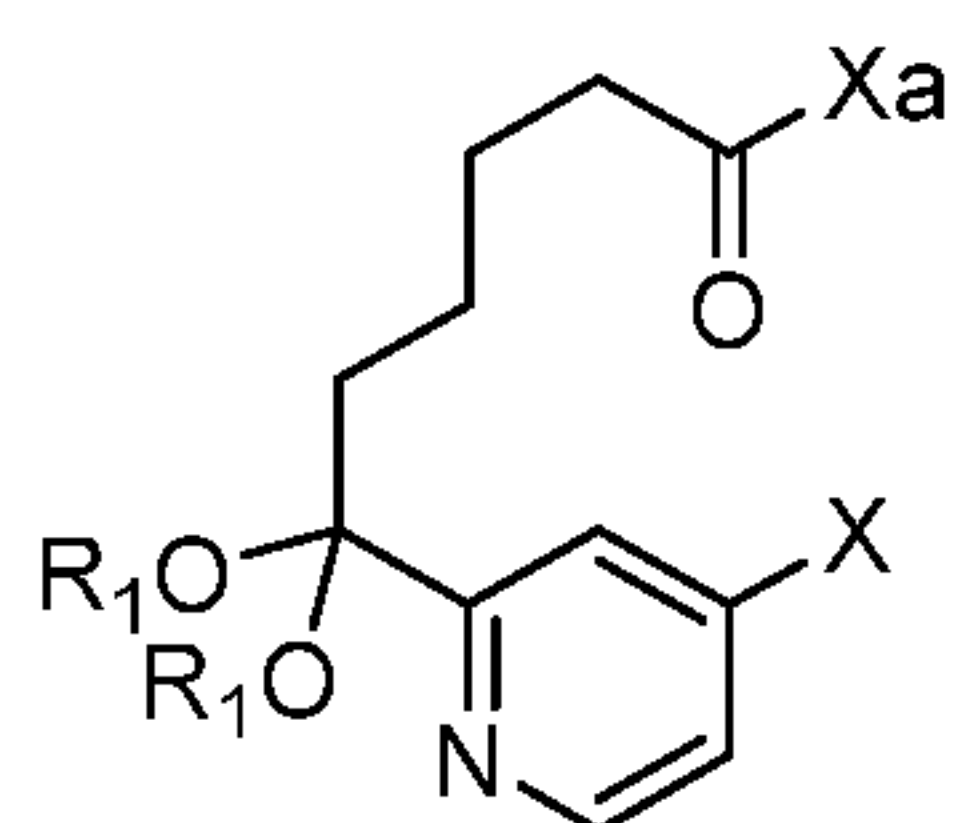
Compound 6a
