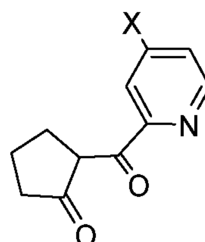
Compound 3b.
