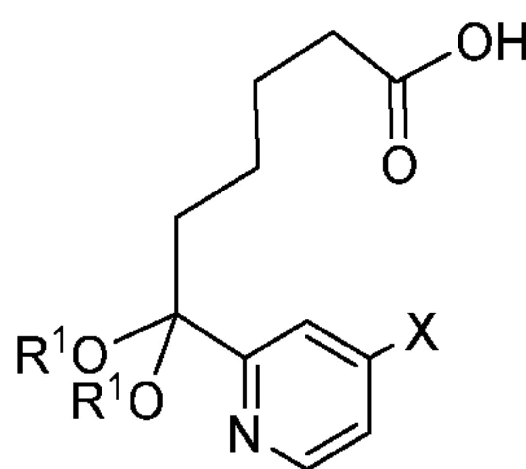
Compound 6
