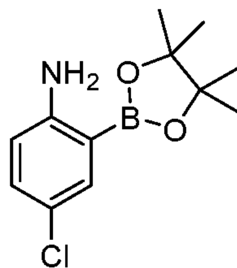
Compound 43
