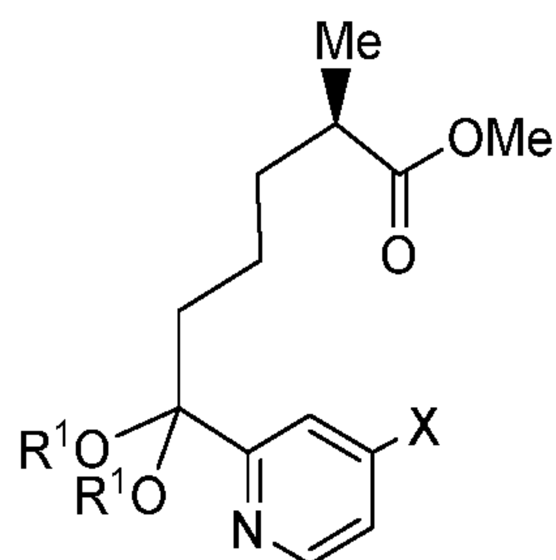
Compound 26
