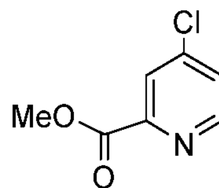
Compound 2a
