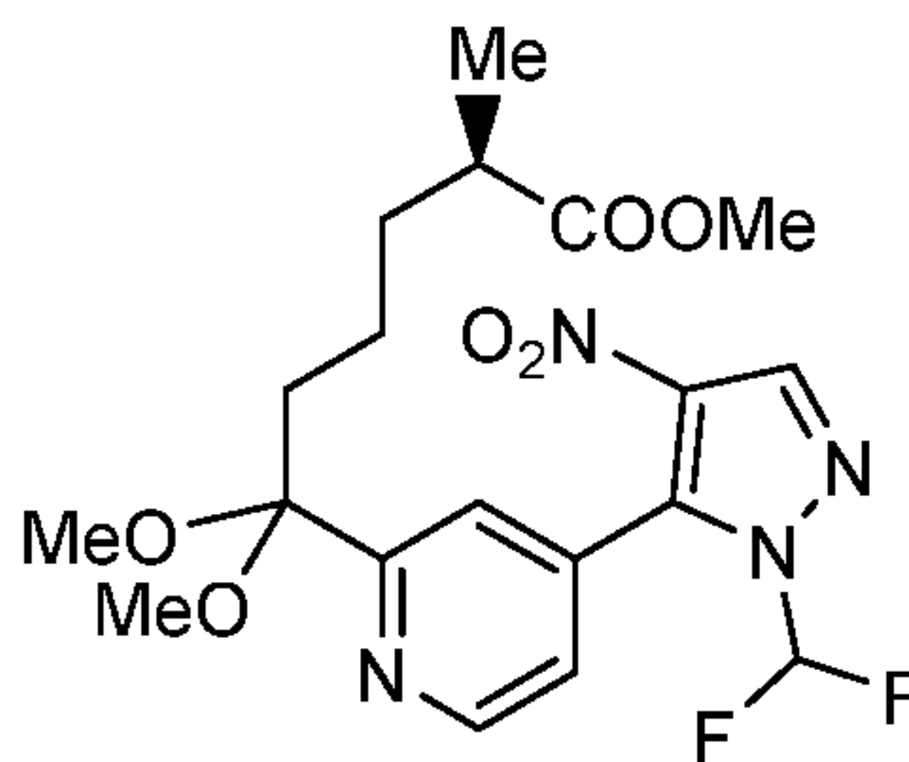
Compound 33.
