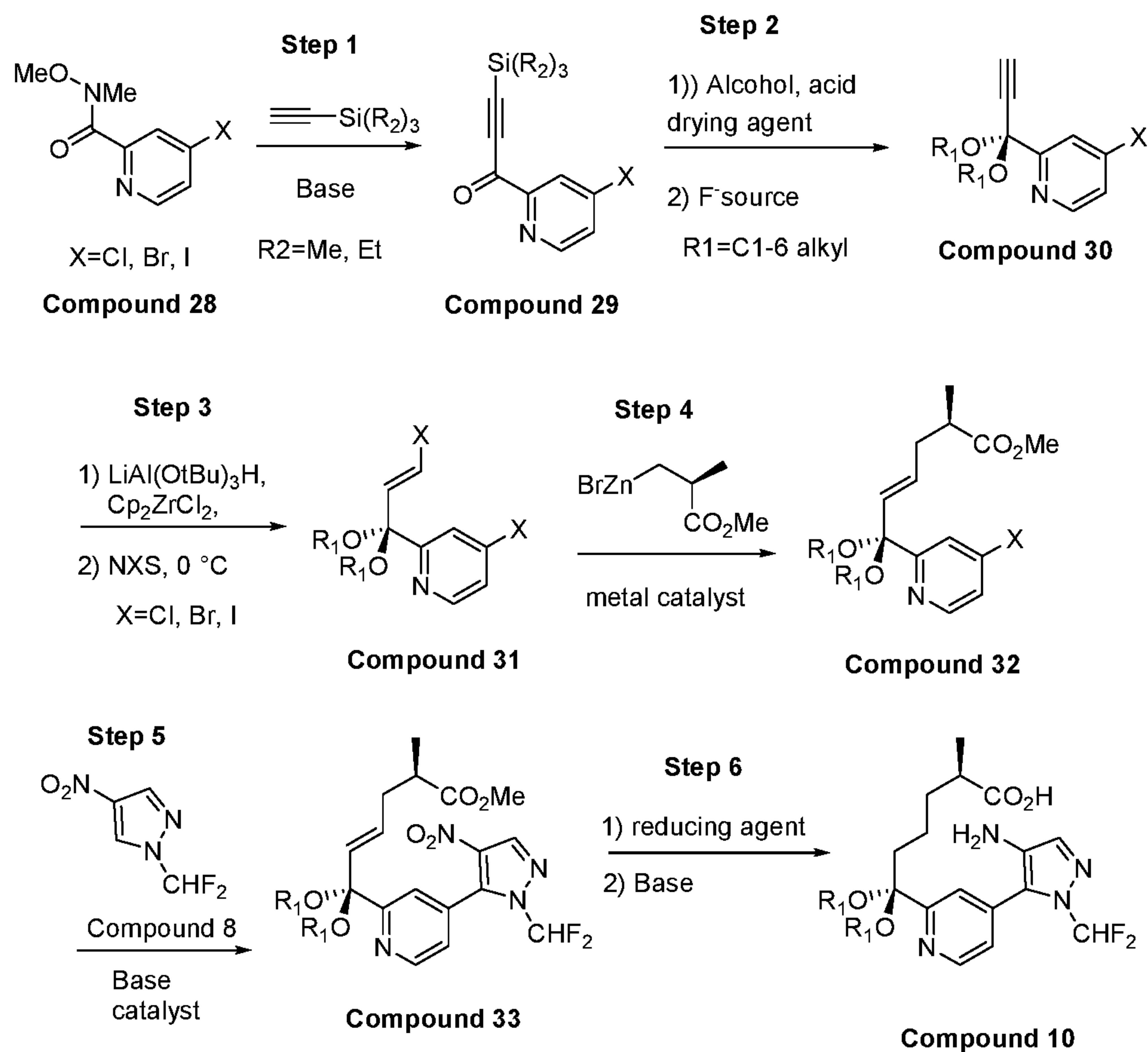
Scheme 8
