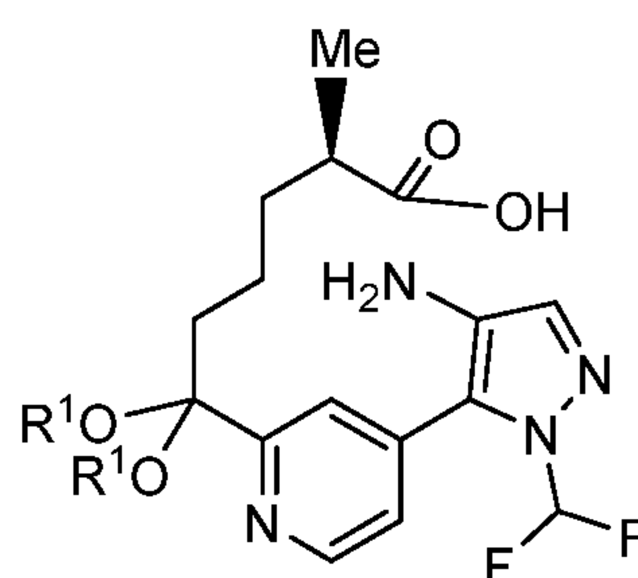
Compound 10;
