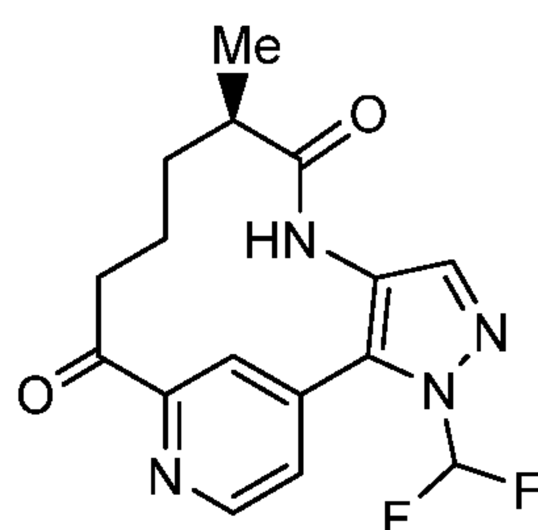
Compound 12;
