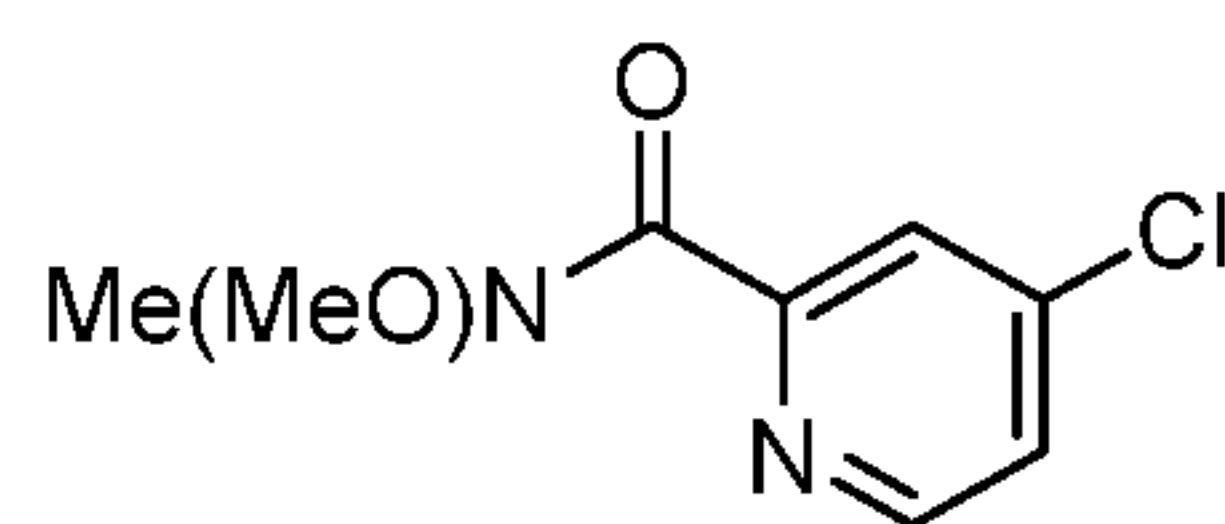
Compound 15
