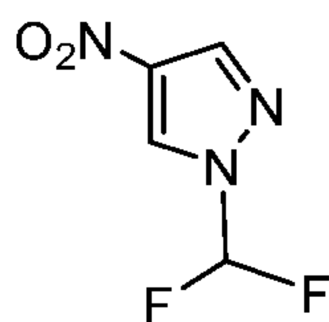
Compound 8
