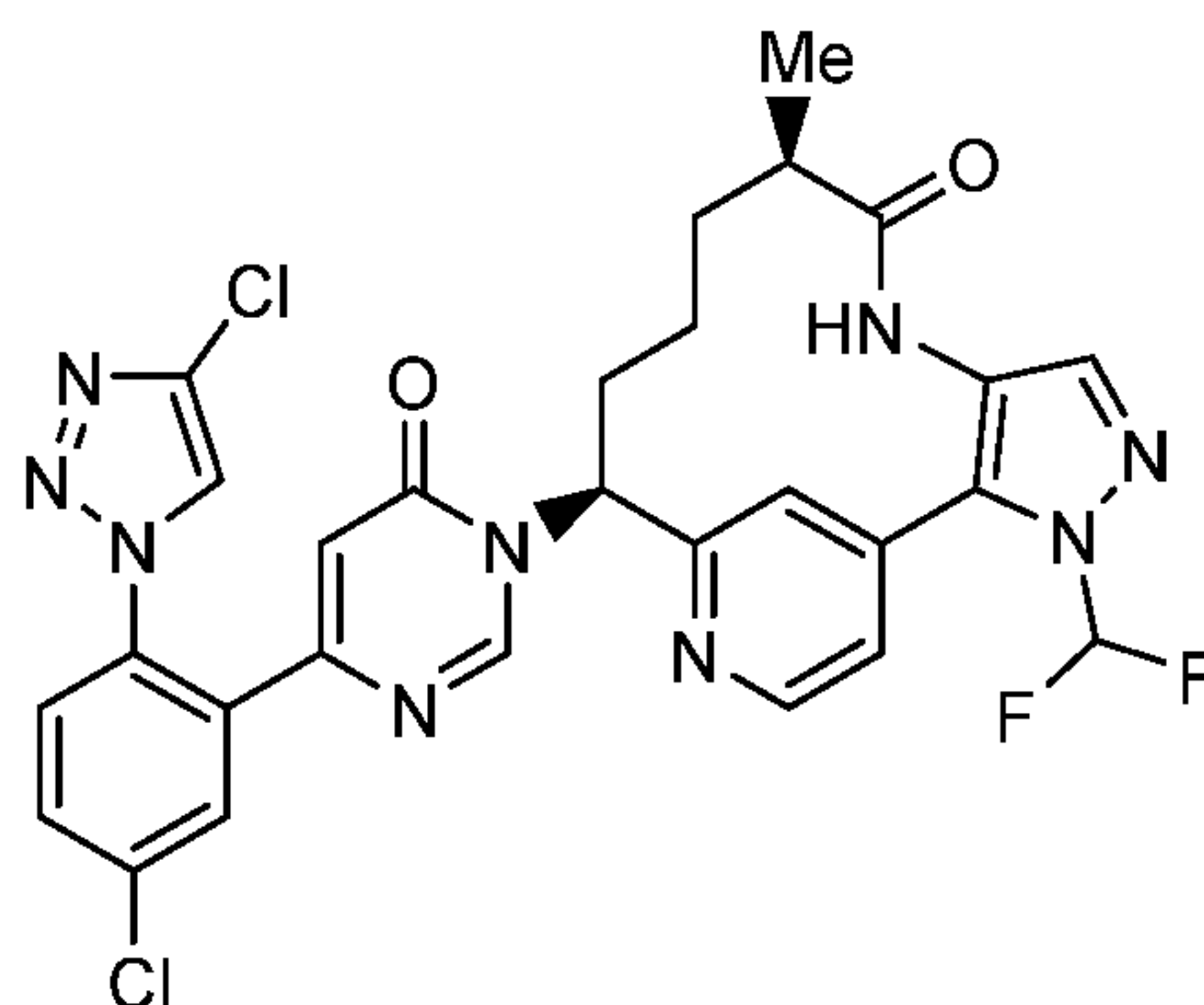
Compound (I).
