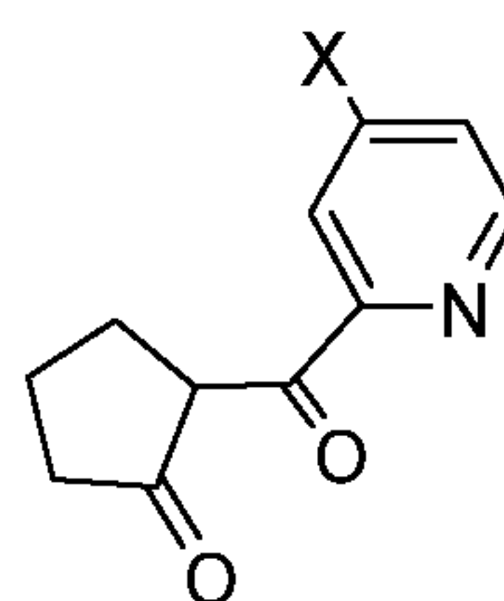
Compound 3b,
