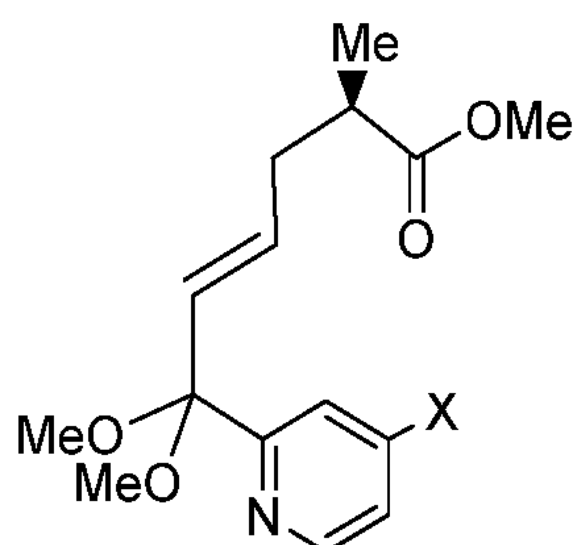
Compound 32
