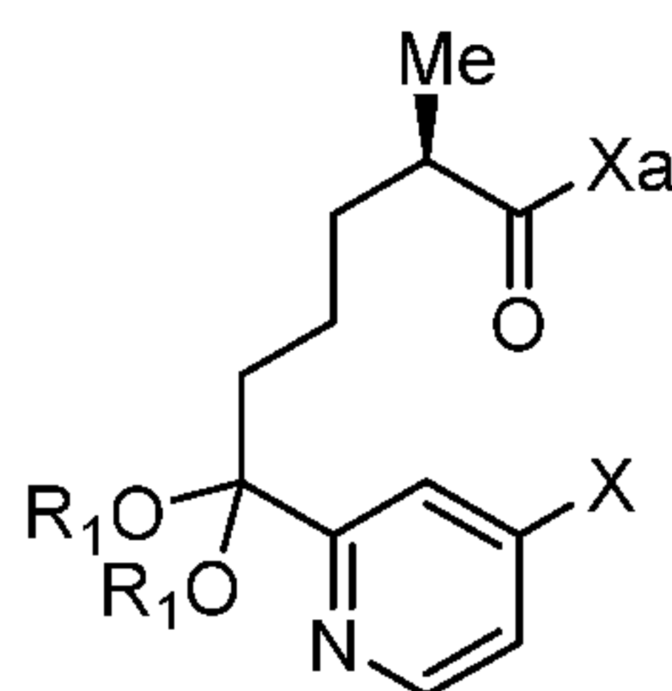
Compound 6b
