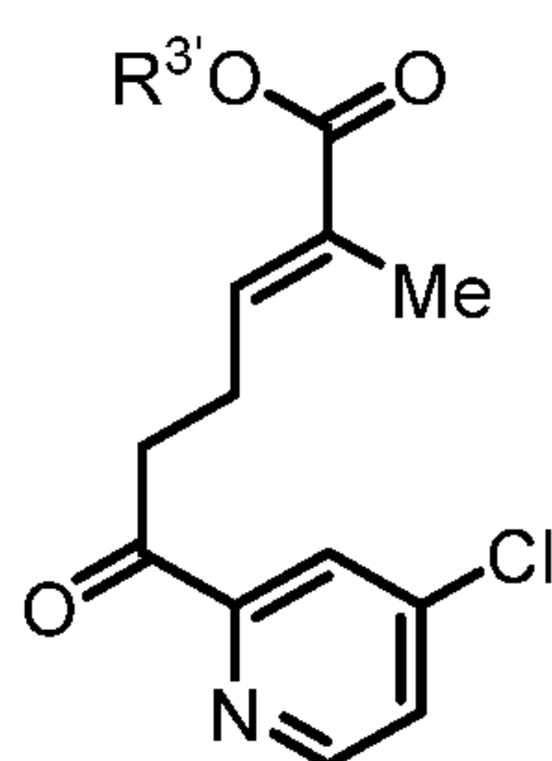
Compound 18
