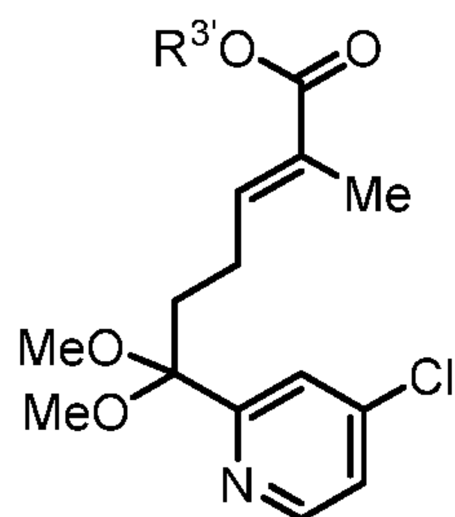
Compound 19
