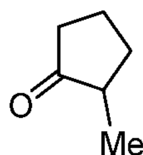
Compound 22
