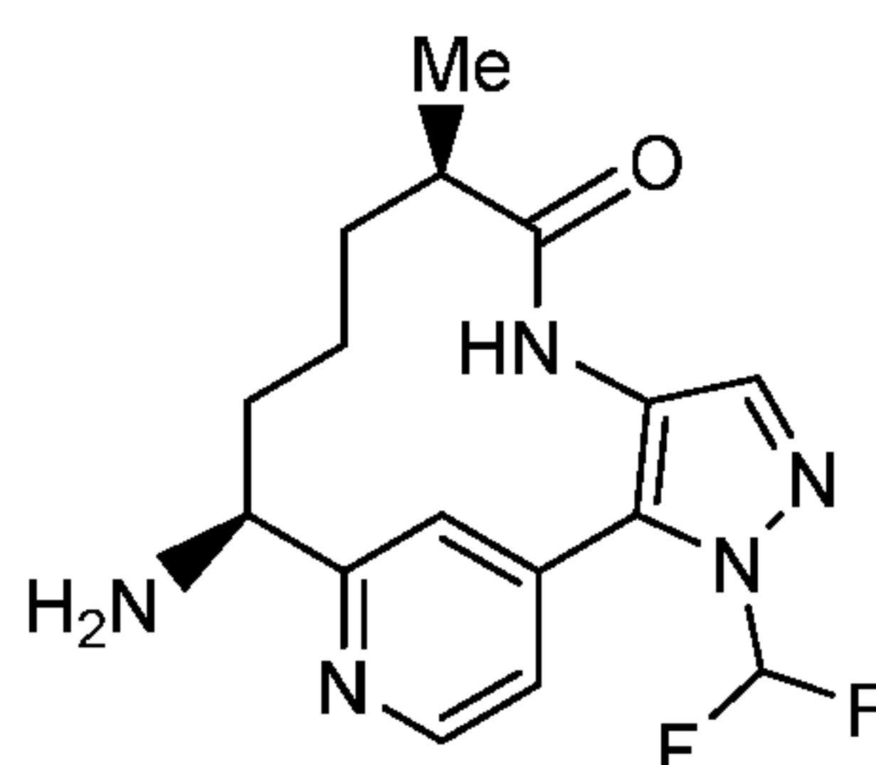
Compound 13
