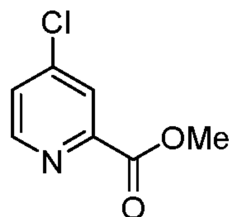
Compound 2a
