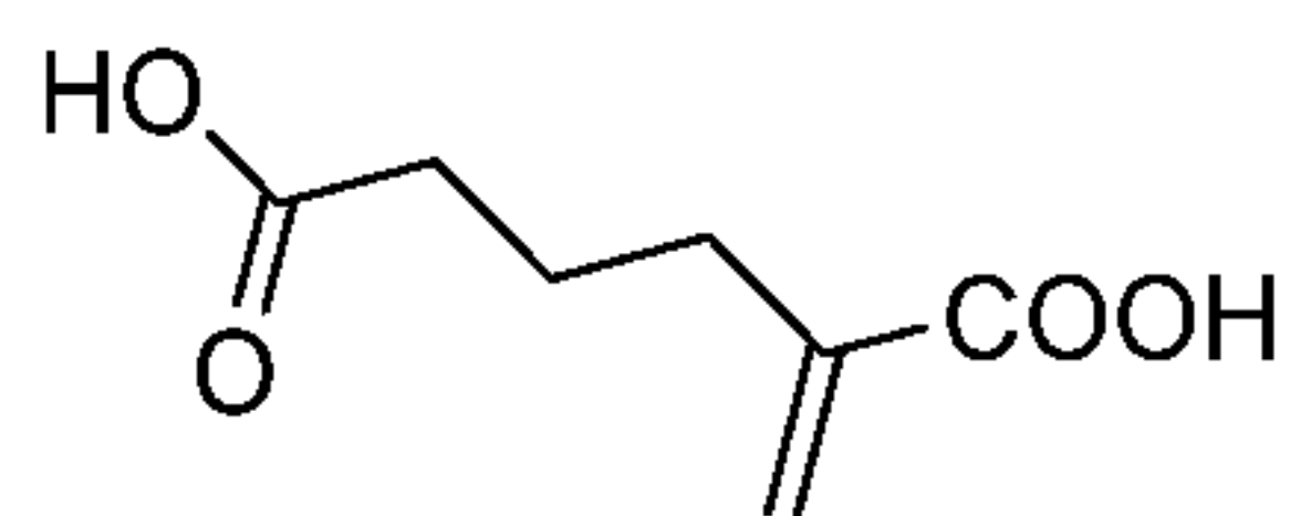
Compound 41;
