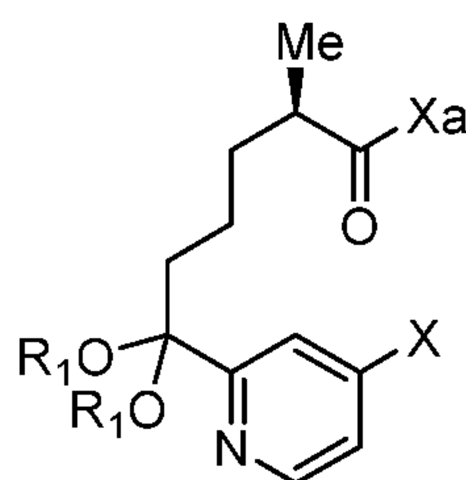
Compound 6b
