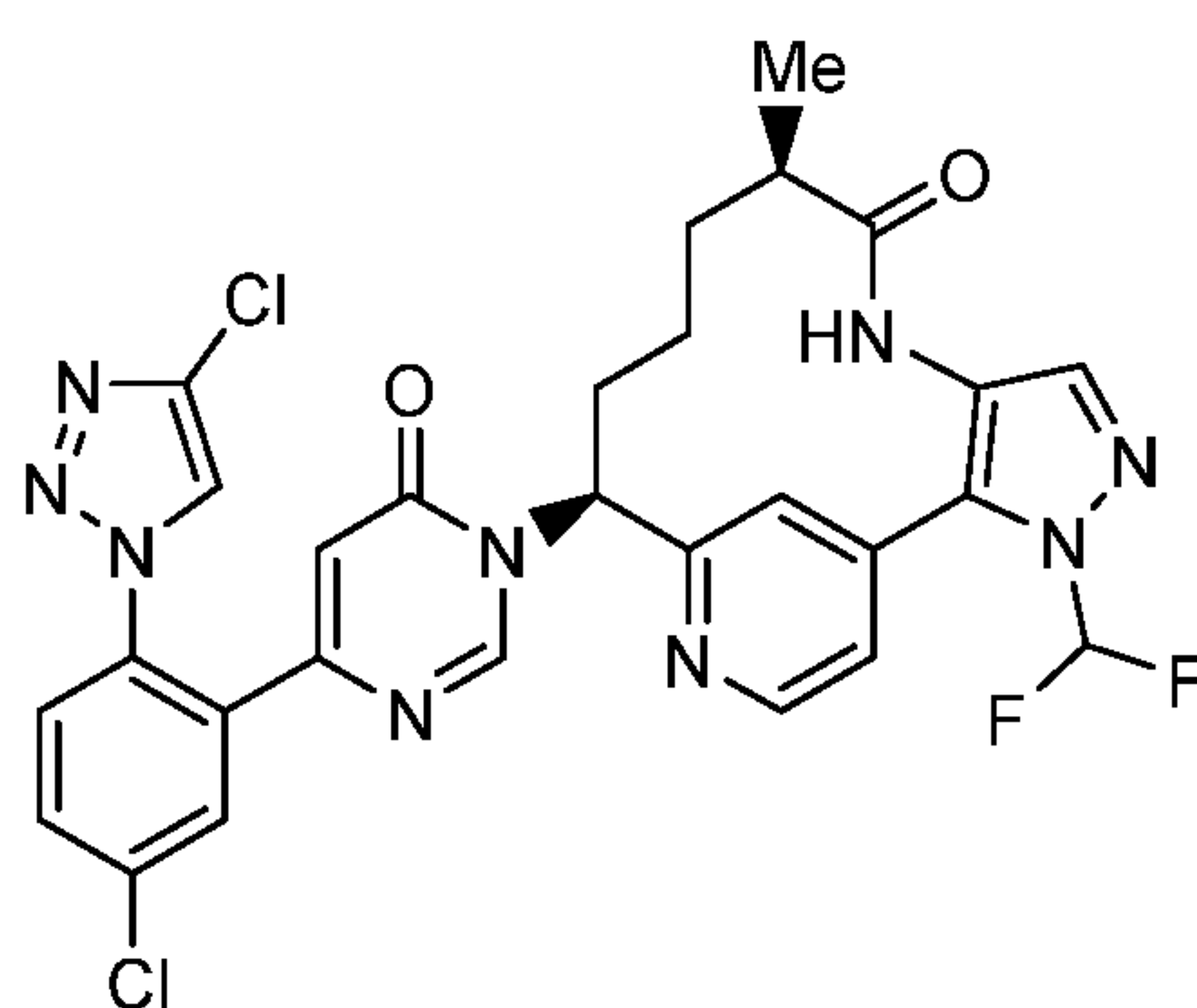
Compound (I).
