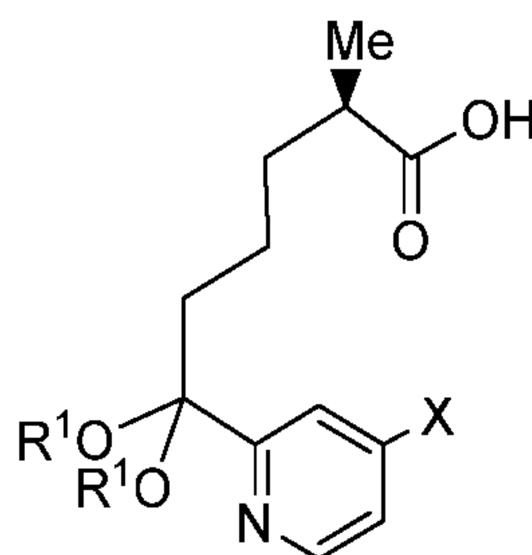
Compound 7
