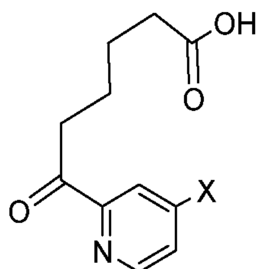
Compound 4
