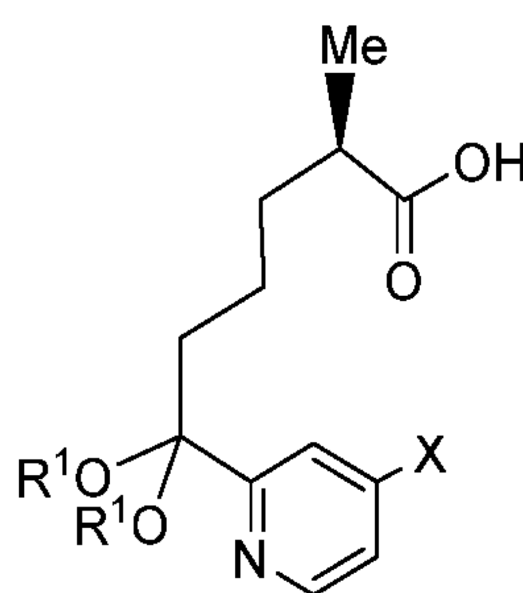
Compound 7
