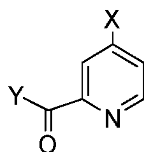
Compound 2
