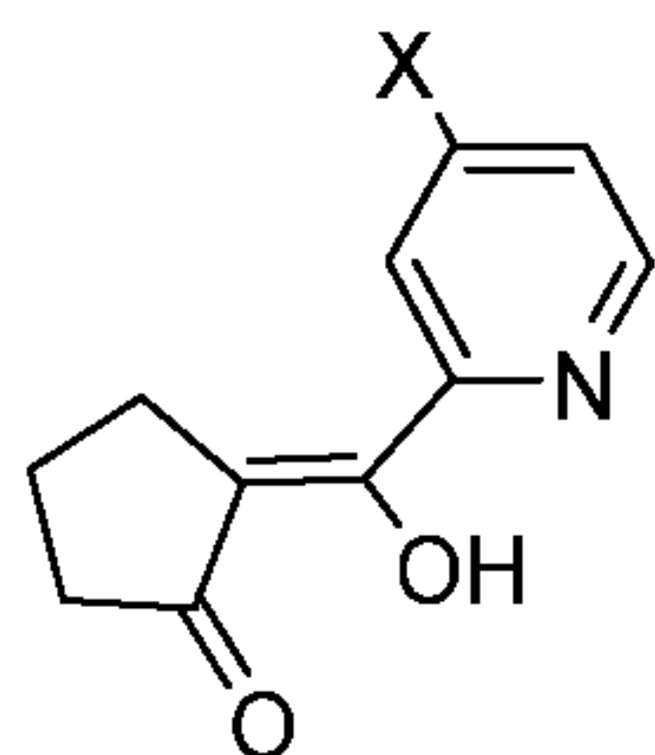
Compound 3a
