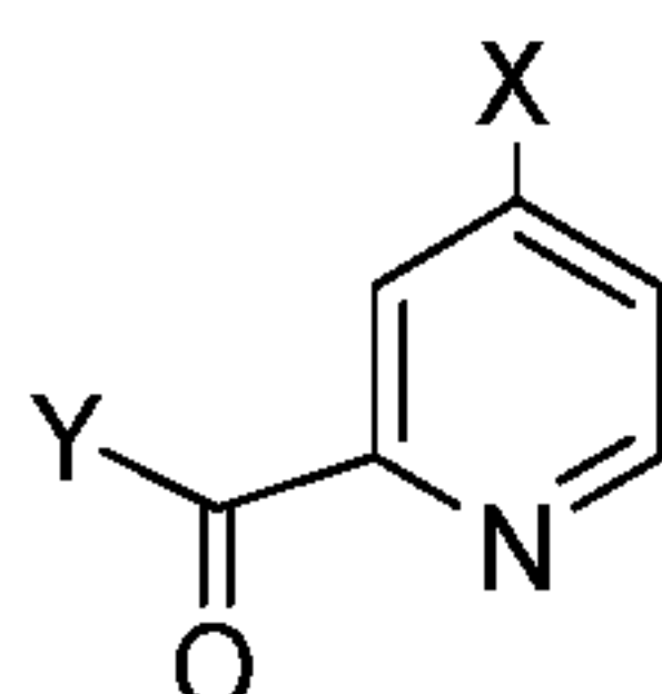
Compound 2
