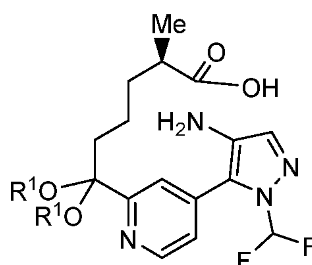
Compound 10
