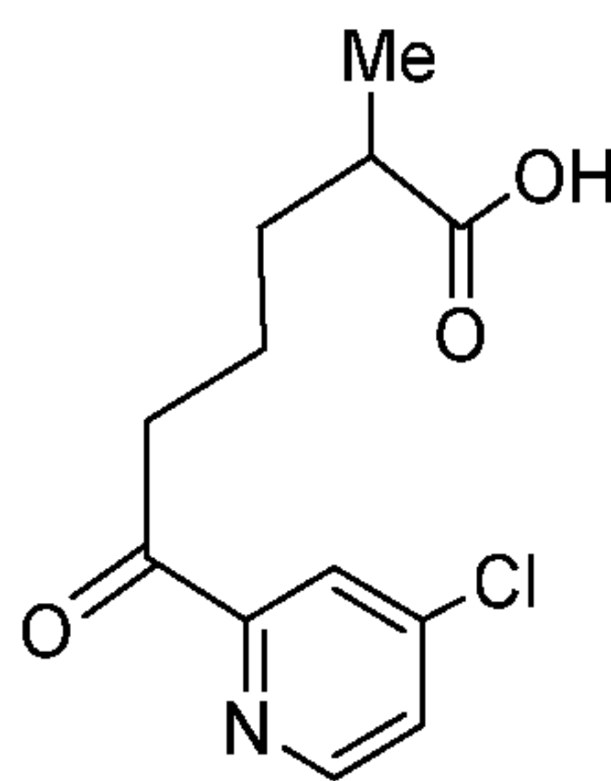
Compound 34.
