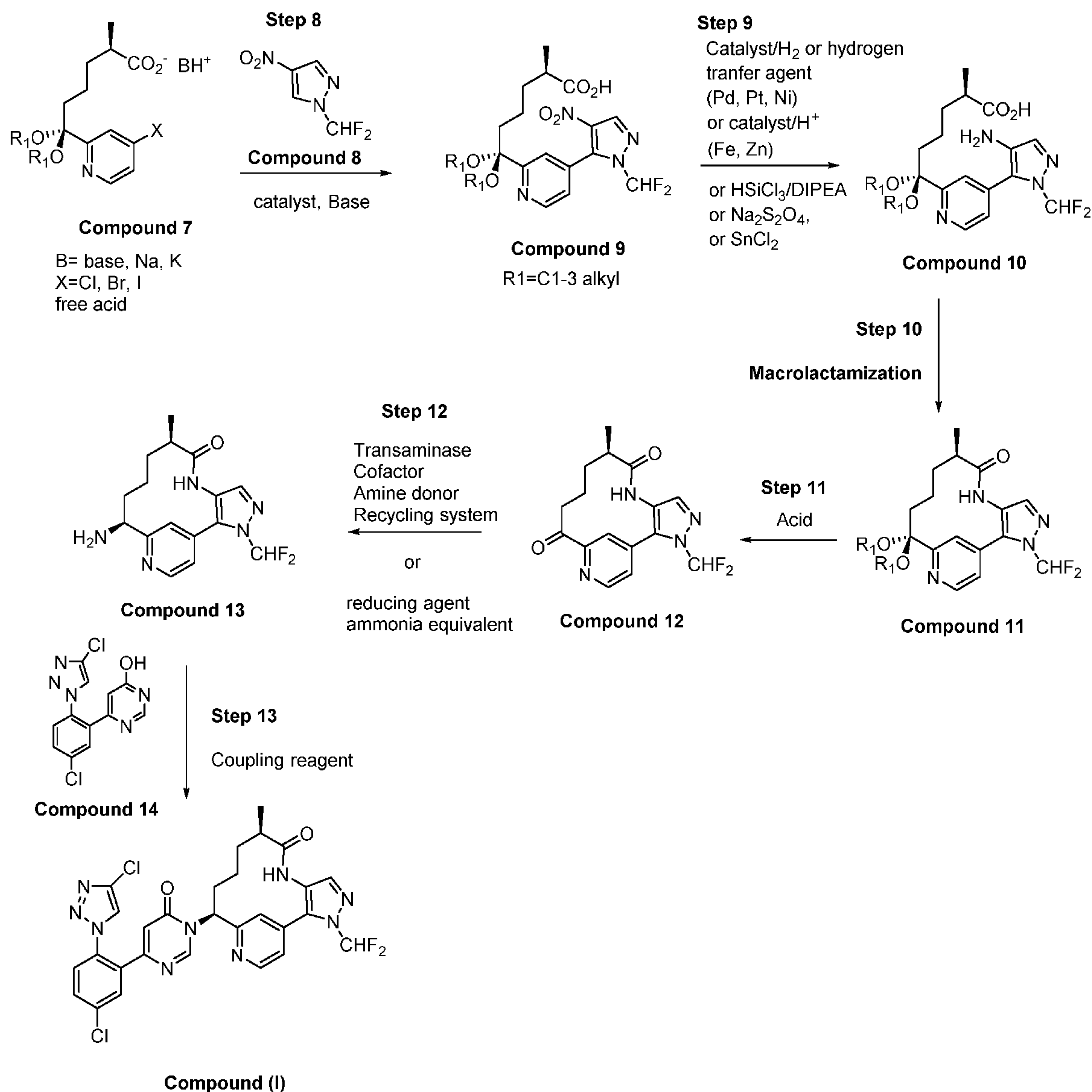
Scheme 2
