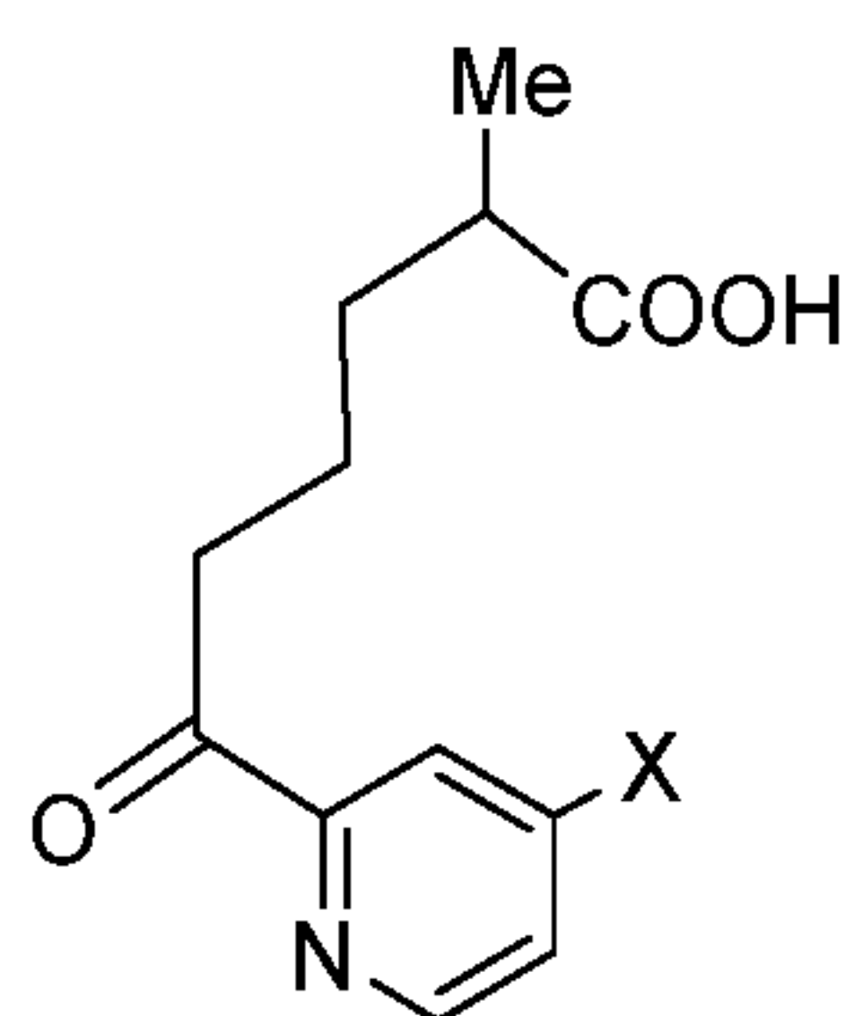
Compound 24
