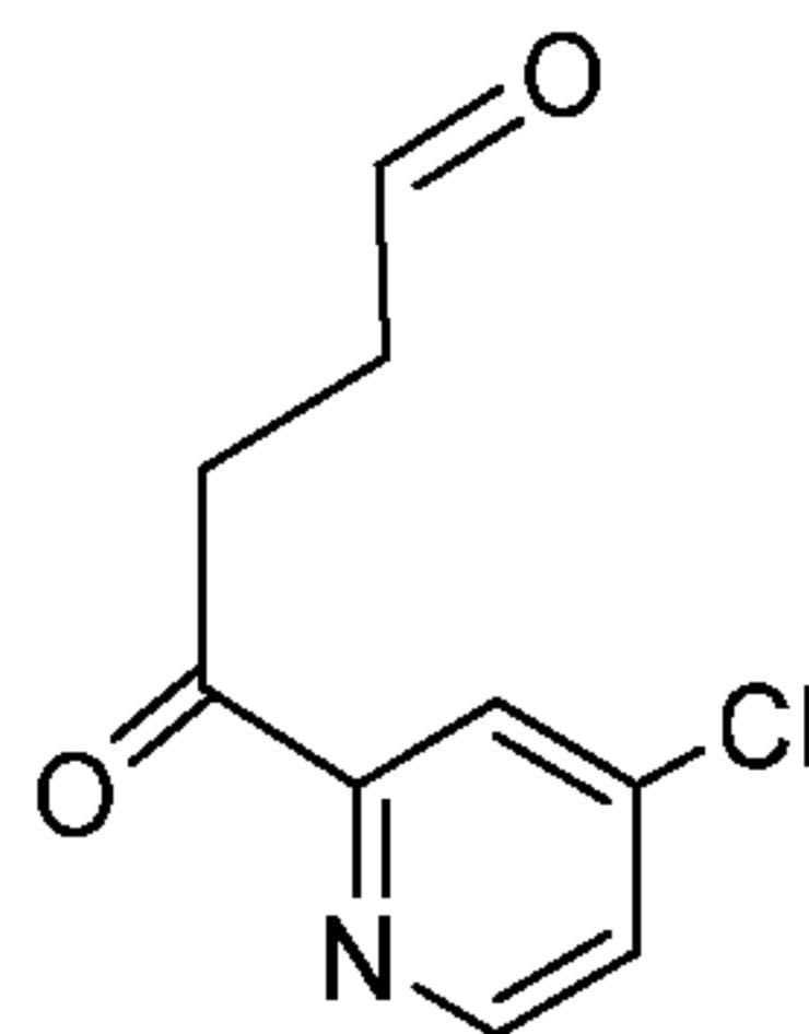
Compound 17
