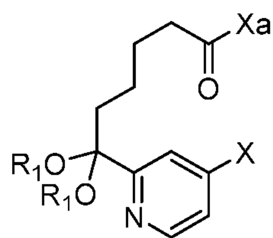
Compound 6a
