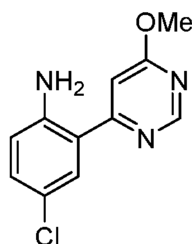
Compound 45;
