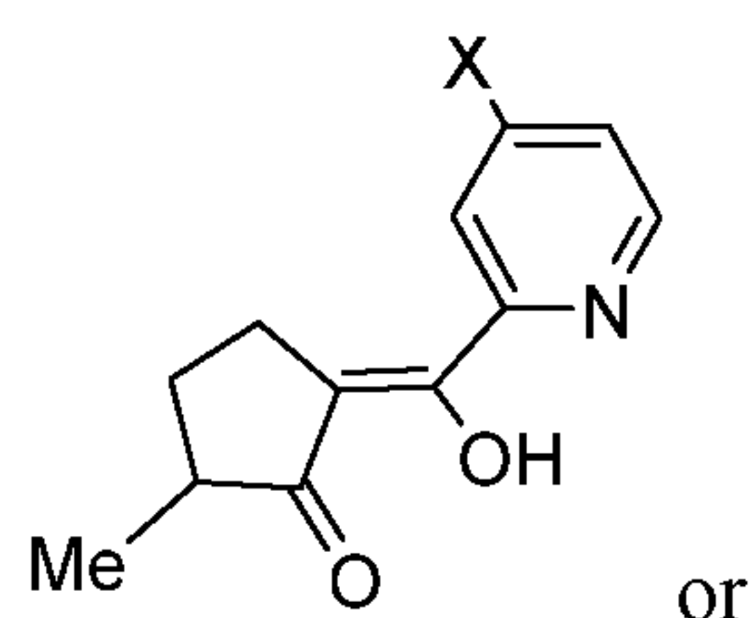
Compound 23a
