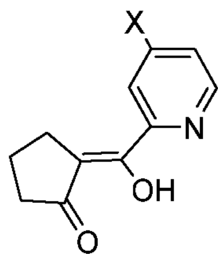
Compound 3a
