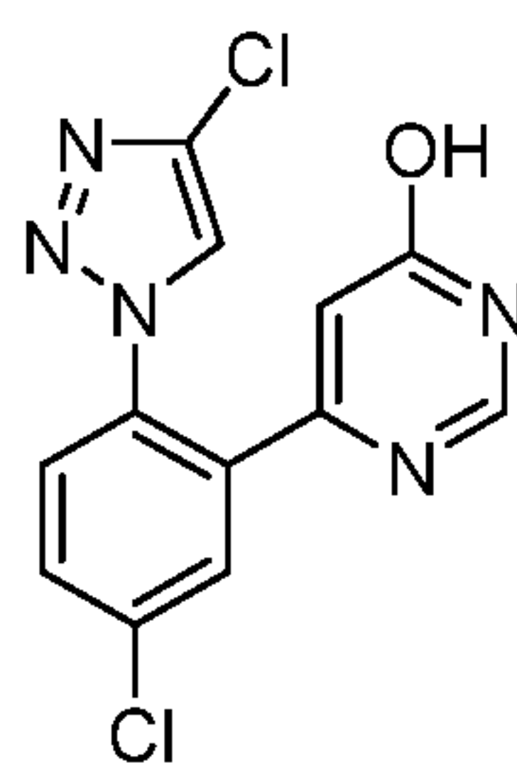
Compound 14
