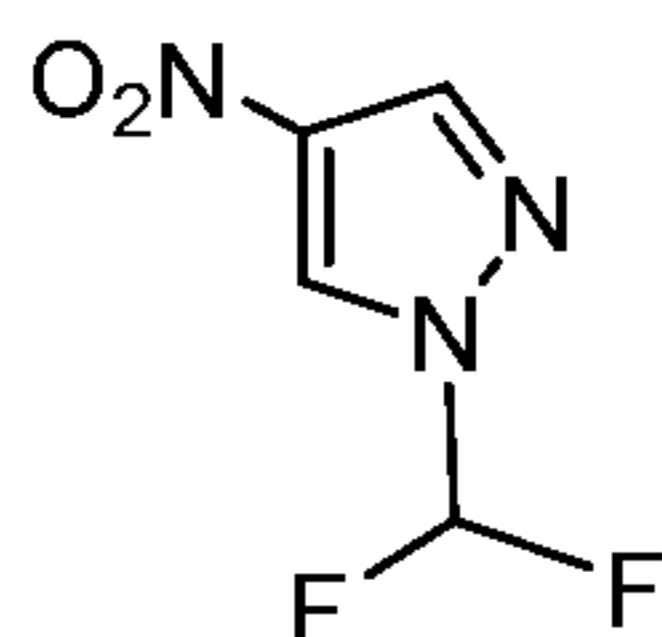
Compound 8
