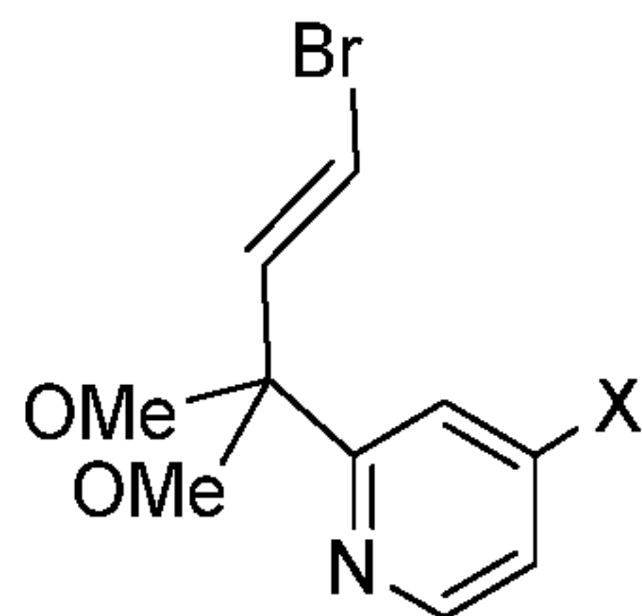
Compound 31
