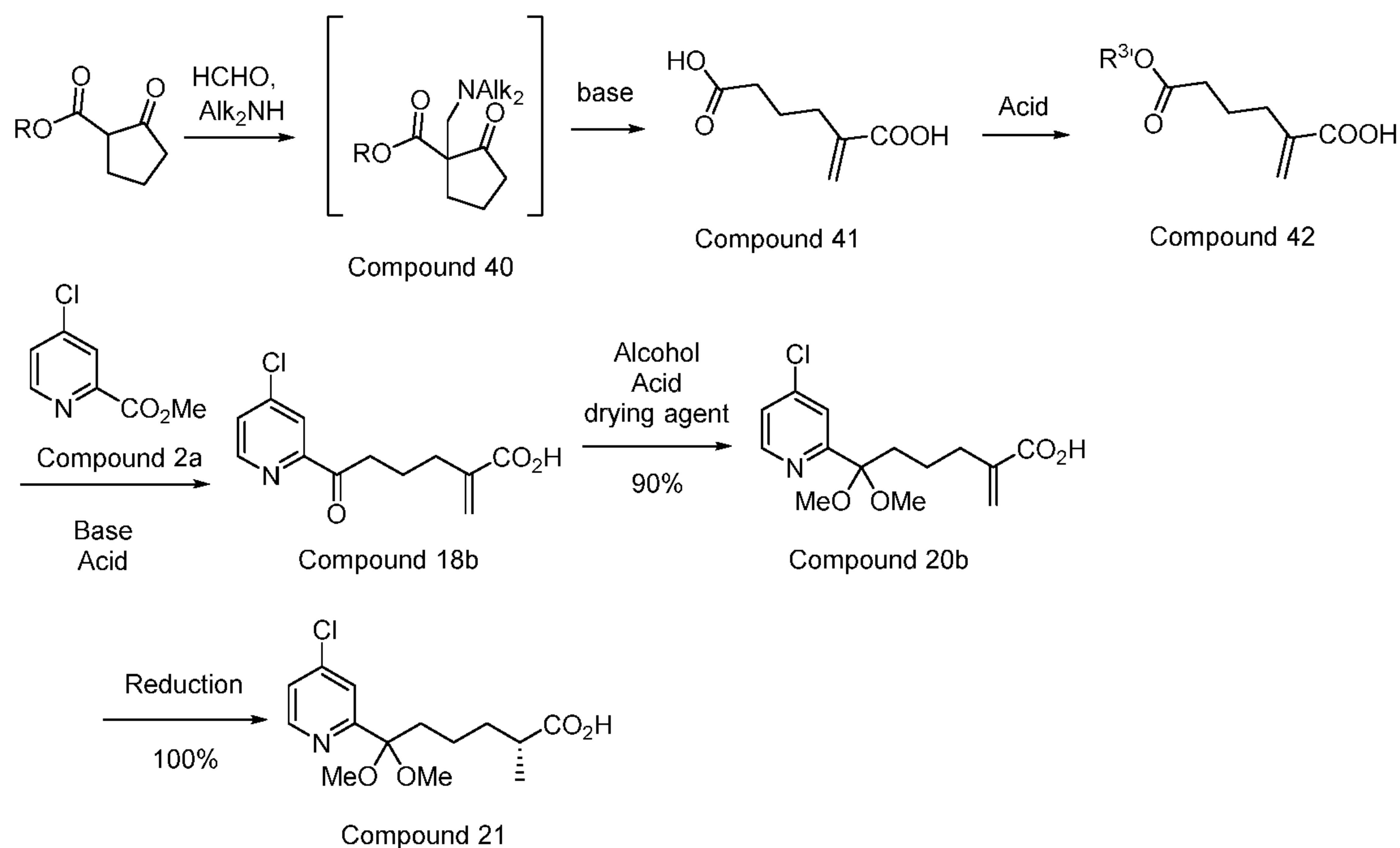
Scheme 5
