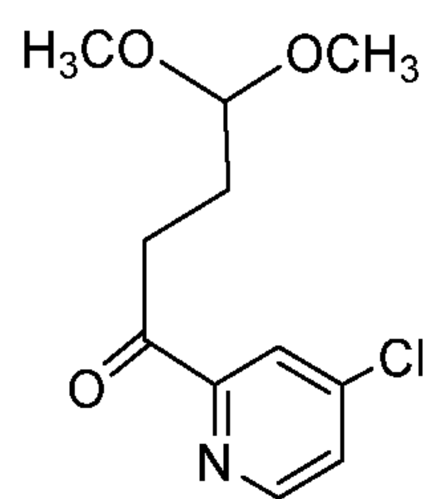
Compound 16
