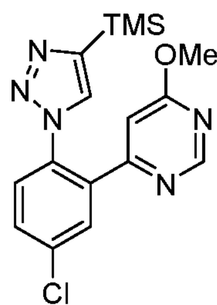
Compound 46;
