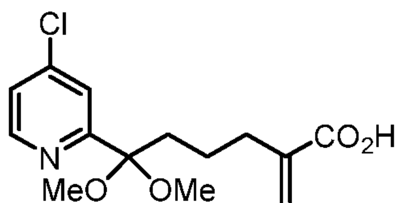
Compound 20b;
