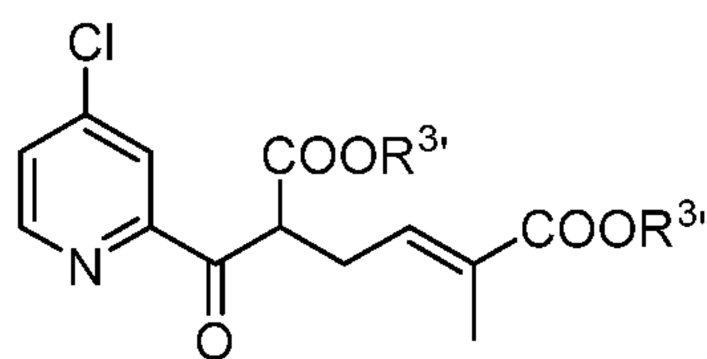
Compound 39;
