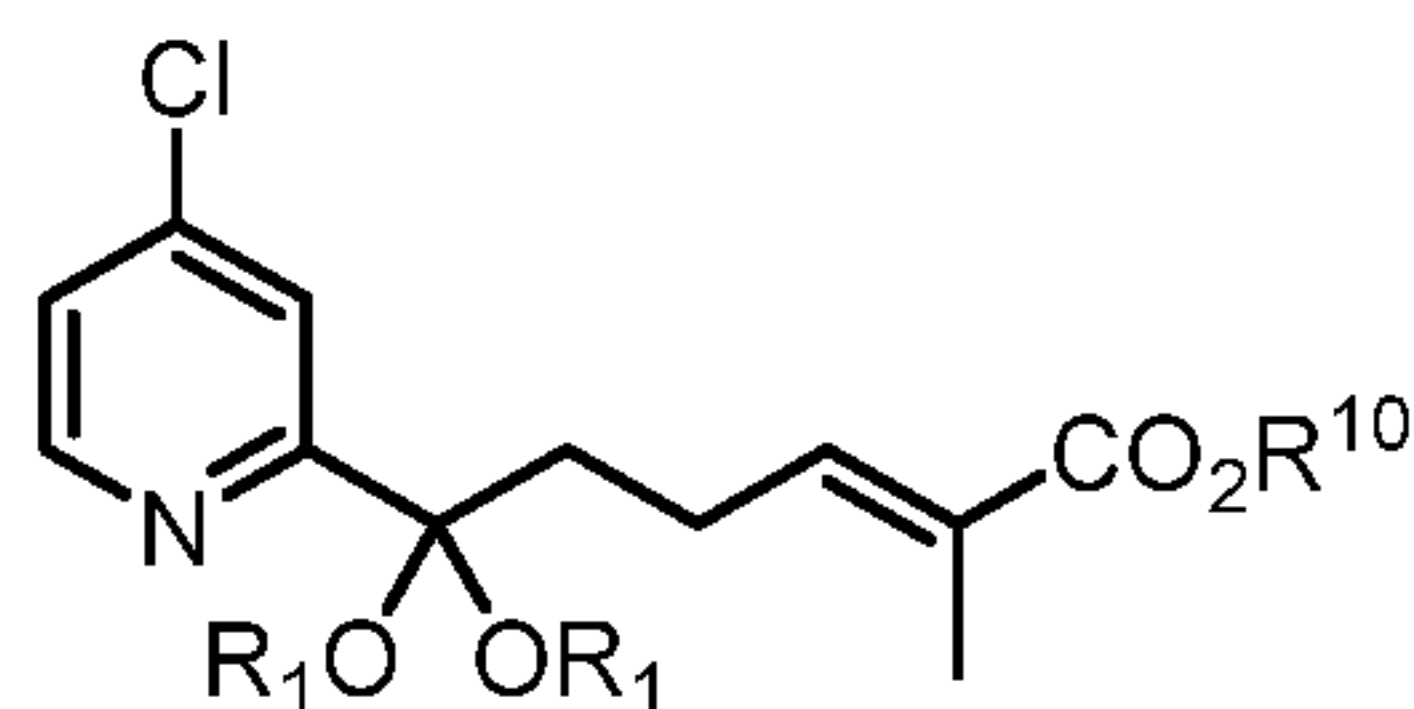
Compound 19
