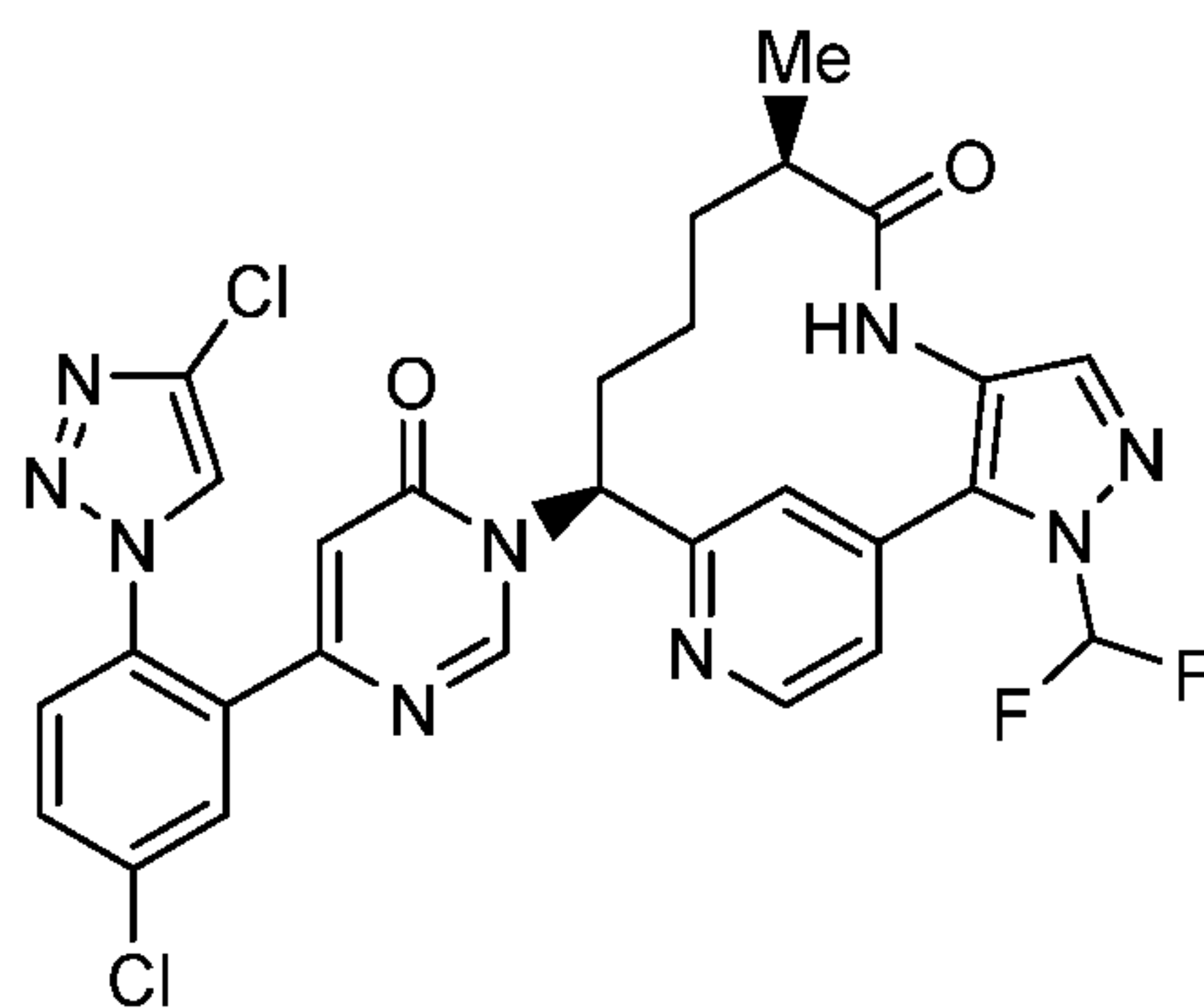
(I)
