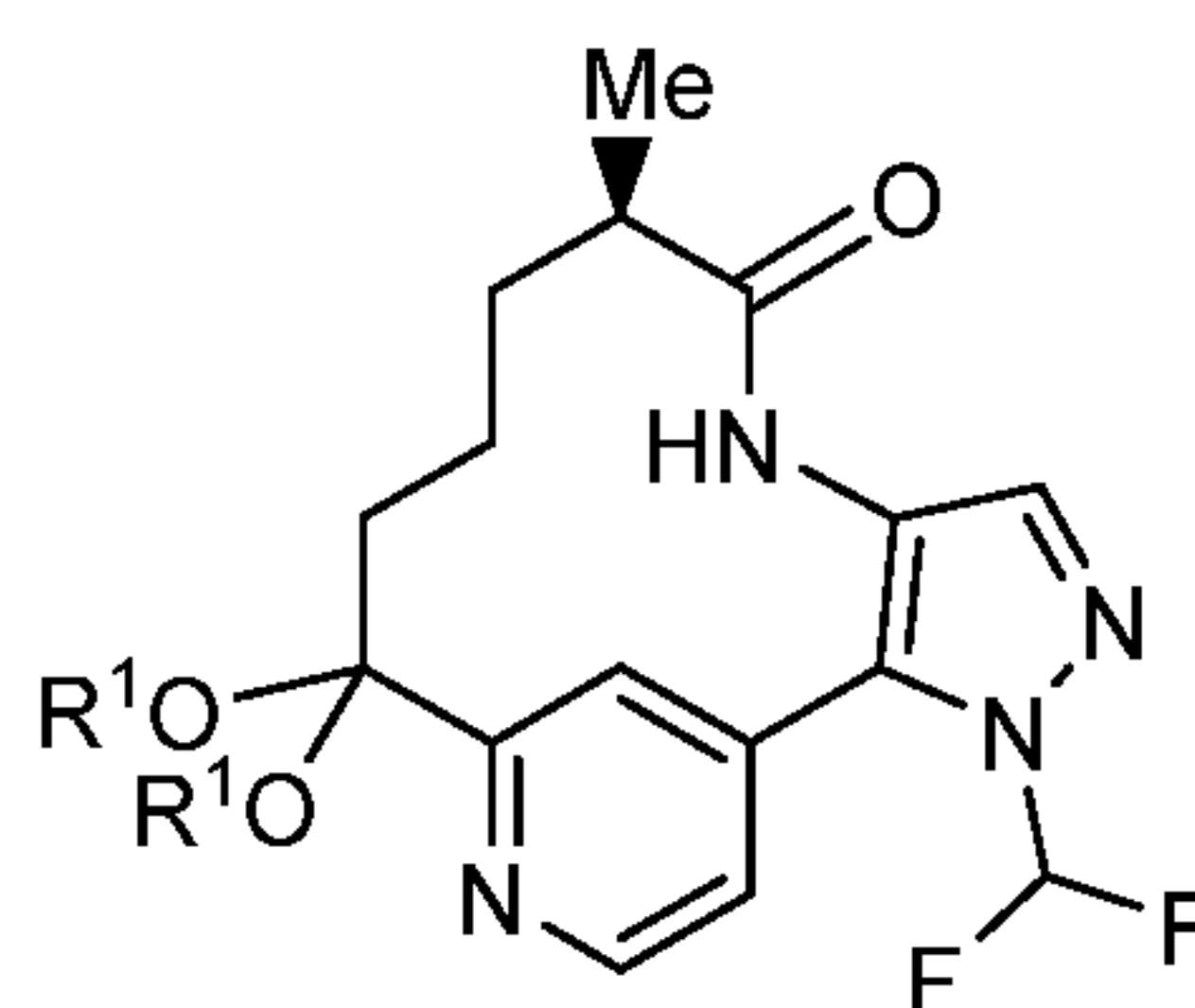
Compound 11
