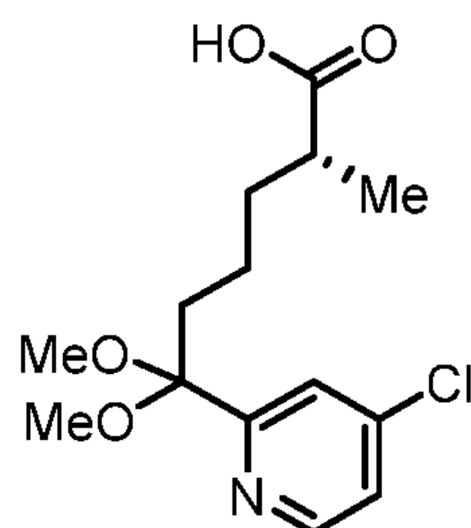
Compound 21.
