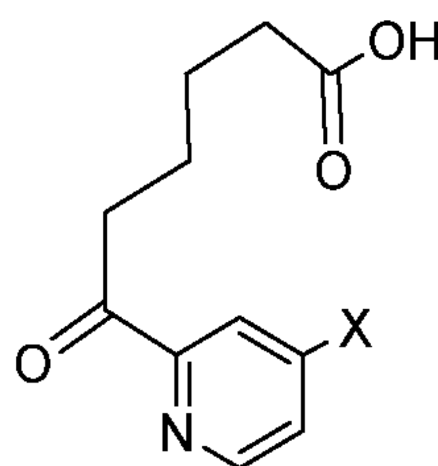
Compound 4;
