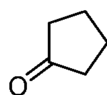
Compound 1
