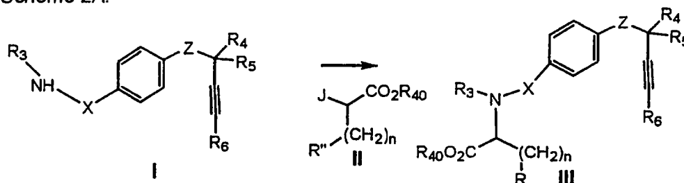
Scheme 2A:
