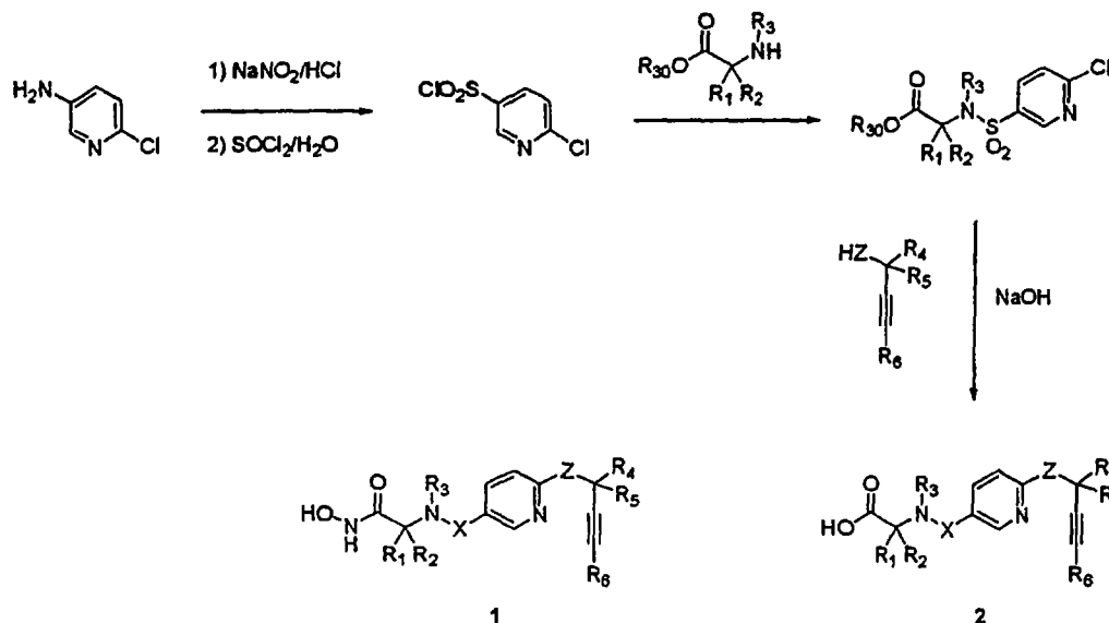
Scheme 2B:
