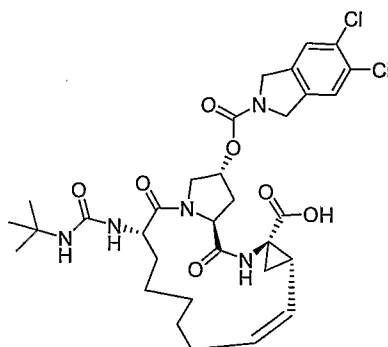
Compound AR00320450
