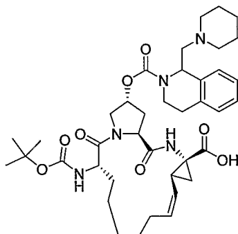
Compound AR00301383
