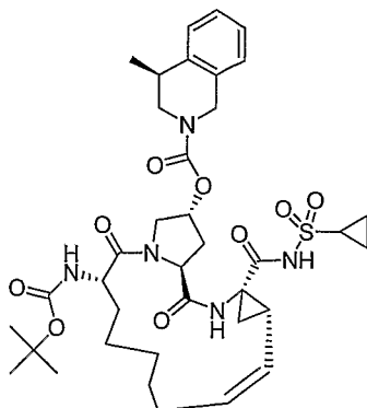
Compound AR00333463
