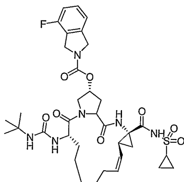
Compound AR00338066
