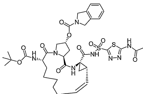
Compound AR00334247
