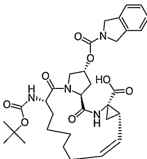
Compound AR00291871
