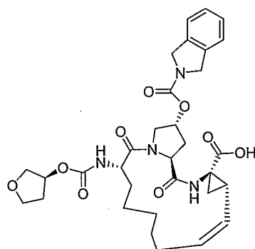
Compound AR00320075
