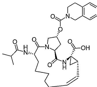
Compound AR00248688
