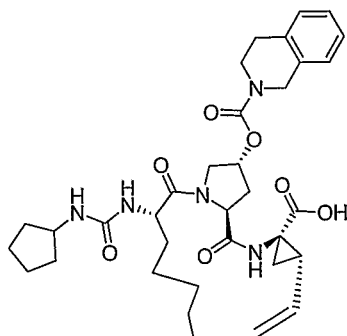
Compound AR00294378
