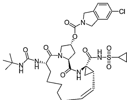
Compound AR00320446
