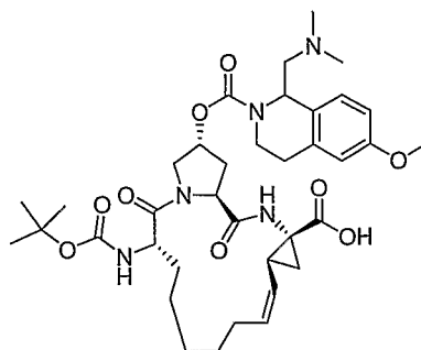
Compound AR00333277
