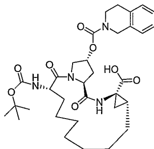
Compound AR00312023
