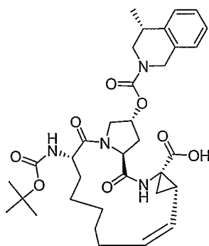
Compound AR00320122
