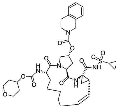
Compound AR00320082
