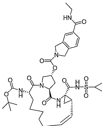
Compound AR00365252
