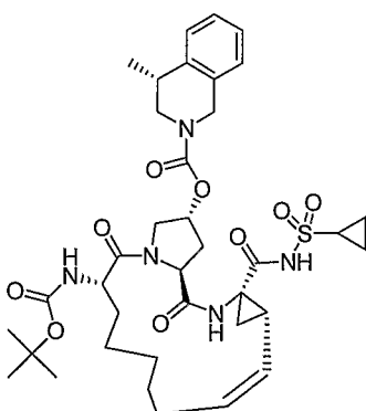
Compound AR00333462
