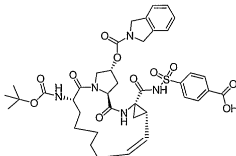
Compound AR00365387
