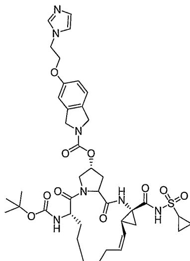
Compound AR00345096
