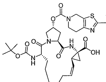
Compound AR00304158
