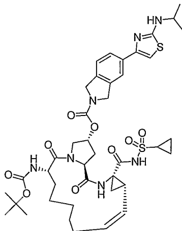
Compound AR00365019
