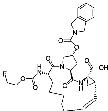
Compound AR00320076
