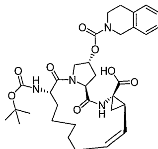
Compound AR00220122
