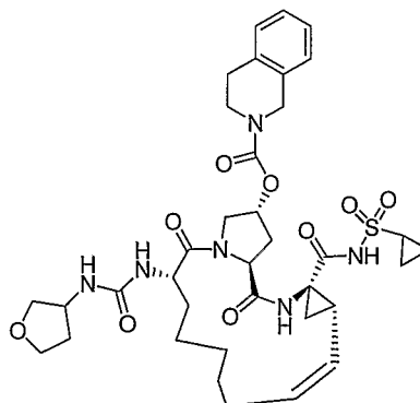
Compound AR00320222
