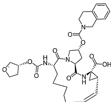
Compound AR00304127
