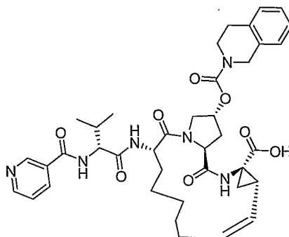
Compound AR00304073
