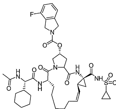
Compound AR00340122
