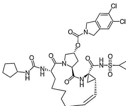
Compound AR00320575
