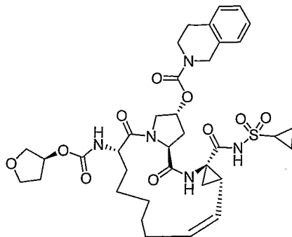
Compound AR00304162
