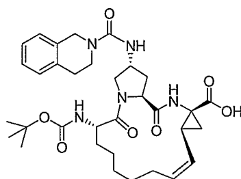
Compound AR00287262
