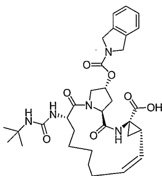
Compound AR00320078
