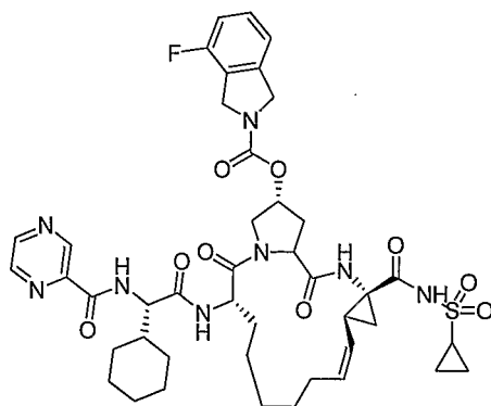
Compound AR00340303
