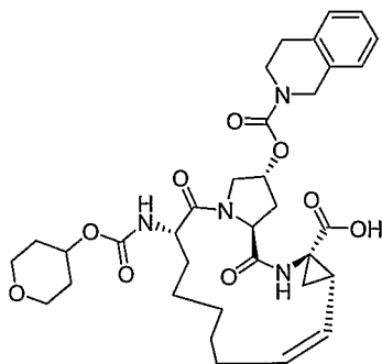
Compound AR00320002
