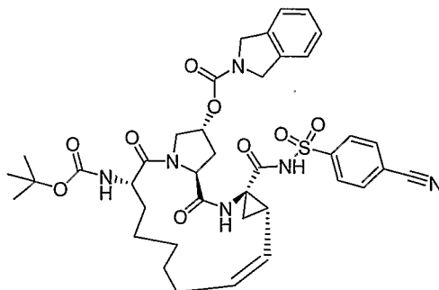
Compound AR00334248
