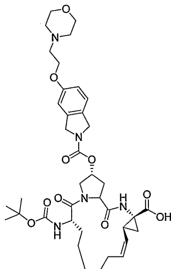
Compound AR00371946
