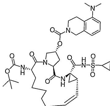
Compound AR00320120
