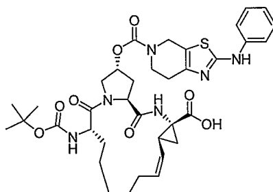
Compound AR00304000
