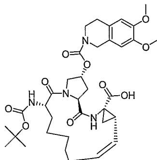
Compound AR00226824
