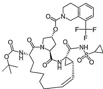
Compound AR00298997
