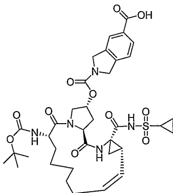
Compound AR00365084
