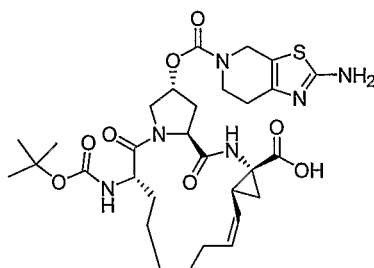
Compound AR00304154
