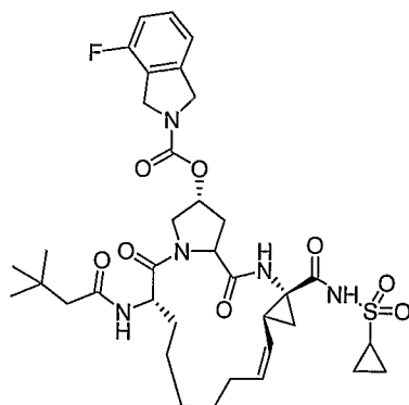
Compound AR00338070
