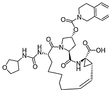
Compound AR00320221
