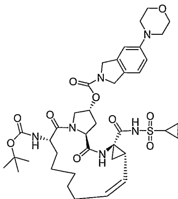
Compound AR00340494
