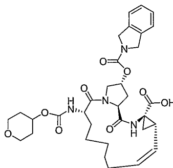
Compound AR00320077
