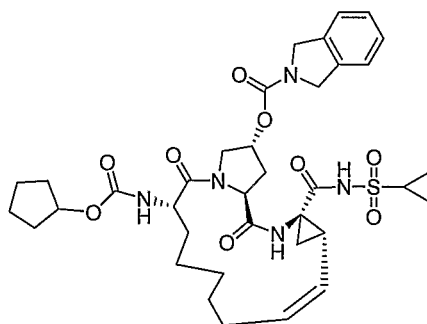
Compound AR00333831
