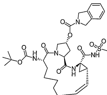
Compound AR00333803
