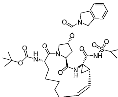
Compound AR00333801
