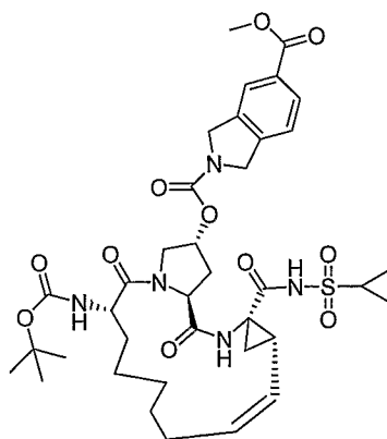
Compound AR00365083
