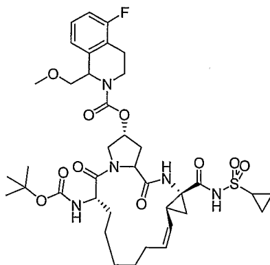
Compound AR00365193
