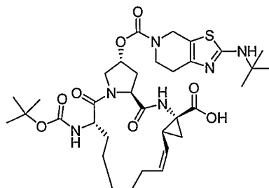
Compound AR00304103
