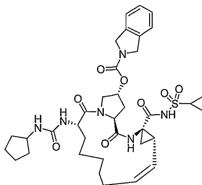
Compound AR00304082
