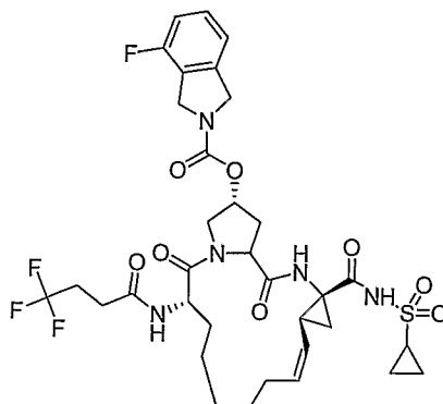
Compound AR00338071
