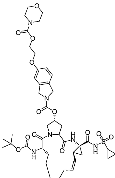
Compound AR00345032
