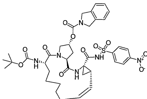
Compound AR00334249
