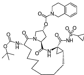
Compound AR00314719
