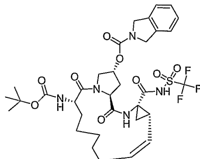
Compound AR00340479
