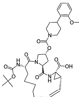
Compound AR00320576
