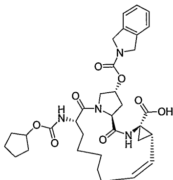
Compound AR00304076
