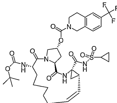
Compound AR00301747
