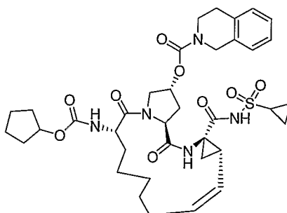
Compound AR00282131
