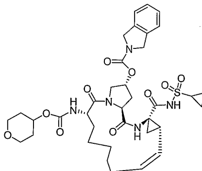
Compound AR00320081
