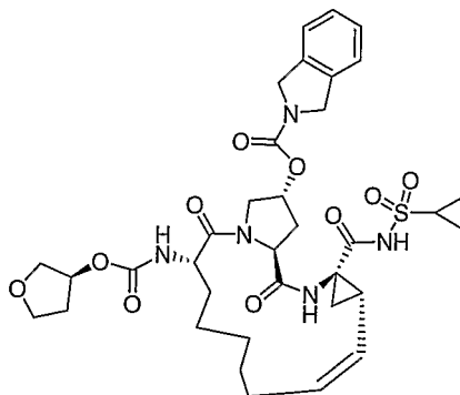
Compound AR00320080
