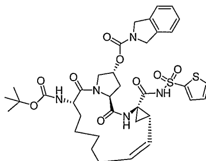
Compound AR00365427
