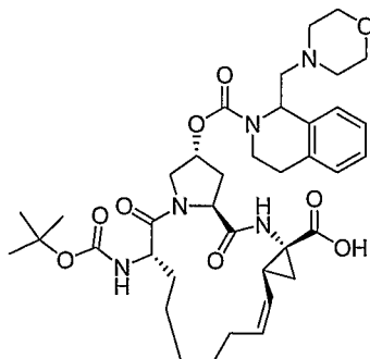
Compound AR00333225
