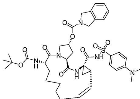
Compound AR00365572
