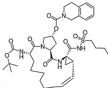
Compound AR00261409
