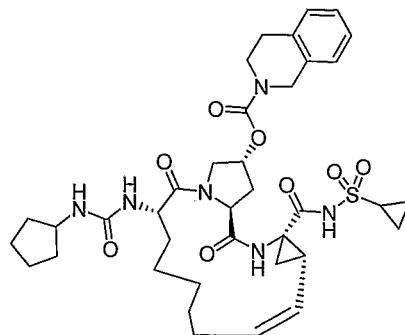
Compound AR00320403
