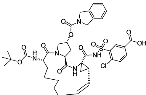
Compound AR00365388
