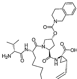
Compound AR00298990
