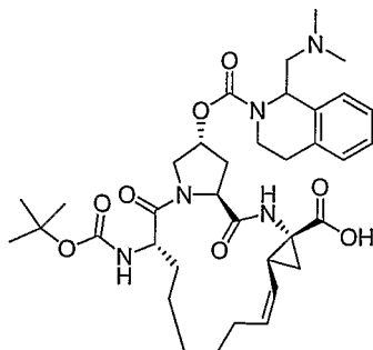
Compound AR00333224
