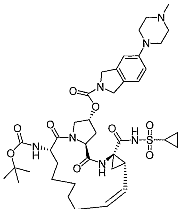
Compound AR00340495
