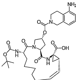
Compound AR00301745
