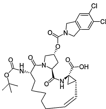
Compound AR00315999
