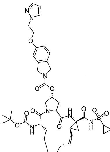
Compound AR00364924
