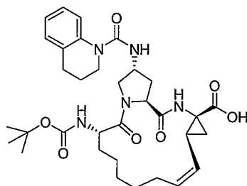
Compound AR00304160
