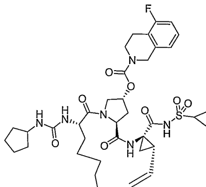
Compound AR00304080
