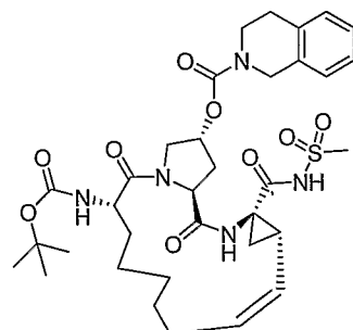
Compound AR00254906
