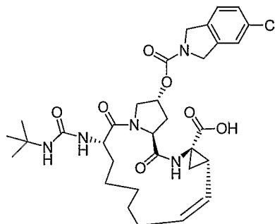
Compound AR00320449
