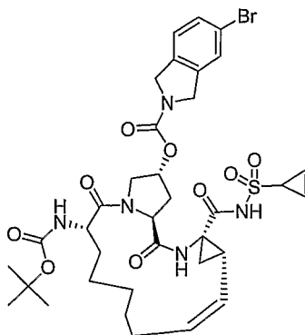
Compound AR00340526
