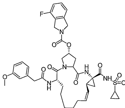
Compound AR00340178
