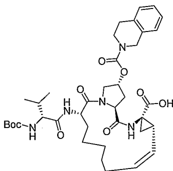
Compound AR00298989
