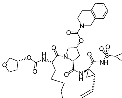
Compound AR00304163
