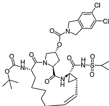
Compound AR00320121
