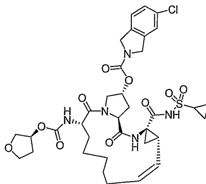
Compound AR00334220
