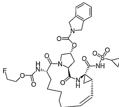
Compound AR00320073
