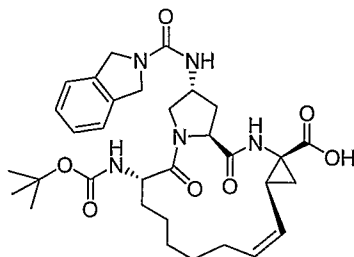
Compound AR00298980
