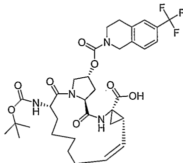
Compound AR00294383
