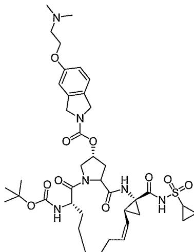
Compound AR00345095
