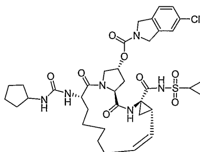
Compound AR00320574
