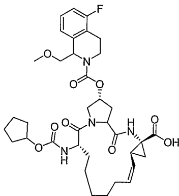
Compound AR00365381
