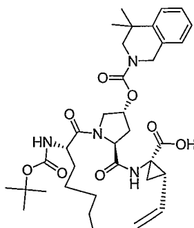
Compound AR00304066
