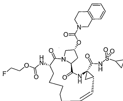
Compound AR00304161
