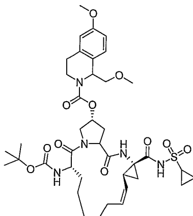
Compound AR00334339
