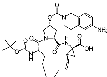
Compound AR00314578
