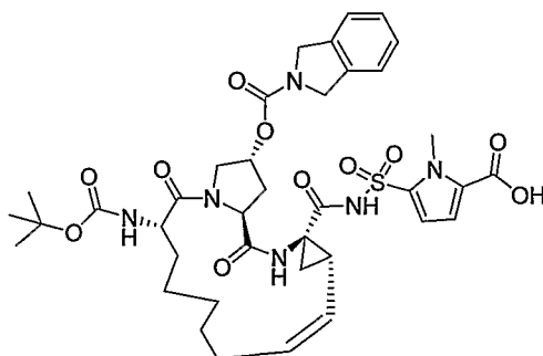
Compound AR00364266
