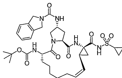
Compound AR00304008
