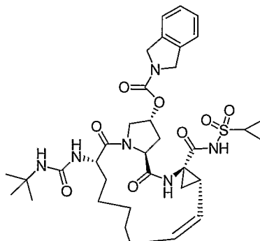
Compound AR00320220
