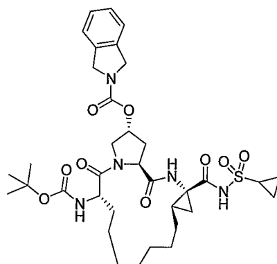
Compound AR00333833
