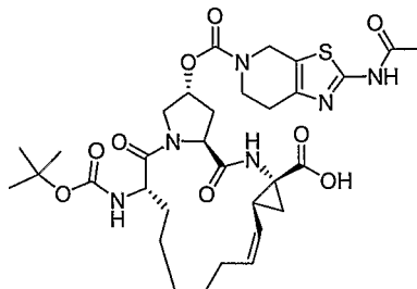
Compound AR00314685
