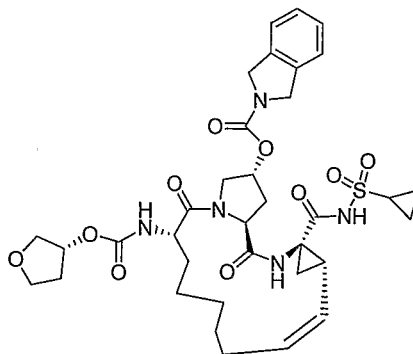
Compound AR00320079
