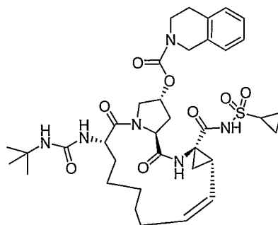
Compound AR00320001
