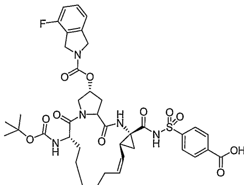
Compound AR00365438
