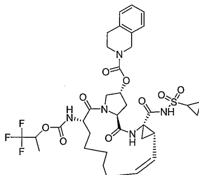
Compound AR00320581
