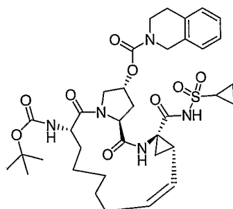
Compound AR00261408
