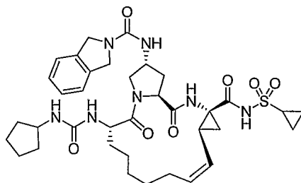
Compound AR00304014
