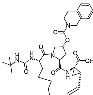
Compound AR00294377
