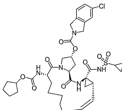
Compound AR00334218
