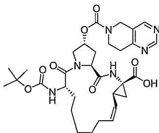
Compound AR00304183
