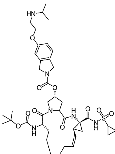
Compound AR00345094
