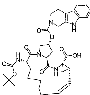
Compound AR00226825
