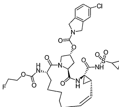
Compound AR00334222
