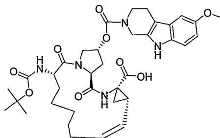
Compound AR00320577
