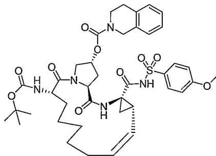
Compound AR00320548
