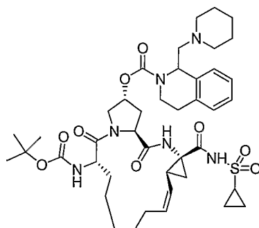
Compound AR00311815
