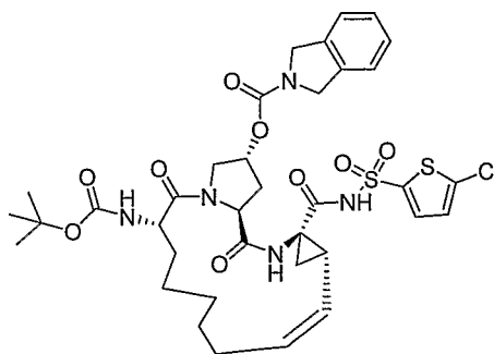
Compound AR00334188
