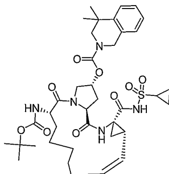
Compound AR00312025
