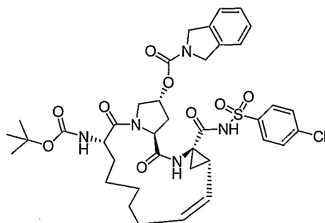
Compound AR00334250
