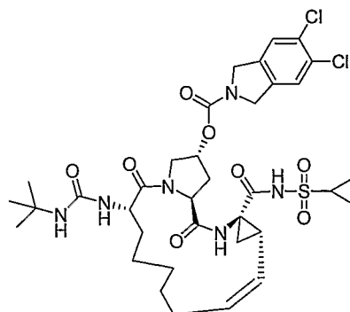
Compound AR00320447
