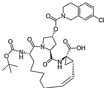
Compound AR00304062
