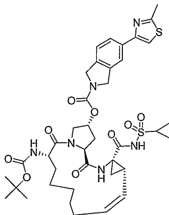
Compound AR00364989
