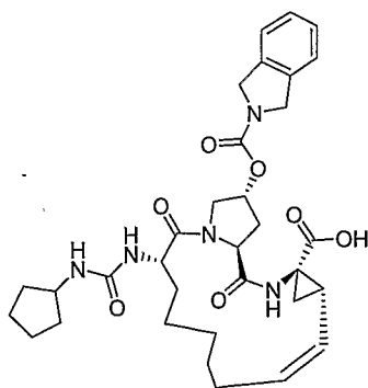
Compound AR00304079
