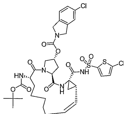
Compound AR00340173
