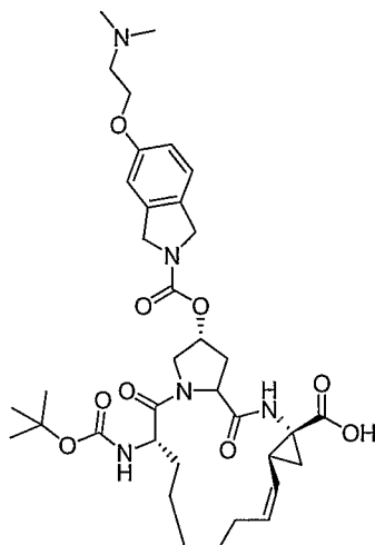
Compound AR00371947
