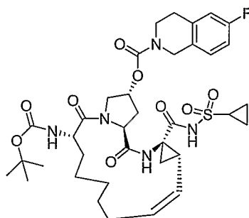
Compound AR00301751
