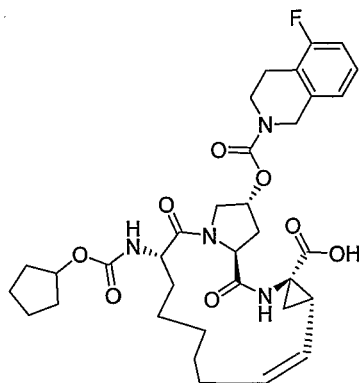
Compound AR00304074
