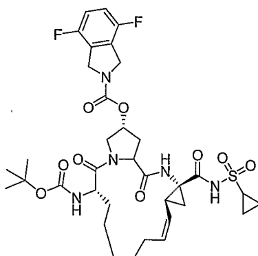
Compound AR00334399
