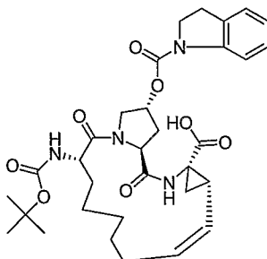
Compound AR00291875
