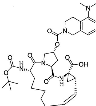
Compound AR00315997
