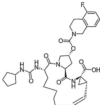
Compound AR00304077
