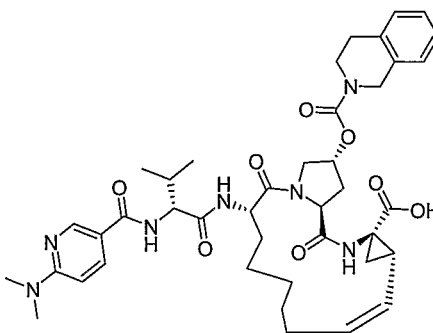
Compound AR00304072
