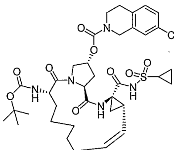
Compound AR00301746
