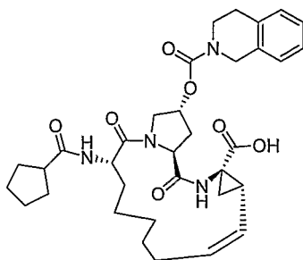
AR00248689
