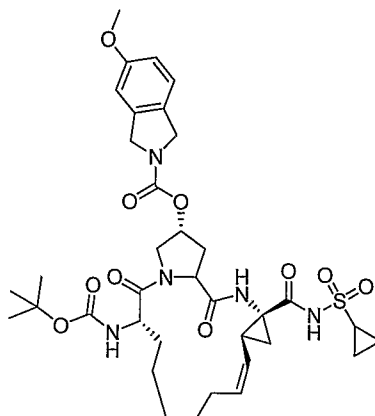
Compound AR00334314
