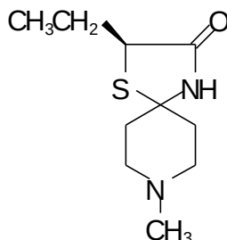
Compound A
