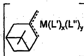
Structure VIb
