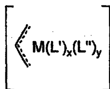
Structure VIa
