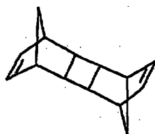
Norbornadiene Dimer exo-trans-exo (2+2 dimer)
