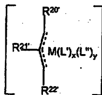
Structure VI
