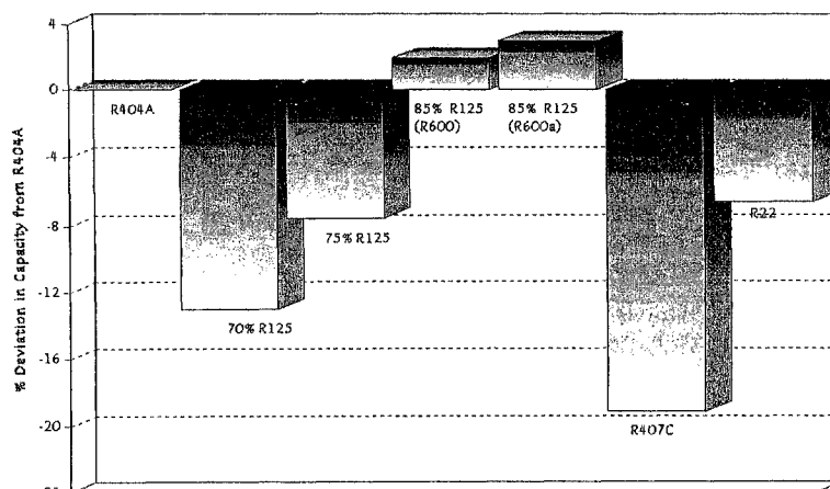
Graph 1 PERCENTAGE DEVIATION IN CAPACITY FROM R404A FOR R22, R407C AND THE HIGH R125 CONTAINING BLENDS BASED ON A MEAN EVAPORATING TEMPERATURE OF -30°C
