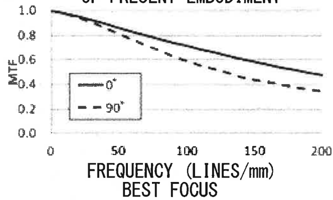
FIG. 6B TORIC INTRAOCULAR LENS OF PRESENT EMBODIMENT
