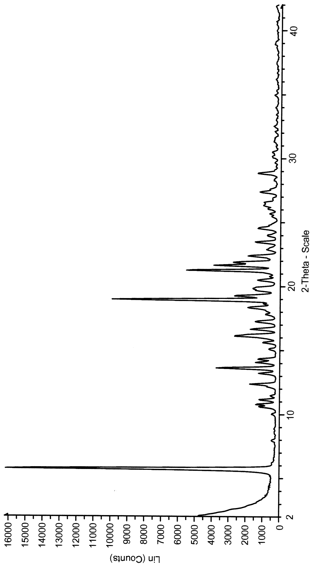
FIG. 1 XRPD Pattern of Form A
