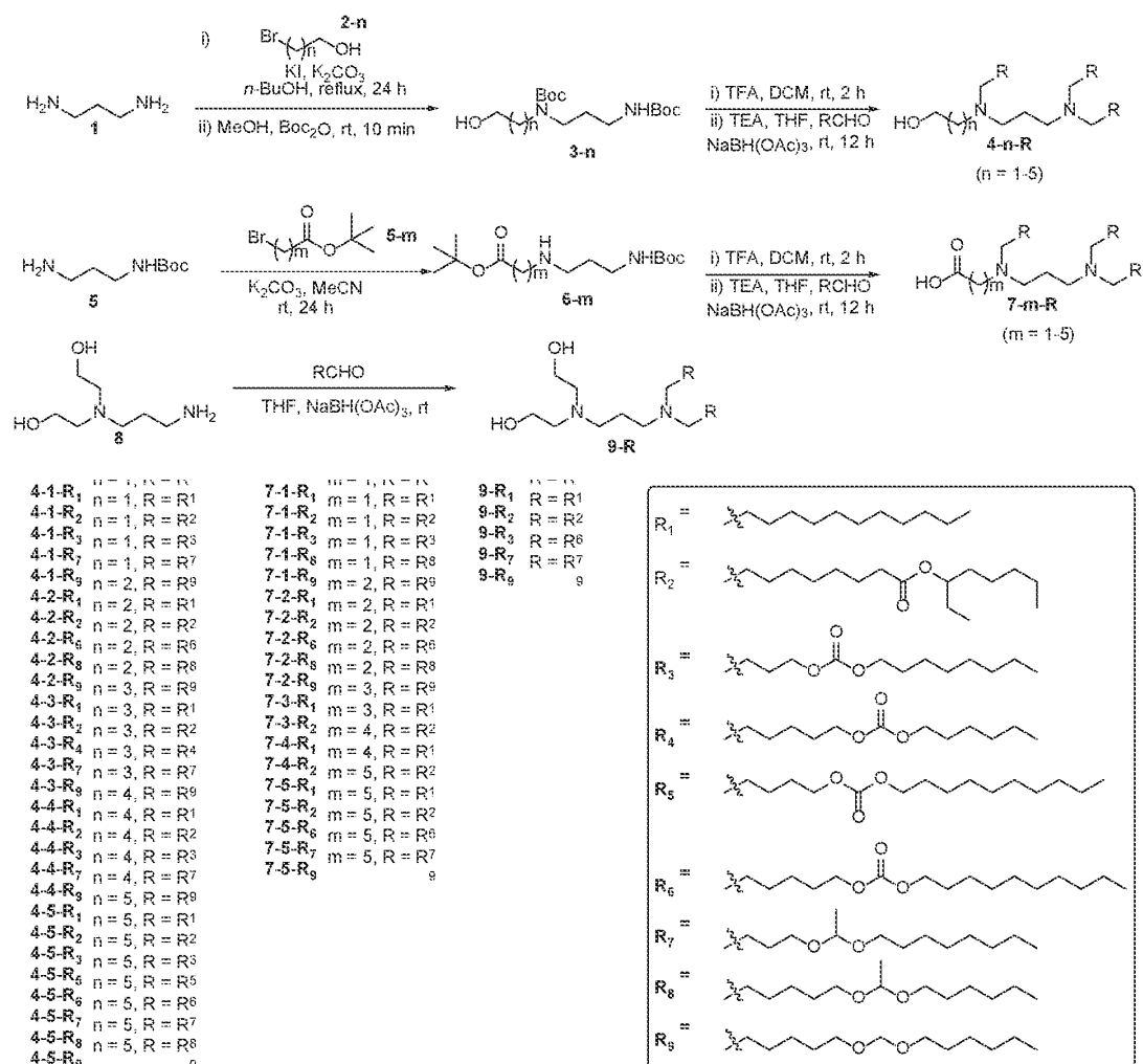
Scheme 1. General synthetic route of amino alcohol lipids and amino acid lipids
