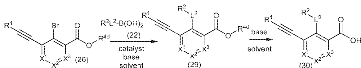
Scheme 6.
