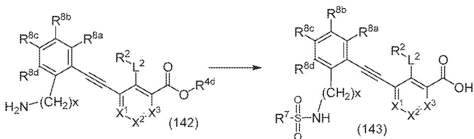
Scheme 37.
