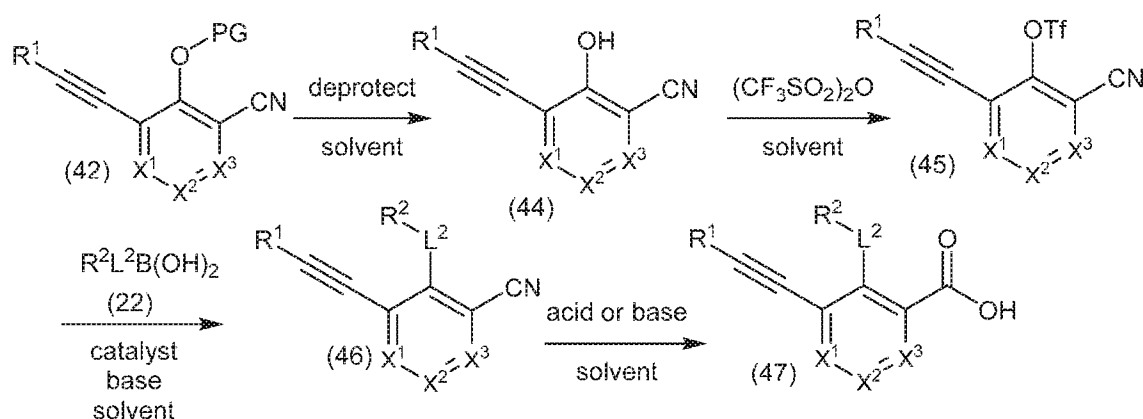
Scheme 10.
