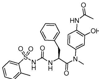
(S)-N-(4-acetamido-3-hydroxyphenyl)-N-methyl-3-phenyl-2-(3-(o-tolylsulfonyl)ureido)propanamide
