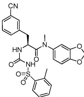
(S)-N-(benzo[d][1,3]dioxol-5-yl)-3-(3-cyanophenyl)-N-methyl-2-(3-(o-tolylsulfonyl)ureido)propanamide
