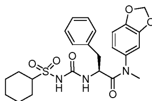
(S)-N-(benzo[d][1,3]dioxol-5-yl)-2-(3-(cyclohexylsulfonyl)ureido)-N-methyl-3-phenylpropanamide
