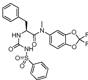
(S)-N-(2,2-difluorobenzo[d][1,3]dioxol-5-yl)-N-methyl-3-phenyl-2-(3-phenylsulfonyl)ureido)propanamide
