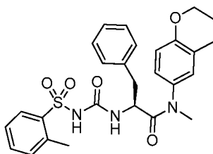
(S)-N-(chroman-6-yl)-N-methyl-3-phenyl-2-(3-(o-tolylsulfonyl)ureido)propanamide
