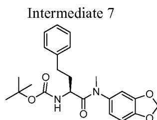
15 (S)-tert-butyl (1-(benzo[d][1,3]dioxol-5-yl(methyl)amino)-1-oxo-4-phenylbutan-2-yl)carbamate
