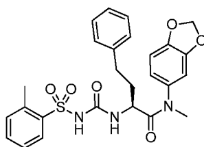
(S)-N-(benzo[d][1,3]dioxol-5-yl)-N-methyl-4-phenyl-2-(3-(o- 10 tolylsulfonyl)ureido)butanamide
