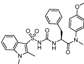
(S)-2-(3-((1,2-dimethyl-1H-indol-3-yl)sulfonyl)ureido)-N-(4-methoxyphenyl)-N-methyl-3-phenylpropanamide
