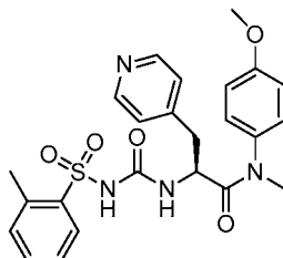
(S)-N-(4-methoxyphenyl)-N-methyl-3-(pyridin-4-yl)-2-(3-(o-tolylsulfonyl)ureido)propanamide
