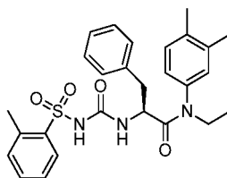
(S)-N-(3,4-dimethylphenyl)-N-ethyl-3-phenyl-2-(3-(o-tolylsulfonyl)ureido)propanamide
