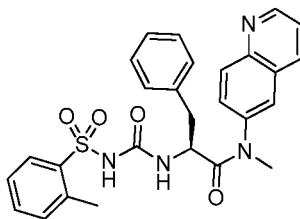
(S)-N-methyl-3-phenyl-N-(quinolin-6-yl)-2-(3-(o-tolylsulfonyl)ureido)propanamide
