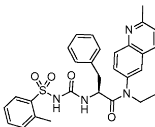
(S)-N-ethyl-N-(2-methylquinolin-6-yl)-3-phenyl-2-(3-(o-tolylsulfonyl)ureido)propanamide
