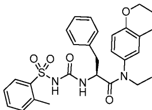
(S)-N-(chroman-6-yl)-N-ethyl-3-phenyl-2-(3-(o-tolylsulfonyl)ureido)propanamide
