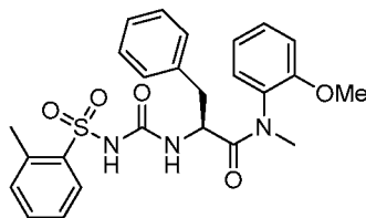
(S)-N-(2-methoxyphenyl)-N-methyl-3-phenyl-2-(3-(o-tolylsulfonyl)ureido)propanamide
