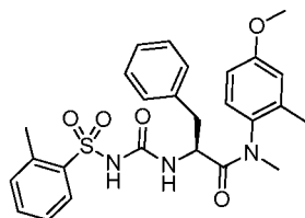
(S)-N-(4-methoxy-2-methylphenyl)-N-methyl-3-phenyl-2-(3-(o-tolylsulfonyl)ureido)propanamide
