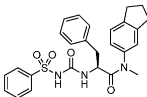
(S)-N-(2,3-dihydro-1H-inden-5-yl)-N-methyl-3-phenyl-2-(3-phenylsulfonyl)ureido)propanamide
