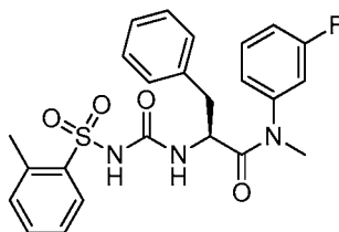
(S)-N-(3-fluorophenyl)-N-methyl-3-phenyl-2-(3-(o-tolylsulfonyl)ureido)propanamide
