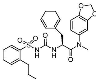
(S)-N-(benzo[d][1,3]dioxol-5-yl)-N-methyl-3-phenyl-2-(3-((2-propylphenyl)sulfonyl)ureido)propanamide
