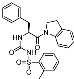
(S)-N-((1-(indolin-1-yl)-1-oxo-3-phenylpropan-2-yl)carbamoyl)-2-methylbenzenesulfonamide
