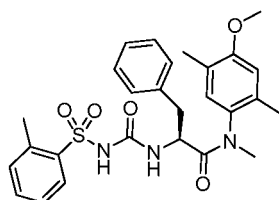
(S)-N-(4-methoxy-2,5-dimethylphenyl)-N-methyl-3-phenyl-2-(3-(o-tolylsulfonyl)ureido)propanamide
