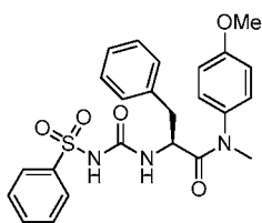
(S)-N-(4-methoxyphenyl)-N-methyl-3-phenyl-2(3-phenylsulfonylureido)propanamide
