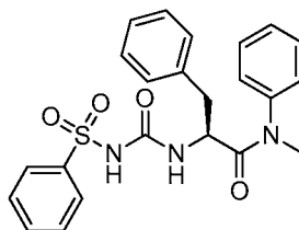
(S)-N-methyl-N,3-diphenyl-2-(3-(phenylsulfonyl)ureido)propanamide
