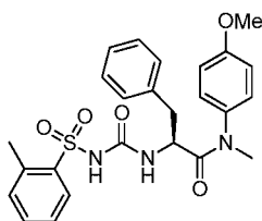
(S)-N-(4-methoxyphenyl)-N-methyl-3-phenyl-2-(3-(o-tolylsulfonyl)ureido)propanamide
