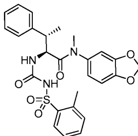
(2S,3S)-N-(benzo[d][1,3]dioxol-5-yl)-N-methyl-3-phenyl-2-(3-(o-tolylsulfonyl)ureido)butanamide
