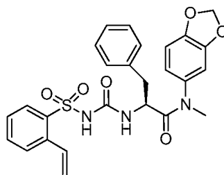
(S)-N-(benzo[d][1,3]dioxol-5-yl)-N-methyl-3-phenyl-2-(3-((2-vinylphenyl)sulfonyl)ureido)propanamide
