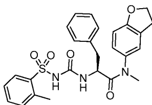
(S)-N-(2,3-dihydrobenzofuran-5-yl)-N-methyl-3-phenyl-2-(3-(o-tolylsulfonyl)ureido)propanamide
