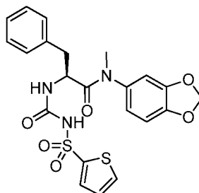
(S)-N-(benzo[d][1,3]dioxol-5-yl)-N-methyl-3-phenyl-2-(3-(thiophen-2-ylsulfonyl)ureido)propanamide
