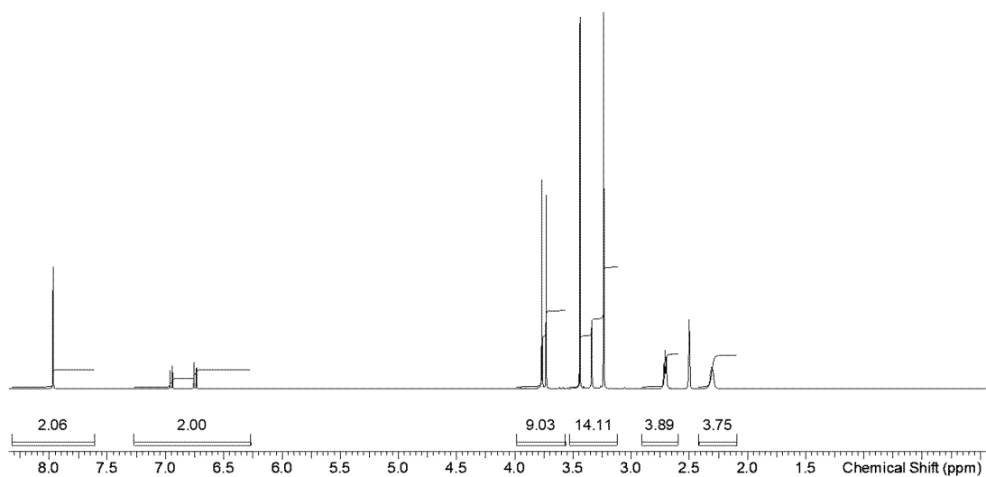
Figure 1 – ^1\text{H} NMR spectrum of the trimetazidine theophylline 1/2 complex obtained in Example 1
