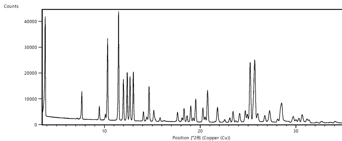
Figure 2 – XRPD pattern of the trimetazidine theophylline 1/2 complex obtained in Example
