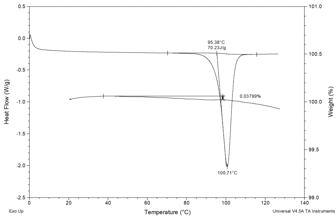
Figure 3 – DSC and TG graphs of the trimetazidine theophylline 1/2 complex obtained in Example 1
