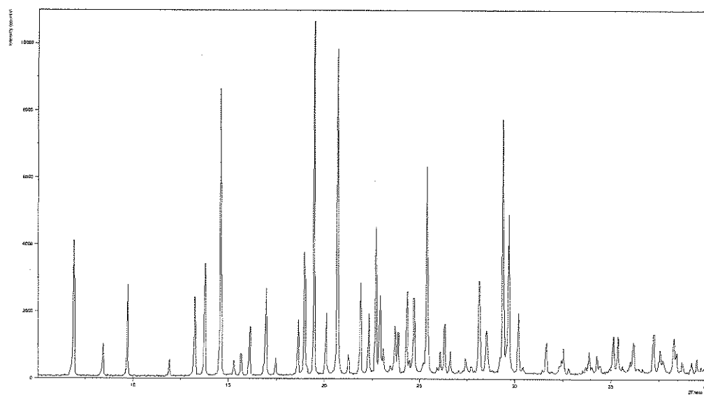
XRPD of 1-[2-(2,4-dimethylphenylsulfanyl)phenyl]piperazine, HBr, \beta -form
