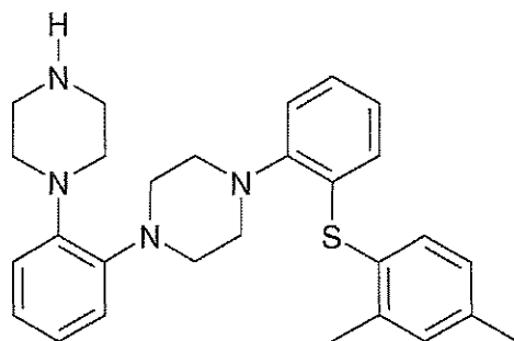
1-[2-(2,4-dimethyl-phenylsulfanyl)-phenyl]-4-(2-piperazin-1-yl-phenyl)-piperazine
