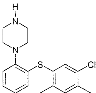
1-[2-(5-chloro-2,4-dimethyl-phenylsulfanyl)phenyl]piperazine
