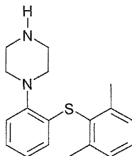
1-[2-(2,6-dimethylphenylsulfanyl)phenyl]piperazine
