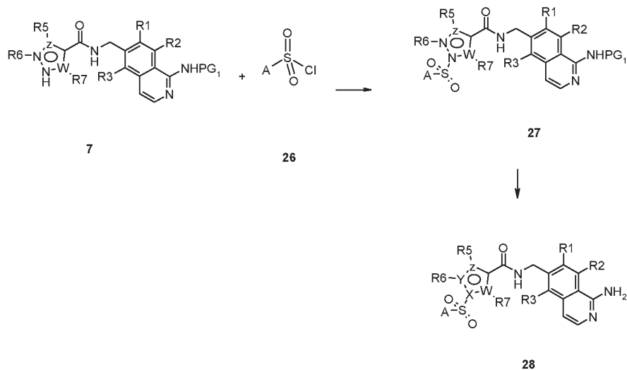
Scheme 7
