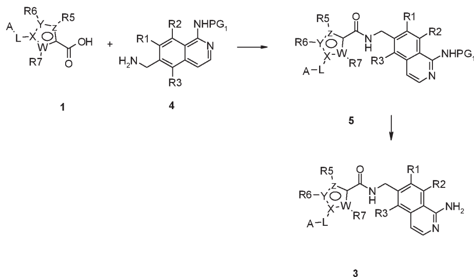
Scheme 2
