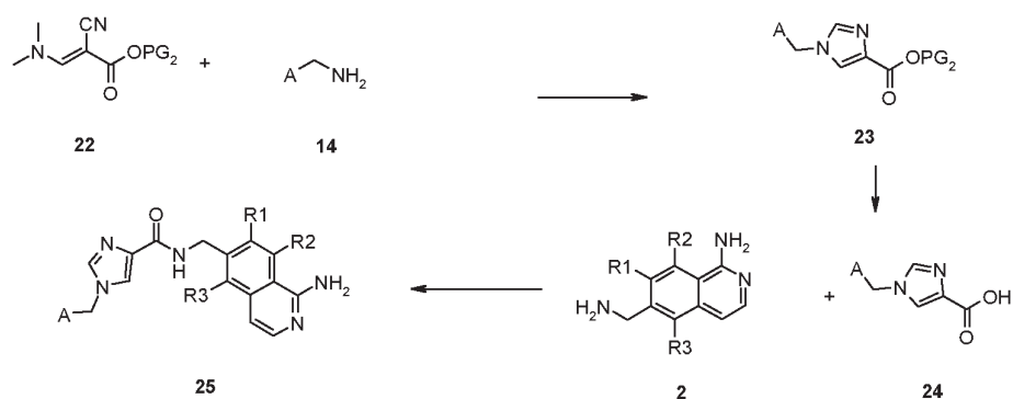
Scheme 6
