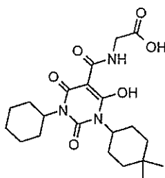
N -{[3-Cyclohexyl-1-(4,4-dimethylcyclohexyl)-6-hydroxy-2,4-dioxo-1,2,3,4-tetrahydro-5-pyrimidinyl]carbonyl}glycine
