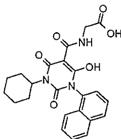
N -{[3-Cyclohexyl-6-hydroxy-1-(1-naphthalenyl)-2,4-dioxo-1,2,3,4-tetrahydro-5-pyrimidinyl]carbonyl}glycine
