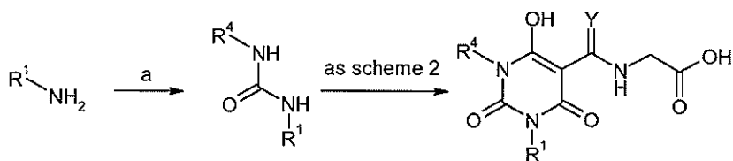
Scheme 3 (for R^1 = R^4 )
