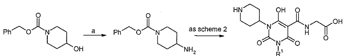
Scheme 6
