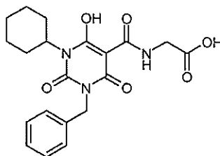
N -{[1-Cyclohexyl-6-hydroxy-2,4-dioxo-3-(phenylmethyl)-1,2,3,4-tetrahydro-5-pyrimidinyl]carbonyl}glycine
