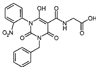
N -{[6-Hydroxy-1-(2-nitrophenyl)-2,4-dioxo-3-(phenylmethyl)-1,2,3,4-tetrahydro-5-pyrimidinyl]carbonyl}glycine
