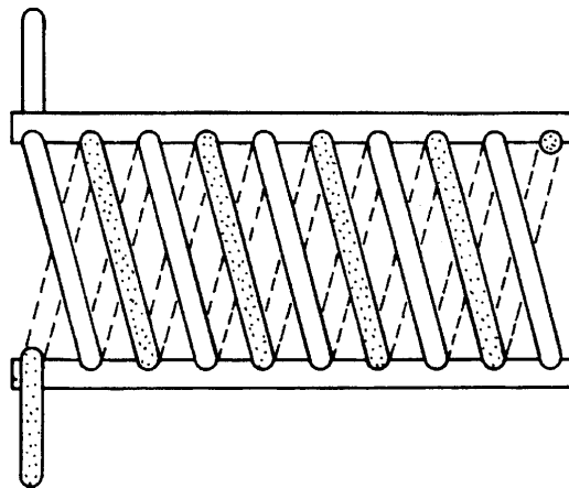
FIGURE 3 (PRIOR ART)
