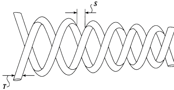
FIGURE 4 (PRIOR ART)
