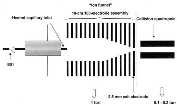
FIGURE 6 (PRIOR ART)
